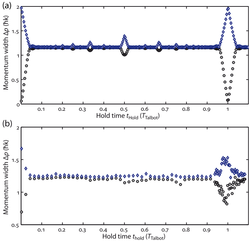
Figure 5. Talbot revival as evidenced by the spread of momentum width \Delta p . (a) Calculated (\Delta p)_{\text{max}} (blue diamonds) and (\Delta p)_{\text{min}} (black circles) as a function of t_{\text{hold}} in units of T_{\text{Talbot}} . (b) Measurement of (\Delta p)_{\text{max}} (blue diamonds) and (\Delta p)_{\text{min}} (black circles) as a function of t_{\text{hold}} in units of T_{\text{Talbot}} for a vertical trap frequency of \omega_z = 2\pi \times 22.0(2) Hz. The extrema are determined from a sample of ten single experimental realizations for each value of t_{\text{hold}} .
