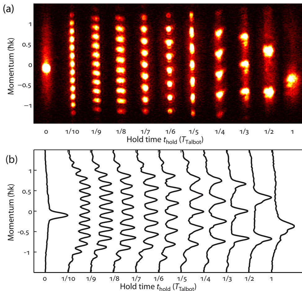
Figure 3. BEC-based temporal Talbot effect—experiment. (a) Series of absorption images after 80 ms of expansion, showing fractional Talbot fringes of different order in momentum space, starting from the initial momentum distribution of the BEC after two BOs (left), followed by the tenth order at T_{\text{Talbot}}/10 , ninth order at T_{\text{Talbot}}/9 , etc, down to the zeroth order at the Talbot time (right). Note that the time axis is not linear. White areas indicate higher density. (b) Horizontally integrated density profiles obtained from the absorption images shown in (a). Note that, for example, for T_{\text{Talbot}}/10 , the outermost momentum component appears twice, i.e. at both edges of the Brillouin zone.
