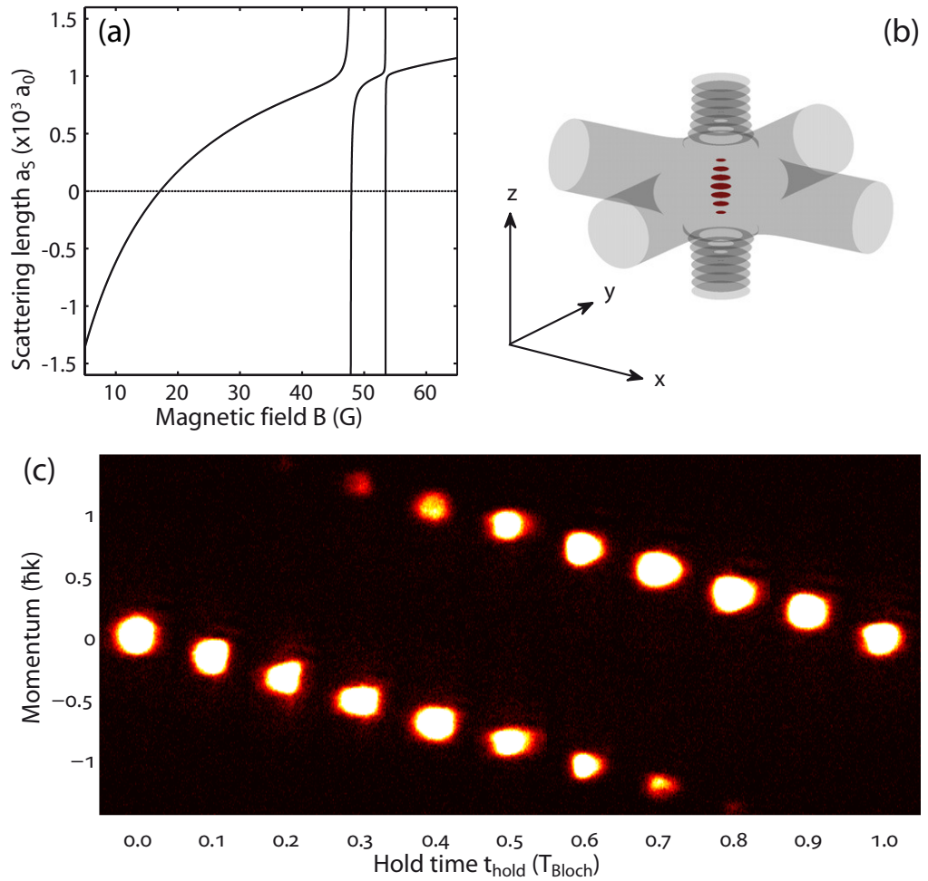
Figure 1. (a) Magnetic field dependence of the scattering length a_s for Cs atoms in F = 3 , m_F = 3 : wide tunability is given by a broad magnetic Feshbach resonance with a pole near -11 G (not shown), leading to a region with attractive interaction, a zero crossing at about 17 G and a repulsive region above [25]. Two narrow Feshbach resonances can be seen in the vicinity of 50 G. (b) Experimental configuration: a vertically oriented standing laser wave creating a stack of pancake-shaped traps is intersected by two horizontal laser beams. (c) BOs: time series in steps of about 57 \mu\text{s} showing the quasi-momentum distribution over the course of one Bloch cycle.
