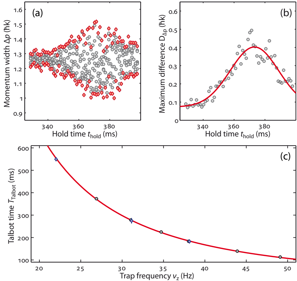
Figure 6. Talbot time T_{\text{Talbot}} as a function of external confinement strength. (a) Momentum width \Delta p in the vicinity of the expected T_{\text{Talbot}} for a dipole trap frequency of \omega_z = 2\pi \times 26.9(2) Hz for ten single experimental realizations (black circles). The extrema (\Delta p)_{\text{max}} and (\Delta p)_{\text{min}} are indicated as red diamonds. (b) Calculated D_{\Delta p} for the measured extrema in (a). The solid line represents a Gaussian fit, from which T_{\text{Talbot}} is derived. (c) Dependence of T_{\text{Talbot}} on trap frequency \nu_z = \omega_z/(2\pi) . The black (blue) circles (diamonds) represent measurements for which the external harmonic trap is generated by the dipole trap beam with a 46 \mu\text{m} ( 144 \mu\text{m} ) beam waist. The solid line gives the calculated values for T_{\text{Talbot}} . The vertical error bars are the 1\sigma uncertainty of the maximum position of the Gaussian fit as shown in (b). The horizontal error bars are equal to or smaller than symbol size.
