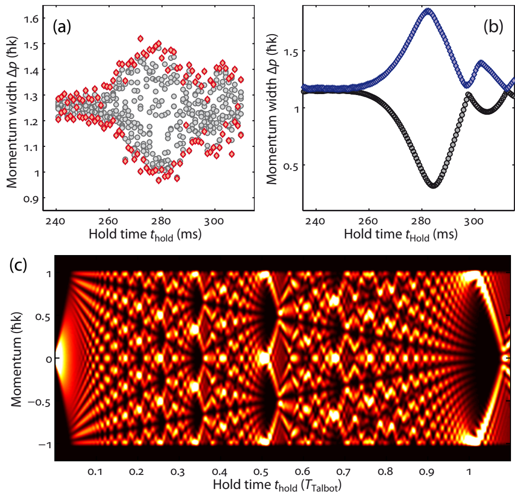
Figure 7. The effect of anharmonic trapping potential on momentum distribution. (a) Momentum width \Delta p in the vicinity of the expected T_{\text{Talbot}} for a dipole trap frequency of 2\pi \times 31.1(2) Hz for ten single experimental realizations (black circles). The vertical dipole trap is created by the more tightly focused dipole trap beam with a beam waist of 46 \mu\text{m} . The extrema (\Delta p)_{\text{max}} and (\Delta p)_{\text{min}} are indicated as red diamonds. (b) Calculated (\Delta p)_{\text{max}} and (\Delta p)_{\text{min}} in the vicinity of the expected T_{\text{Talbot}} for the same experimental parameters as in (a). For the trapping potential, the real Gaussian shape of the dipole trap is used. (c) Full calculation of the momentum distribution as a function of hold time t_{\text{hold}} using the same parameters as in (b).
