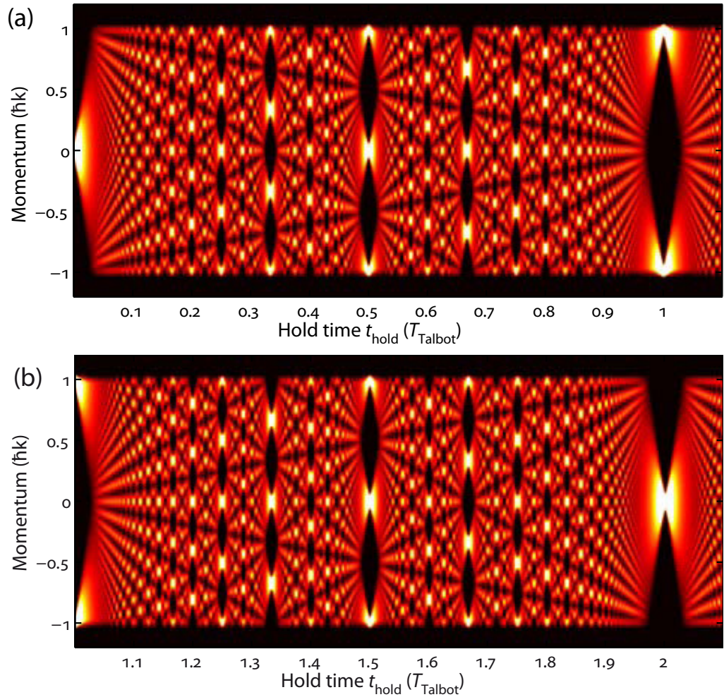
Figure 2. Calculated BEC-based temporal Talbot effect. (a) Momentum distribution as a function of hold time t_{\text{hold}} starting from the initial BEC to the first revival at T_{\text{Talbot}} for a pure harmonic potential. White areas indicate a high occupation of the respective momentum state. (b) Same as in (a) from t_{\text{hold}} = T_{\text{Talbot}} to t_{\text{hold}} = 2T_{\text{Talbot}} .
