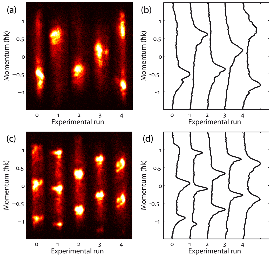
Figure 4. Variations in the momentum distribution between successive experimental realizations for long hold times. (a) Absorption images of five individual experimental realizations with t_{\text{hold}} = T_{\text{Talbot}} . White areas indicate higher density. (b) Horizontally integrated density profiles obtained from the absorption images shown in (a). (c) Absorption images of five individual experimental realizations with t_{\text{hold}} = T_{\text{Talbot}}/2 . (d) Horizontally integrated density profiles obtained from the absorption images shown in (c). Note that, in addition to the random shift in quasi-momentum space caused by \delta , effects of horizontal dynamics, especially fragmentation and density variations along the horizontal axis, can be observed.
