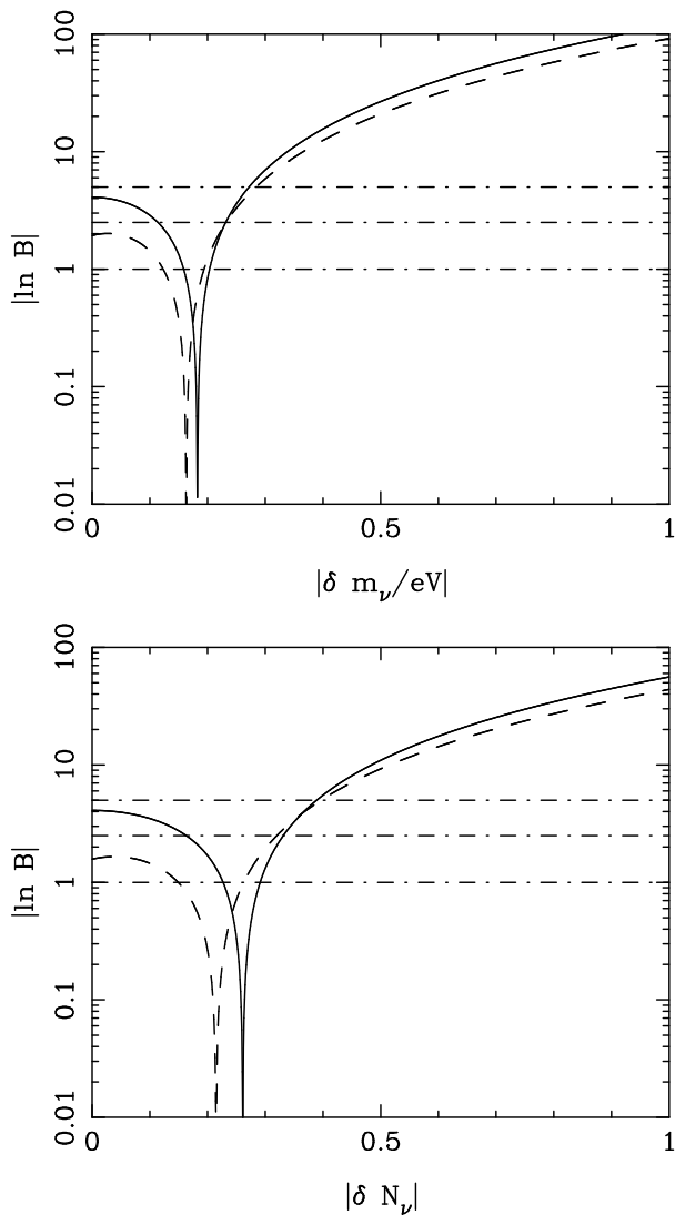
FIG. 2: The predicted evidence for the number N_\nu and total mass m_\nu of neutrinos individually for 3D cosmic shear using the fiducial survey combined with a Planck prior. In each plot the solid line show the conditional evidence assuming that the other parameter is fixed at its fiducial value, the dashed line shows the marginal expected evidence when the possible values of the hidden parameter are taken into account, see Eqn. (12). The dot-dashed lines show the defining evidence limits on the Jeffery’s scale where \ln B < 1 is ‘inconclusive’, 1 < \ln B < 2.5 is ‘substantial’ evidence in favour of a model, 2.5 < \ln B < 5 is ‘strong’, and \ln B > 5 is ‘decisive’.
