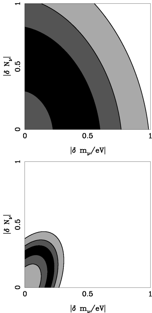
FIG. 1: The expected joint evidence for the number N_\nu and mass m_\nu of neutrinos using 3D cosmic shear and the fiducial survey design. White=‘decisive’, lightest gray=‘substantial’, darkest gray=‘strong’ and black=‘inconclusive’. The upper panel shows the constraints from Planck alone, the lower panel shows the constraints when 3D cosmic shear from the fiducial survey is combined with Planck .
