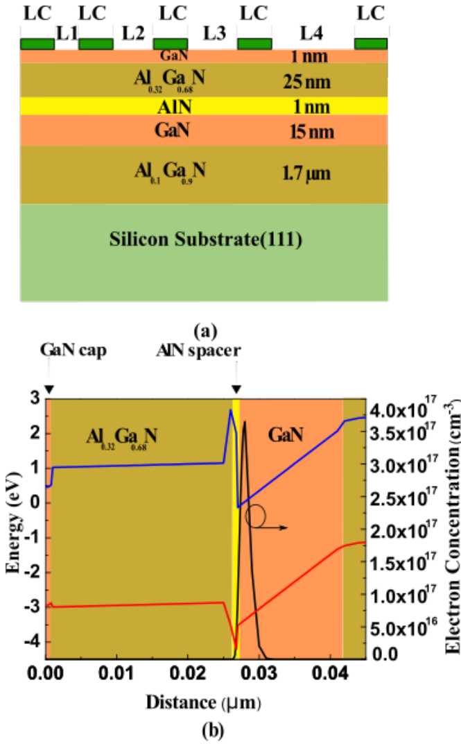
Fig. 1. (a) Schematic cross section of the AlGaIn/GaN TLM structure and (b) energy band diagram and electron concentration profile at equilibrium.
