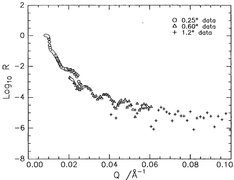
Figure 4.10: Reflectivity data collected from the same sample at three different incident angles. 0.25^\circ data normalised to 1 in region of total reflectivity, other data un-normalised.
