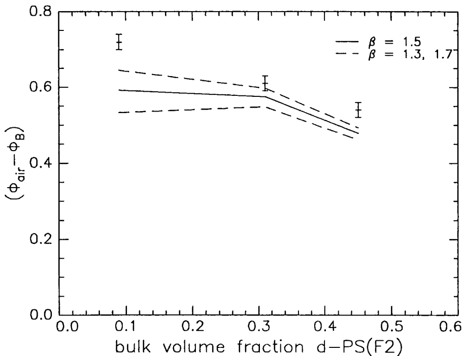
Figure 7.25: Comparison between experimental (\phi_{\text{air}} - \phi_B) and theoretical prediction from SCF theory model. Solid line is from best fit to z^*/R_g for the FL blends equivalent to \beta = 1.5 .
