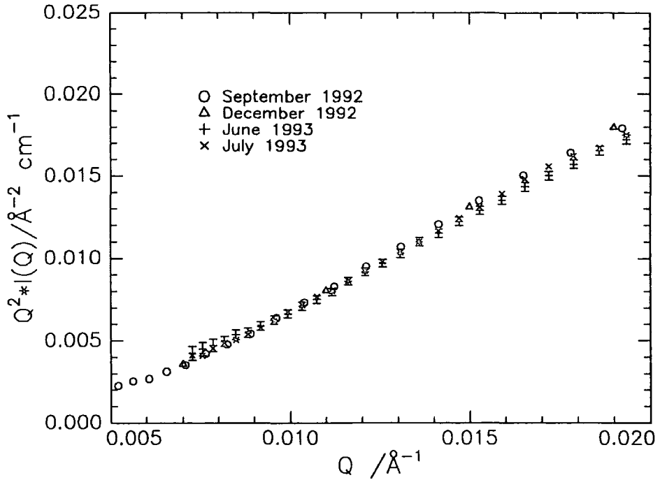
Figure 4.6: Detail of Figure 4.5 (above) showing the low Q region of the Kratky plots.
