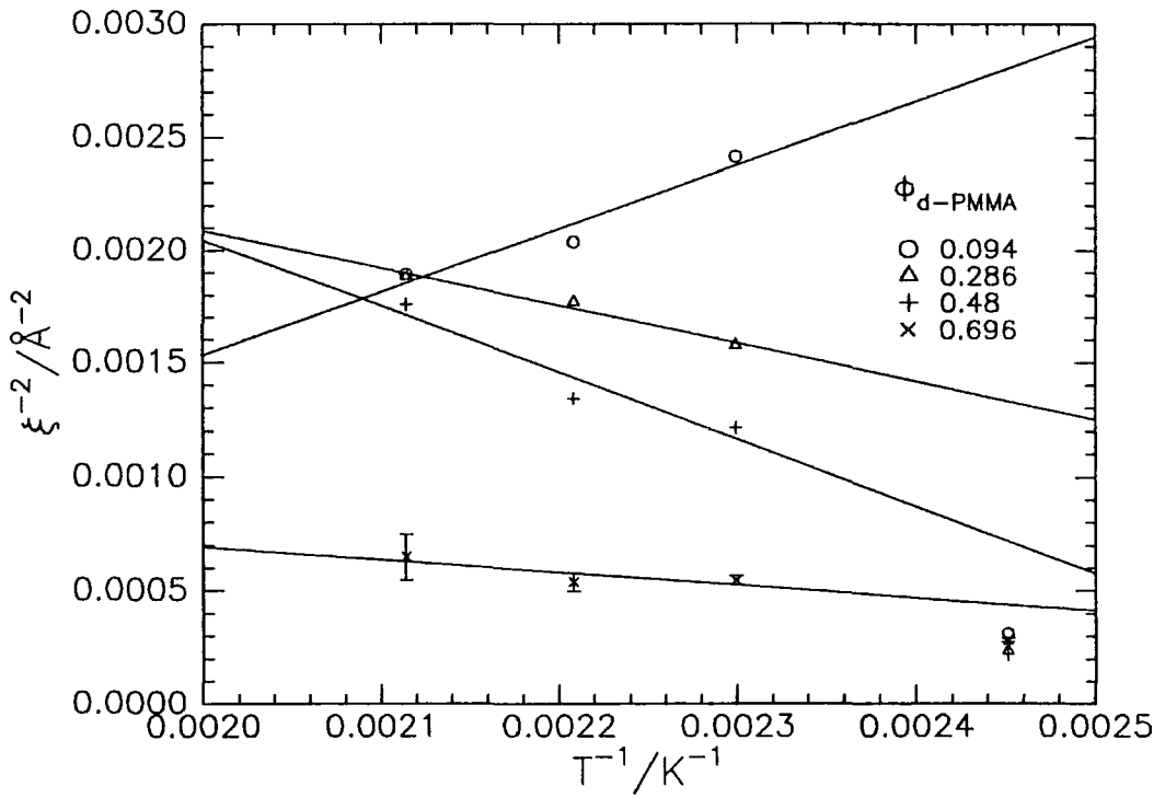
Figure 5.7b: \xi^{-2} vs 1/T for blend B, with straight line fits to 435K-473K data, error bars on \phi = 0.696 from fitting statistics.
