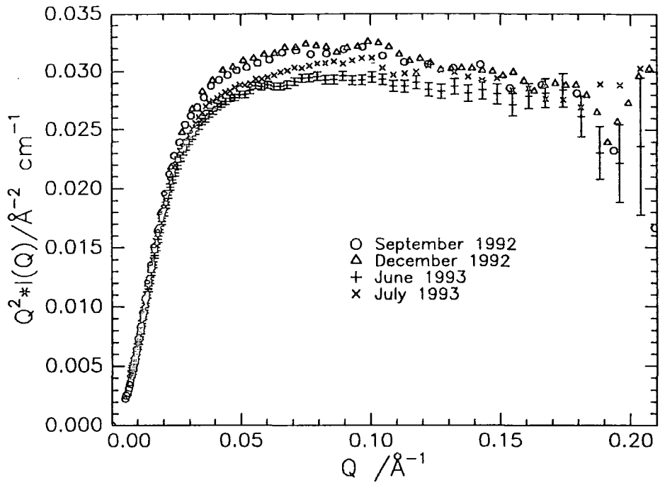
Figure 4.5: Kratky plots of data collected from calibration samples and normalised by calibration constant.
