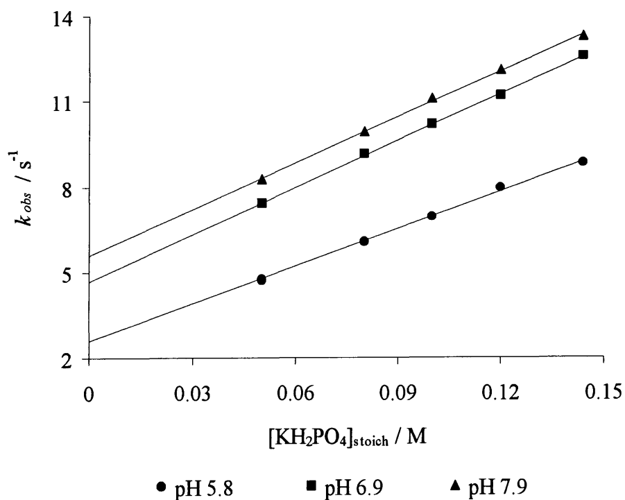
Figure 2.4: k_{obs} / s^{-1} against [KH 2 PO 4 ] stoich / M at pH 5.8, 6.9 and 7.9 at 25 °C in aqueous solution with [HCHO (aq) ] = 0.053 M, I = 1 M
