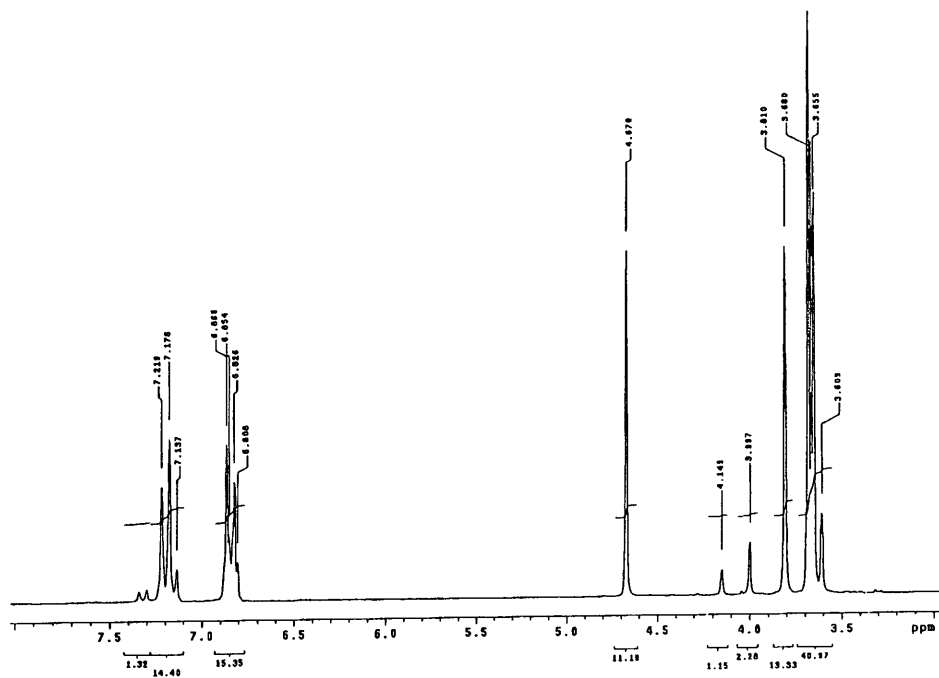
Figure 6.10: 0.19 M 4-methoxybenzylamine and 0.20 M CH 2 (OH)(SO 3 Na): 36 minutes after mixing
