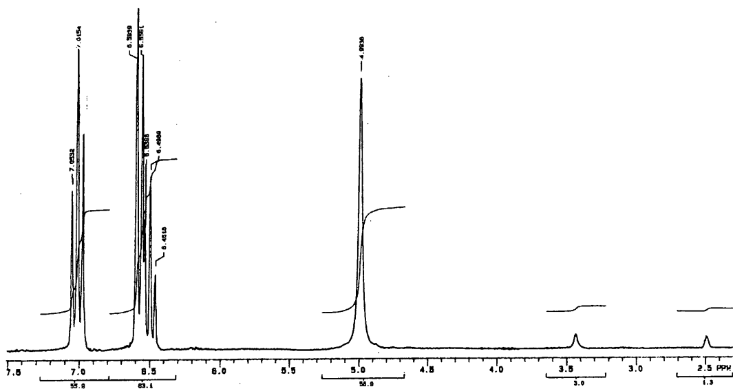
Figure 3.1: ^1\text{H} NMR spectrum of aniline in \text{d}_6 -DMSO
