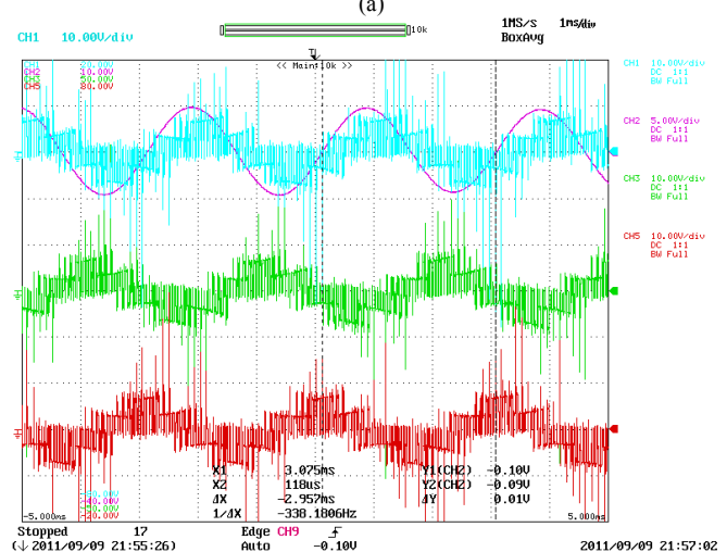
Fig. 21. The measured phase voltage and current waveforms under flux-weakening conditions, (a) with 60degrees current phase advanced angle, (b) with 85degrees current phase advanced angle. (CH1 - Phase A voltage, CH3 - Phase B voltage, CH5 - Phase C voltage, CH2 - Phase A current.)
