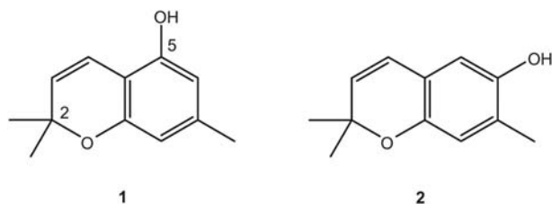
Figure 1 Structures of 2,2,7-trimethyl-2H-chromen-5-ol ( 1 ) and acremine C ( 2 ).
