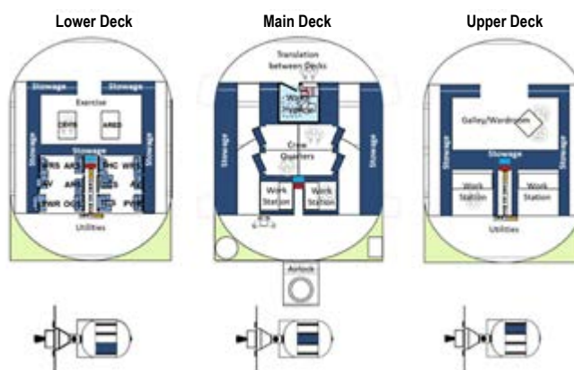
Skylab Gen 2 internal layout.
