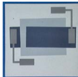
First ultracapacitor single cell built at MSFC (electrodes are dark blue and active material is pale blue). This device weighs <10 gm but has an equal capacitance and voltage of a bank of capacitors weighing over 490 gm.
