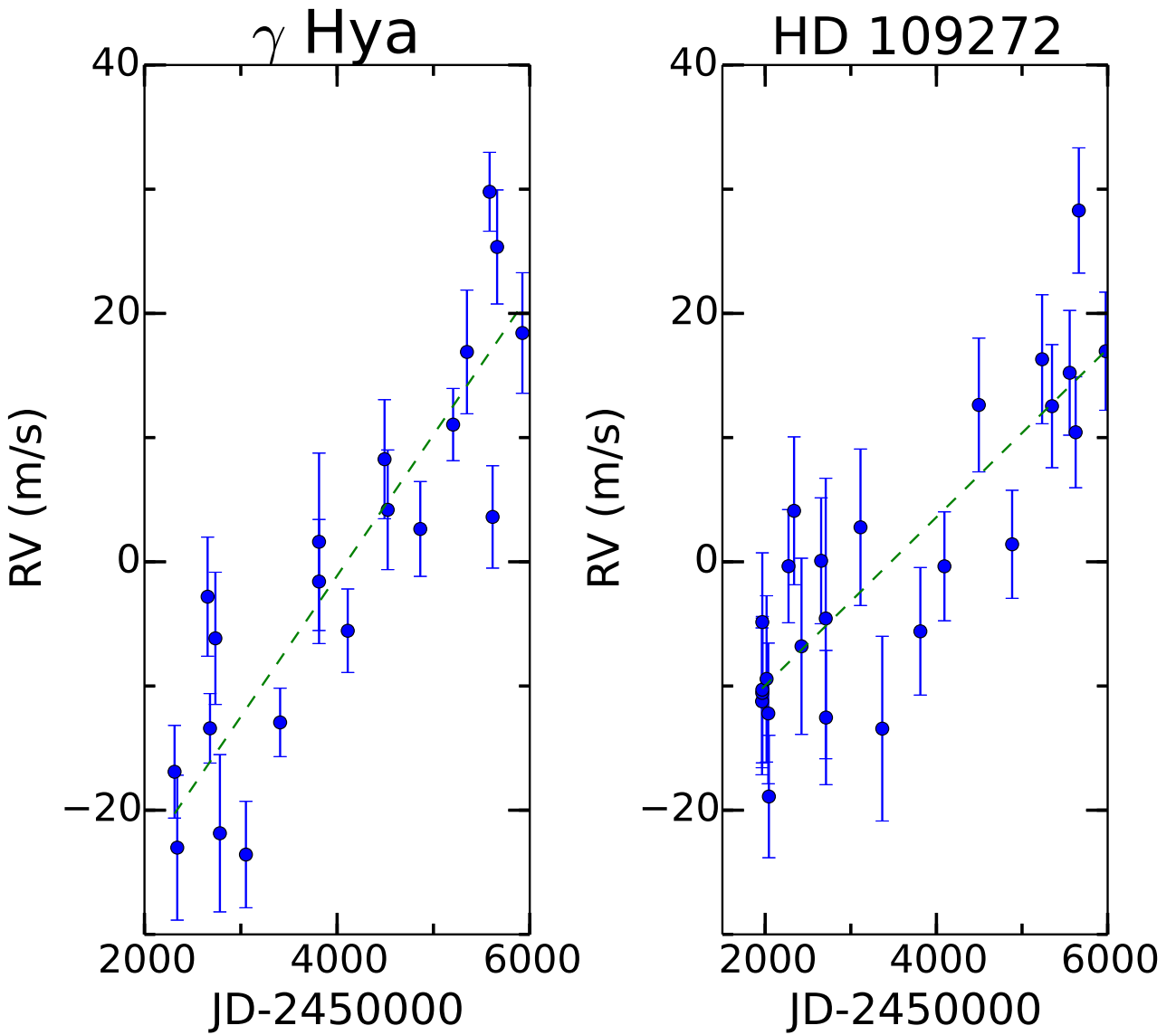
Fig. 2.— Measured RV data of the two systems \gamma Hya (left) and HD 109272 (right). The dashed lines show the best-fit linear trends.
