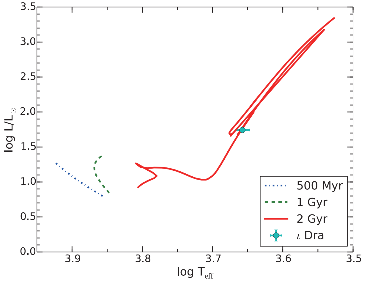
Fig. 7.— PARSEC (Bressan et al. 2012) isochrone plot, effective temperature T_{\text{eff}} vs. luminosity. The green dot with error bars is the measured value for \iota Dra, which clearly agrees with the 2-Gyr PARSEC isochrone model.
