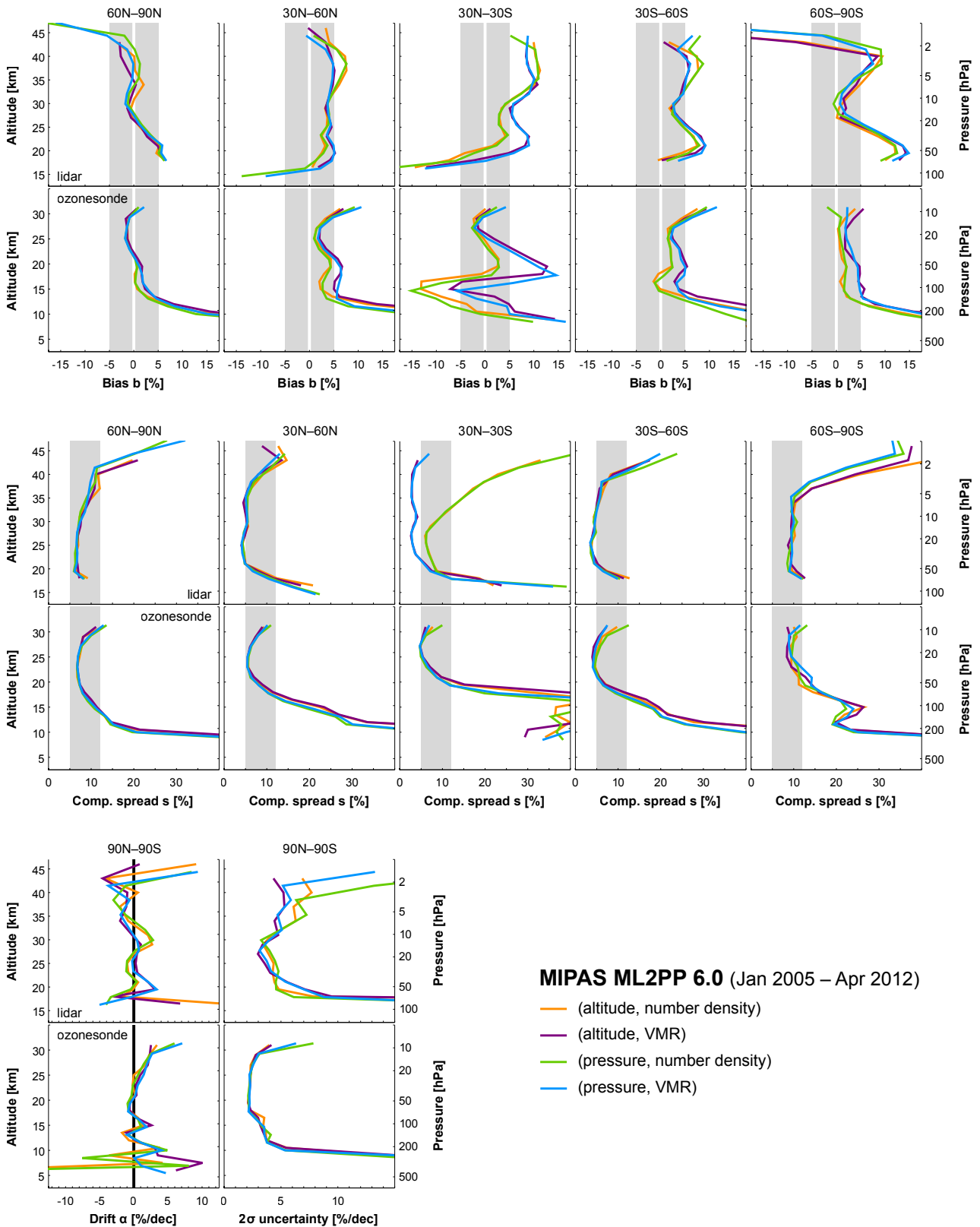
Figure S13. Same as Fig. S3, but for MIPAS ML2PP6.0 2005–2012 nominal observation data (nominal representation: ozone VMR on variable pressure levels). The large increase in the spread of tropical lidar comparisons is due to outliers in the averaging kernels. It is not seen when a triangular smoothing function is used.
