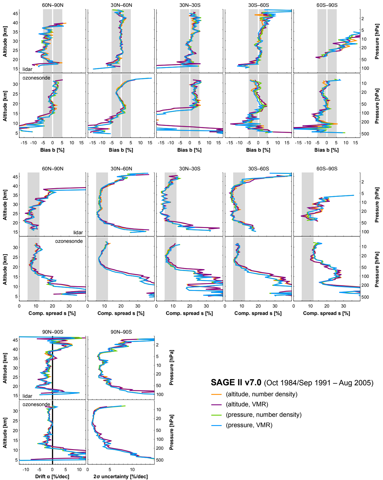
Figure S3. SAGE II v7.0 ozone data quality in different profile representations (see legend): bias (top part), comparison spread (middle) and drift (bottom) from comparisons to NDACC/GAW/SHADOZ ozonesonde and NDACC stratospheric lidar instruments. Only latitude bands with at least 10 comparison pairs are shown. The nominal representation of SAGE II is ozone number density on fixed altitude levels. Satellite and ozonesonde profiles are converted using auxiliary information included in the ozone data files, lidar profiles are converted using ERA-Interim fields. More information in Sect. 6. The SAGE II versus lidar results shown here cover 1991–2005, since we had no ERA-Interim data at our disposal to cover the earlier years. The SAGE II versus ozonesonde results cover 1984–2005.
