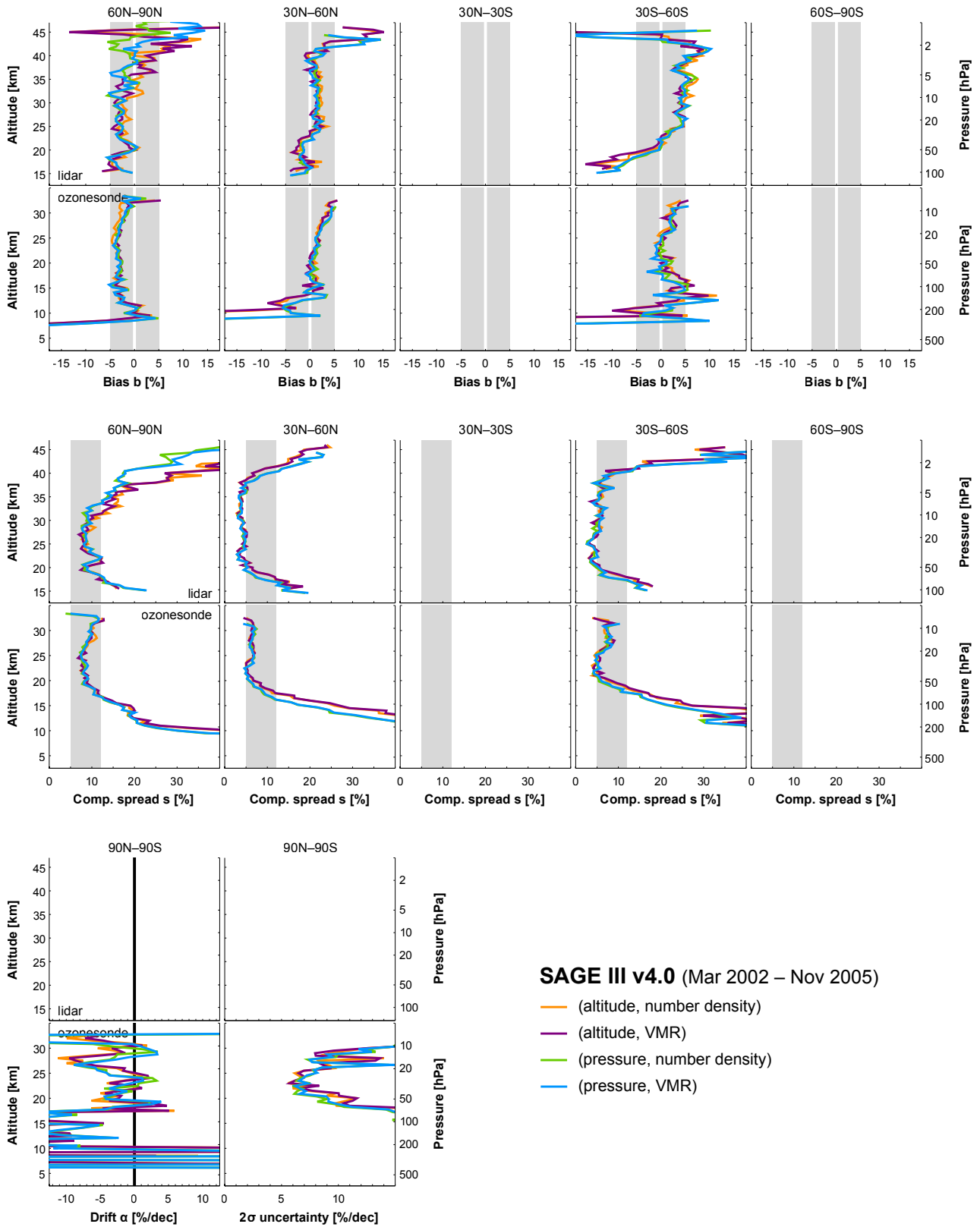
Figure S4. Same as Fig. S3, but for SAGE III v4.0 (nominal representation: ozone number density on fixed altitude levels).
