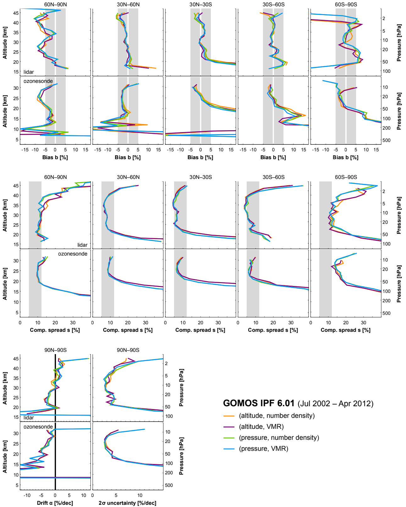
Figure S12. Same as Fig. S3, but for GOMOS IPF6.01 (nominal representation: ozone number density on variable altitude levels).
