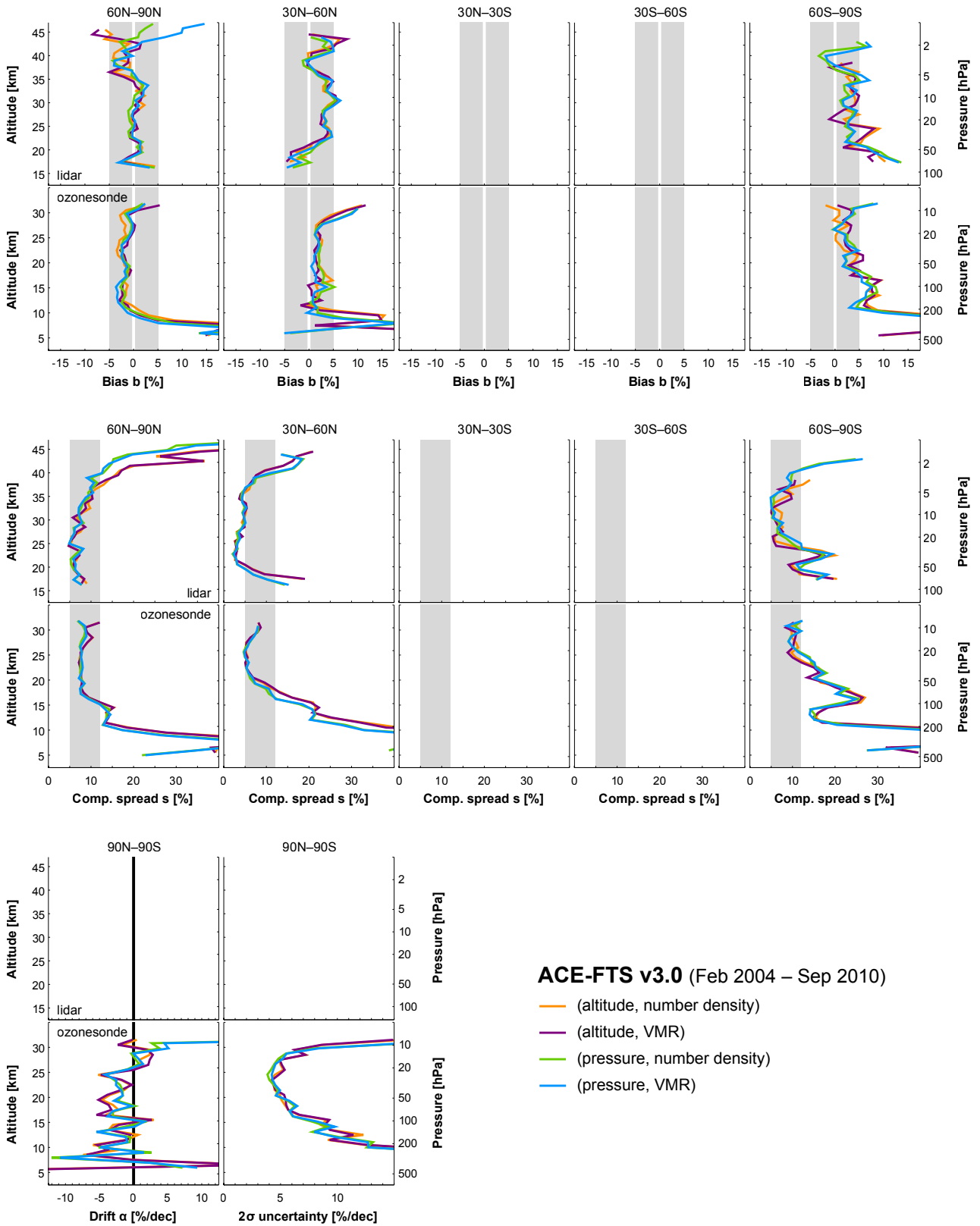
Figure S15. Same as Fig. S3, but for ACE-FTS v3.0 (nominal representation: ozone VMR on fixed altitude levels).
