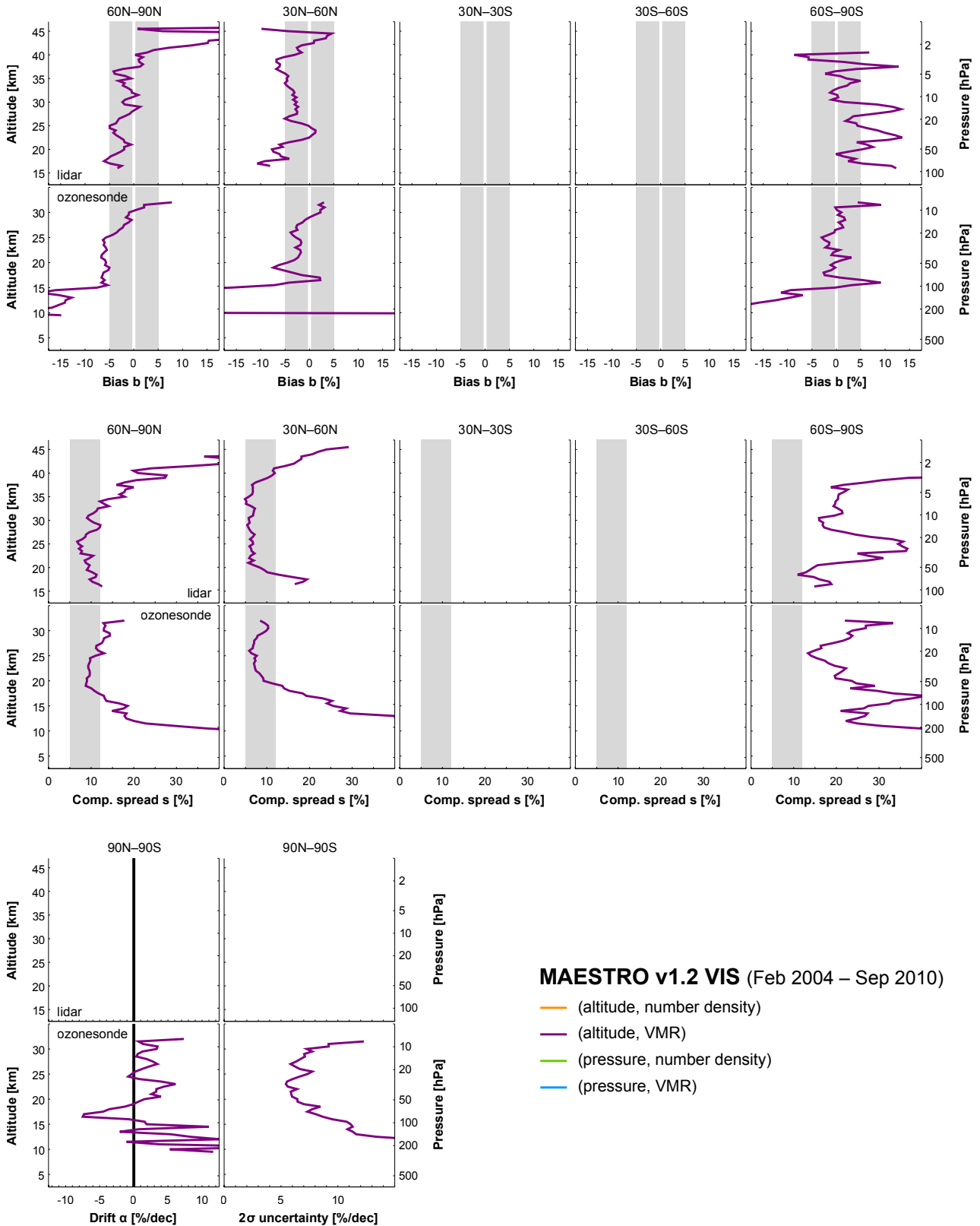
Figure S16. Same as Fig. S3, but for the nominal representation of MAESTRO v1.2 (ozone VMR on variable altitude levels). Non-native representations were not verified here since the required auxiliary data are identical to those of ACE-FTS v3.0. So we expect a similar representation-dependence as in Fig. S15.
