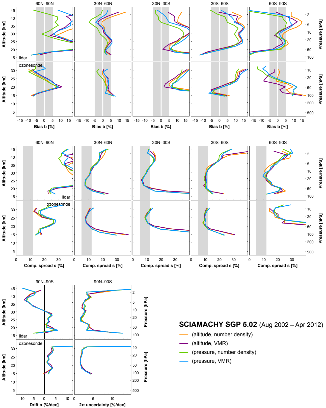
Figure S14. Same as Fig. S3, but for SCIAMACHY SGP5.02 (nominal representation: ozone number density on fixed altitude levels).
