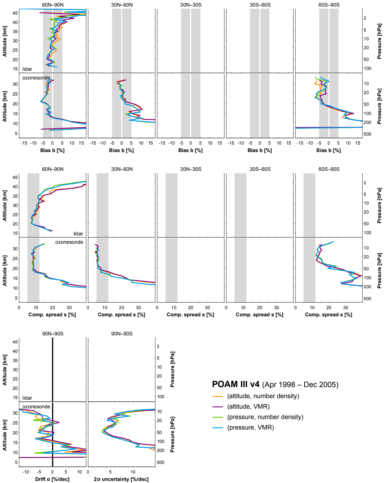
Figure S9. Same as Fig. S3, but for POAM III v4 (nominal representation: ozone number density on fixed altitude levels).
