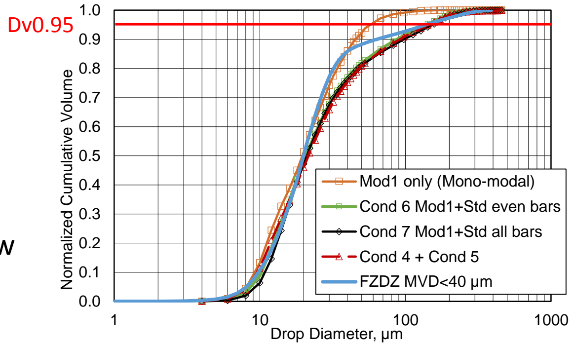
Drop-Size Distributions resembling FZDZ, MVD<40 μm
