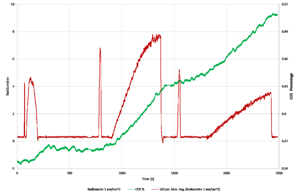
Saffire-2 Samples 7, 8, and 9
