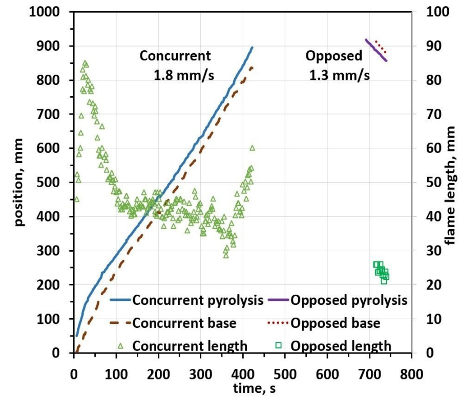
Left: Flame base and pyrolysis position for concurrent and opposed-flow test in Saffire-1. Air flow speed was 20 cm/s.
