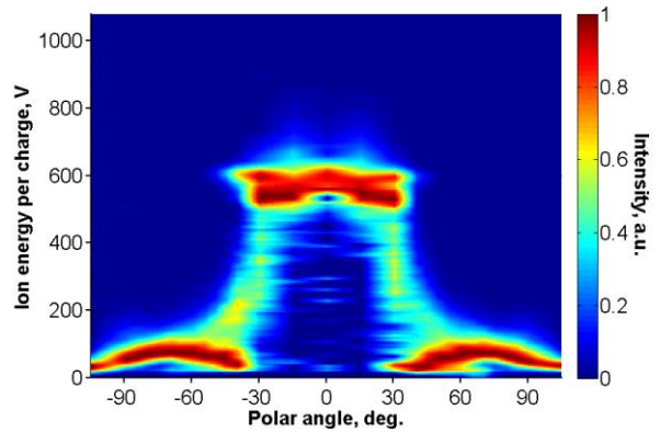
Figure 29. Plot of ion energy per charge distribution versus polar angles for the alumina covers with floating configuration at the 600-12.5 RFC.
