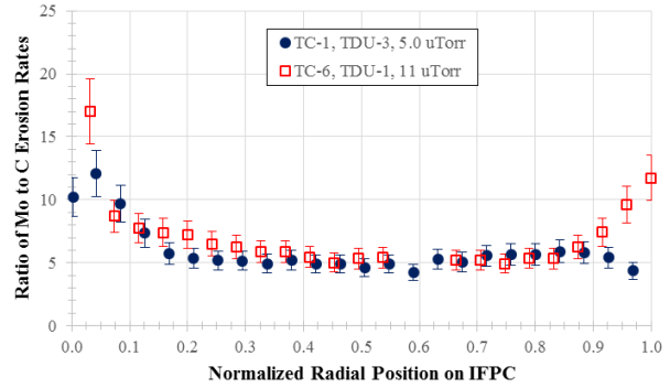
Figure 28. Ratios of Mo to C IFPC erosion rates as a function of facility pressure and TDU configuration for V_a=300 V.
