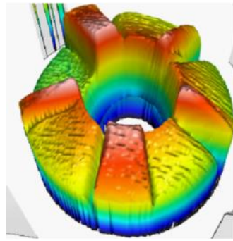
Figure 12. Erosion of the TDU-3 keeper during each of the short duration wear tests in VF-5.
