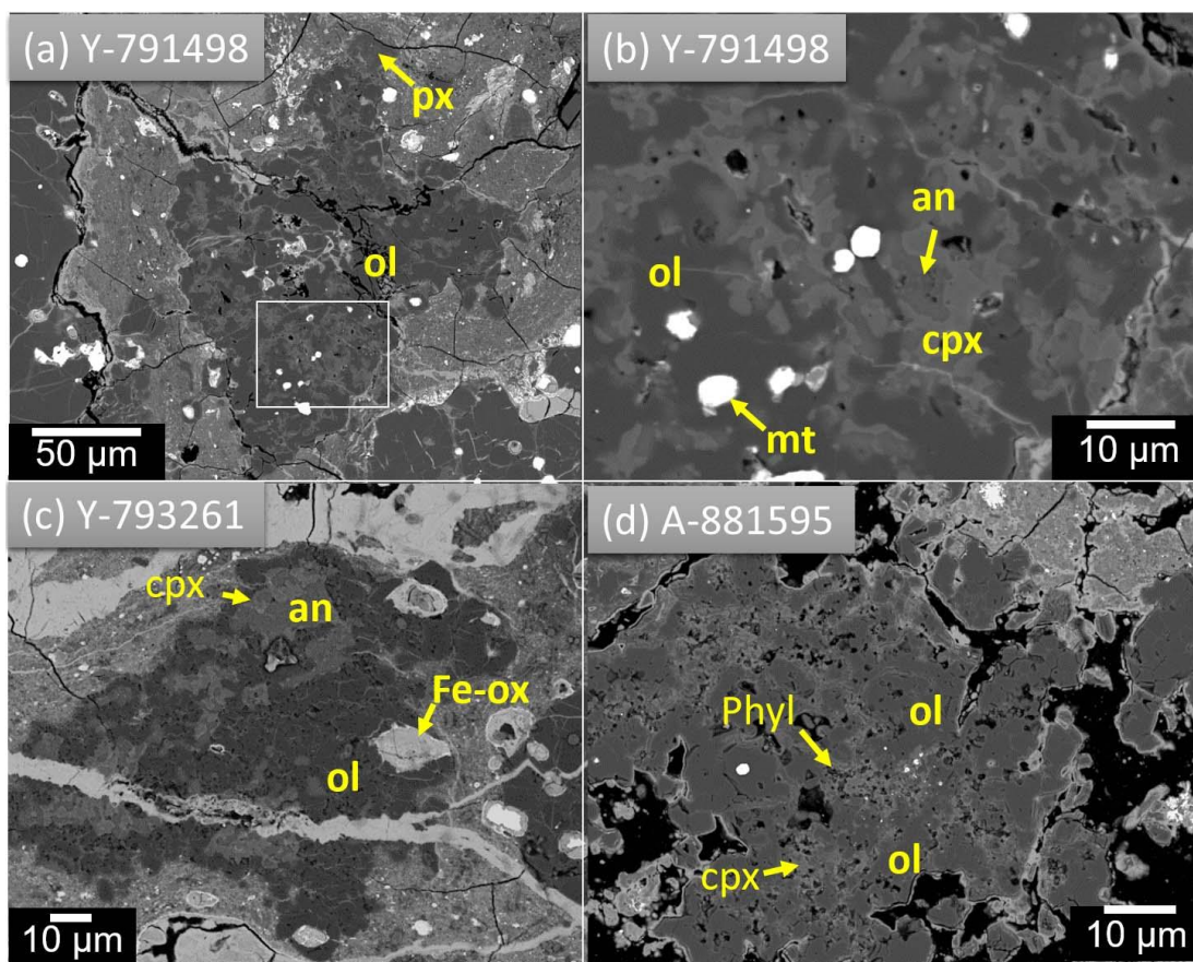
Fig.1. BSE image of AOAs. (a, b) AOA from the sample with little alteration. (c) AOA from the sample with intermediate alteration. (d) AOA from severely altered sample.
