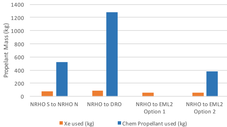
Figure 21. Comparison of SEP vs. Chemical propulsion for cislunar transfers
