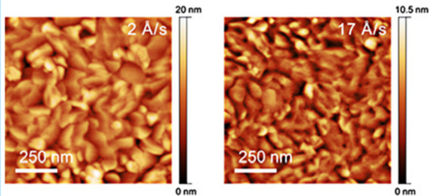
Fig. 10. AFM images at a length scale of 1 \mu\text{m} \times 1 \mu\text{m} of UHV electron beam evaporated Al films (60 nm thickness) at deposition rates of 2 Å/s (left) and 17 Å/s (right).
