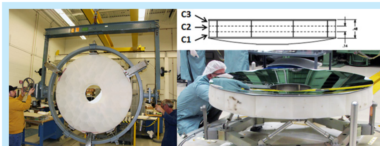
Fig. 1: Left: LTF mirror substrate. Top Right: 5-layer design. Bottom Right: Completed mirror assembly.
