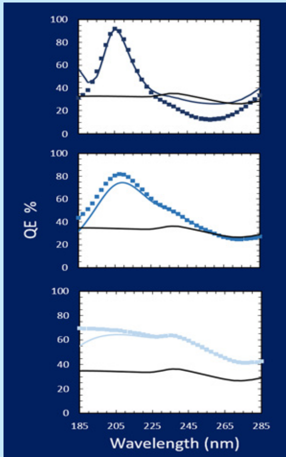
Fig. 5. Left: QE performance in the UV with (top to bottom) five-layer, three-layer, and single-layer dielectric designs. Right: CCD201s processed by superlattice doping and ALD coating for the same three designs. The middle option was selected for flight.
