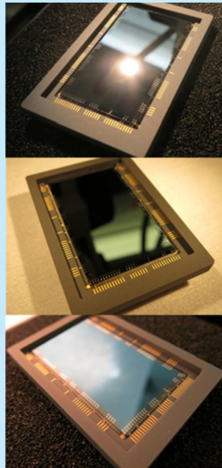
Fig. 5. Left: QE performance in the UV with (top to bottom) five-layer, three-layer, and single-layer dielectric designs. Right: CCD201s processed by superlattice doping and ALD coating for the same three designs. The middle option was selected for flight.
