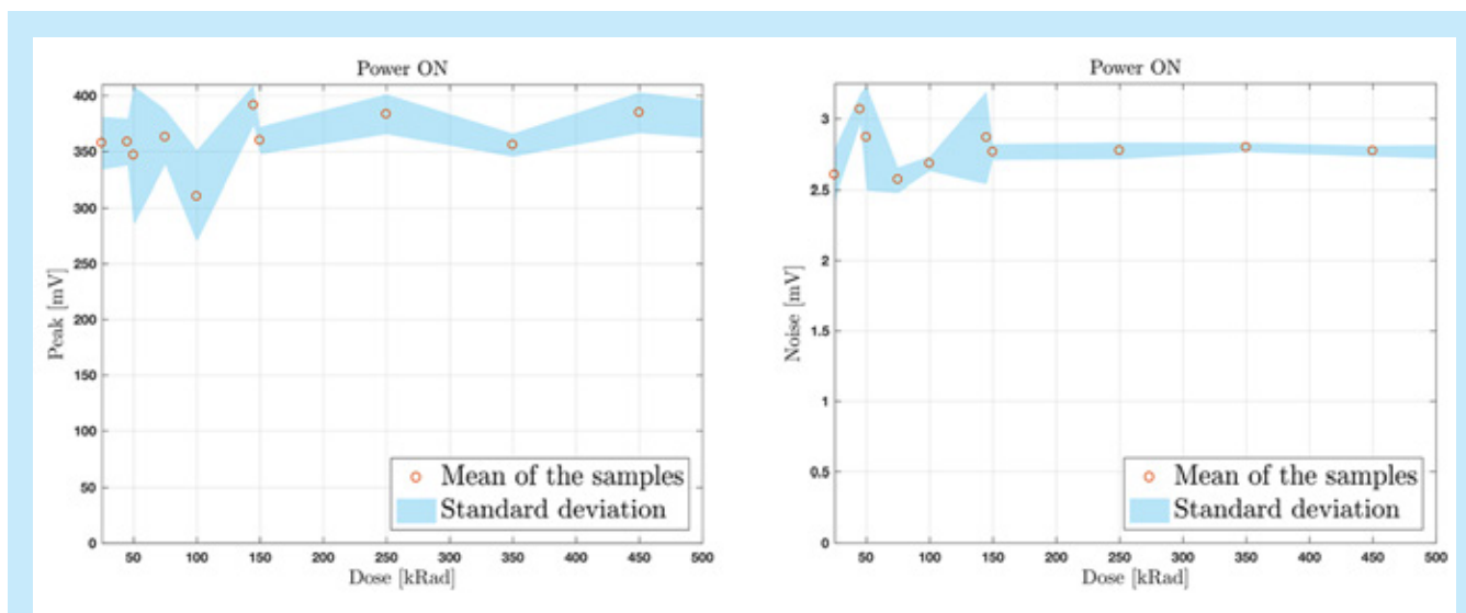
Fig. 20. Gain (left) and rms noise (right) of the CSAv3 CSA ASICs vs. TID from ^{60}\text{Co} gamma rays. Six chips with 16 channels each were tested and the standard deviation was derived from the variation of the channels. Not all chips received the full dose.
