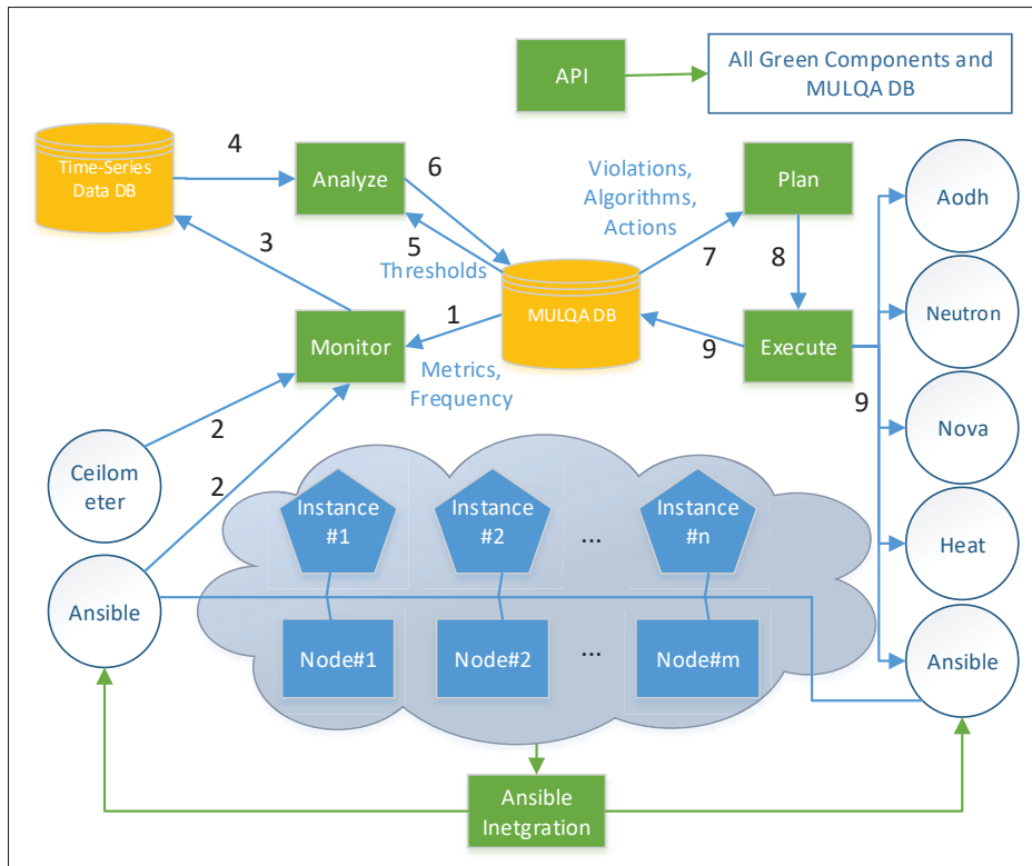
Figure 4.3 MULQA implementation modules and the control loop workflow
