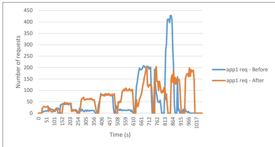
Figure 4.20 Chart for number of received requests by app1 over time before and after MULQA control
