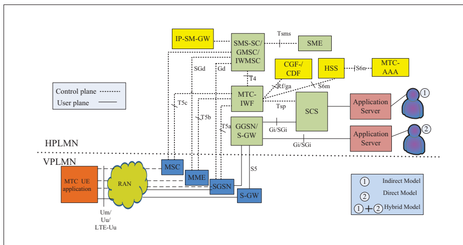
Figure 1.7 3GPP LTE/LTE-A architecture reference model for M2M communications
