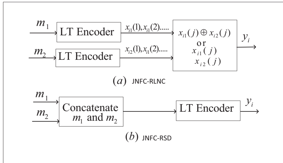
Figure 4.5 Encoding schemes at relay nodes
