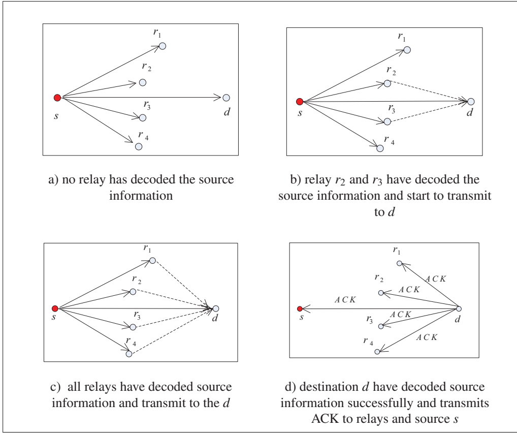
Figure 2.6 Steps of the source-feedback based protocol
