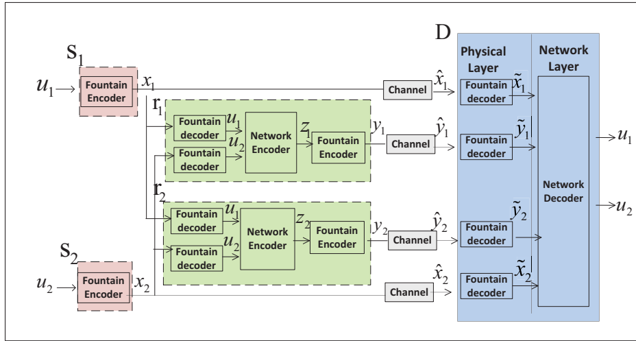
Figure 3.3 Block diagram of separated network and fountain coding
