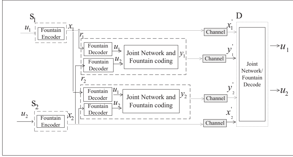
Figure 3.5 Block diagram of joint network and fountain coding system
