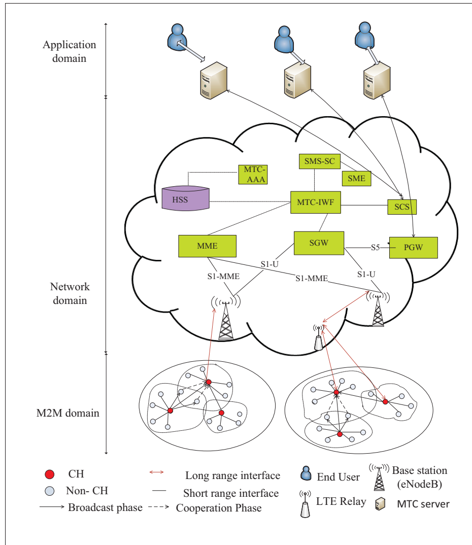
Figure 2.3 An LTE-A connected heterogeneous M2M networking architecture
