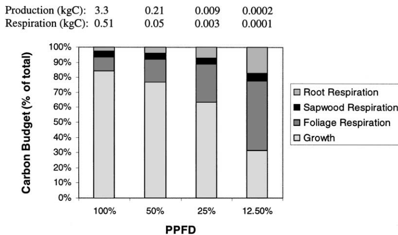
Fig. 6. Yearly carbon budget for a 10-year-old model Jack pine for four light levels. The amounts are expressed as percentages of the total photosynthetic carbon production of the tree. Absolute annual amounts of carbon (in kg) for total respiration and photosynthetic production are listed above the graph.
