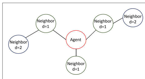
Figure 4.6 — The neighborhood
