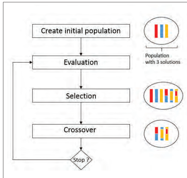
Figure 2.6 — Genetic Algorithm
