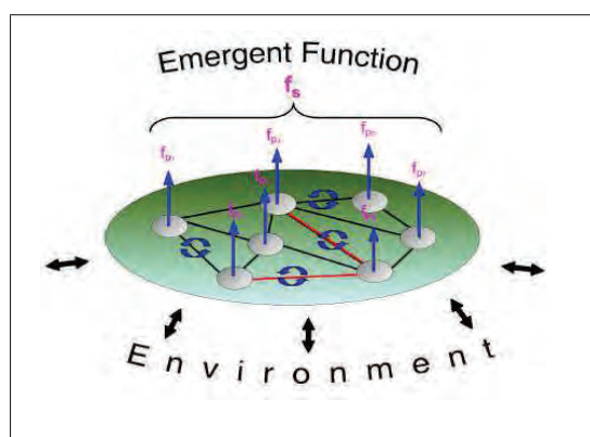
Figure 3.6 — Emergent function
