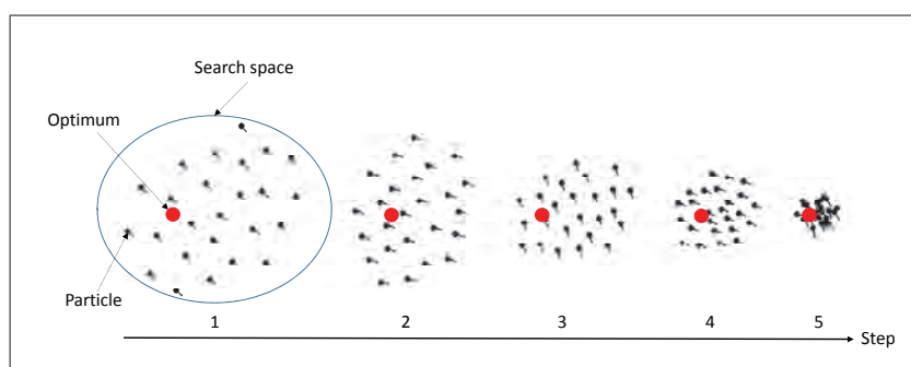
Figure 2.7 — PSO example
