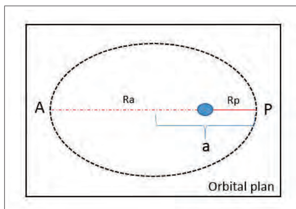
Figure 1.8 — Ellipse parameters
