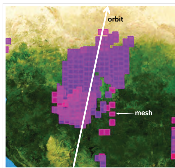
Figure 5.1 — An hot-spot
