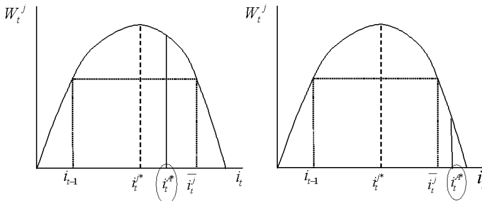
Figure 2: a) Policy problem when: i^{A*} < \bar{i}^j . b) Policy problem when: i^{A*} > \bar{i}^j .
