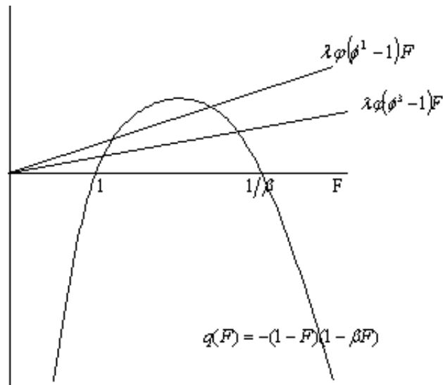
Figure 1: Determinacy condition
