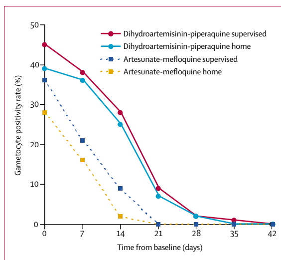
Figure 2: Proportions of patients with patent gametocytaemia
