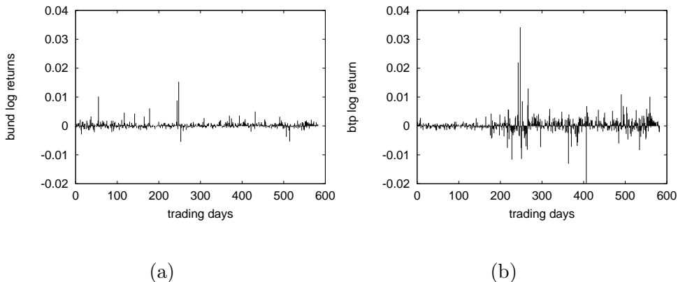
Fig. 2. Logarithmic returns for the BUND (a) and BTP (b) futures
