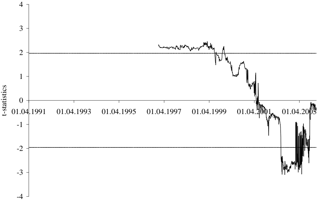
Figure 7: Rolling GARCH(1,1) t-Statistics for \beta_1 (Window = 1500 Observations)
