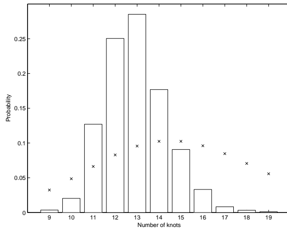
Figure 6: Firm size data: The bars indicate the posterior probability mass function of the number of knots, while the crosses indicate the corresponding prior probabilities.
