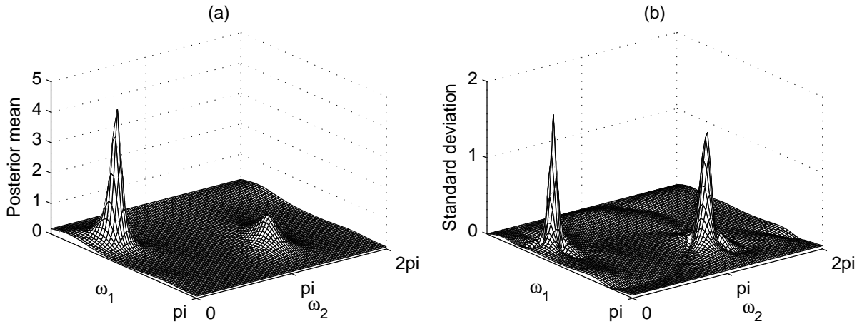
Figure 5: Firm size data: Posterior mean (panel (a)) and posterior standard deviation (panel (b)) of directional dispersion D as a function of direction d_{y-\mu_y} parameterised as in Theorem 1.
