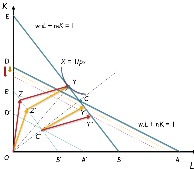
Figure 3. Small KL Gap versus Large KL Gap
