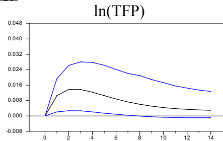
Figure 10: Impulse Responses to technology Shocks: The Solow Period
