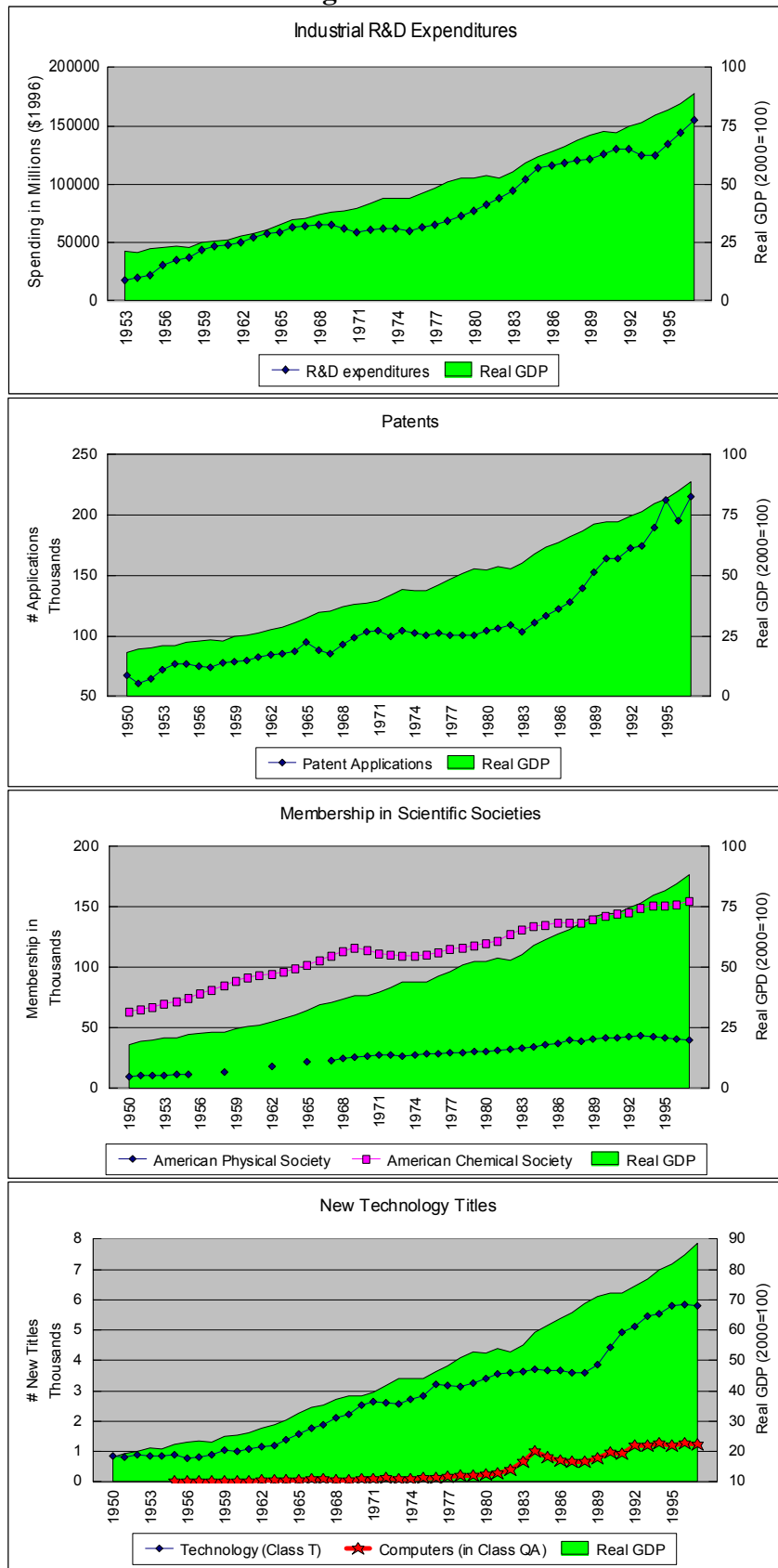
Figure 3. Comparison of Technical Change Measures: 1949-1997
