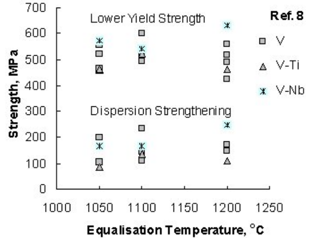
Fig. 11 Effect of equalisation temperature on the strength.
