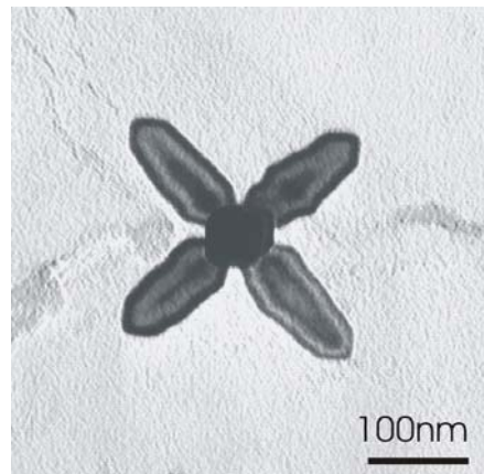
Fig. 4 Cruciform Particle in Steel V-Ti-N Steel after equalisation at 1100°C.
