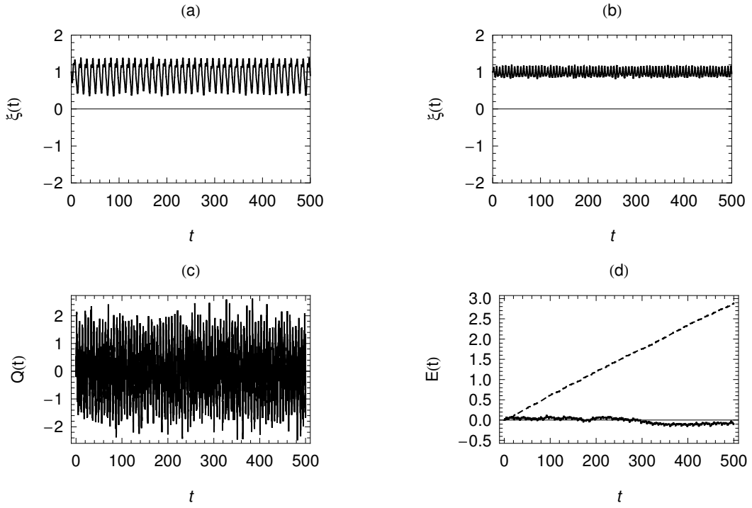
Fig. 5. Un-tuned system far from stochastic resonance with \omega = 0.5 a: Response with forcing ( \eta = 0.7 ) b: Response without forcing ( \eta = 0. ) c: External noise Q(t) and \langle\rho(t)\rangle = 0 d: Energy available from the mechanism with forcing (solid line) and without forcing (dashed line) with damping \bar{c} = 0.5 .
