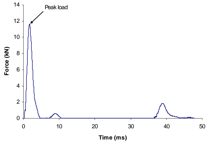
Fig. 6 A representative impact response of an isotropic material [aluminium].
