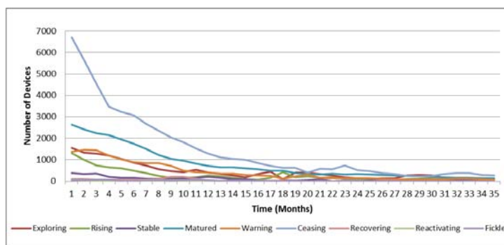
Figure 8. 16 – Distribution of Devices over the Usage Patterns ('Mushroom Garden')
