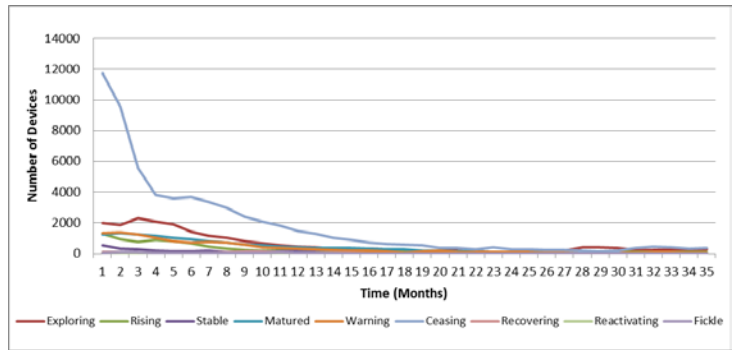
Figure 8. 15 – Distribution of Devices over the Usage Patterns ('Temple Run')
