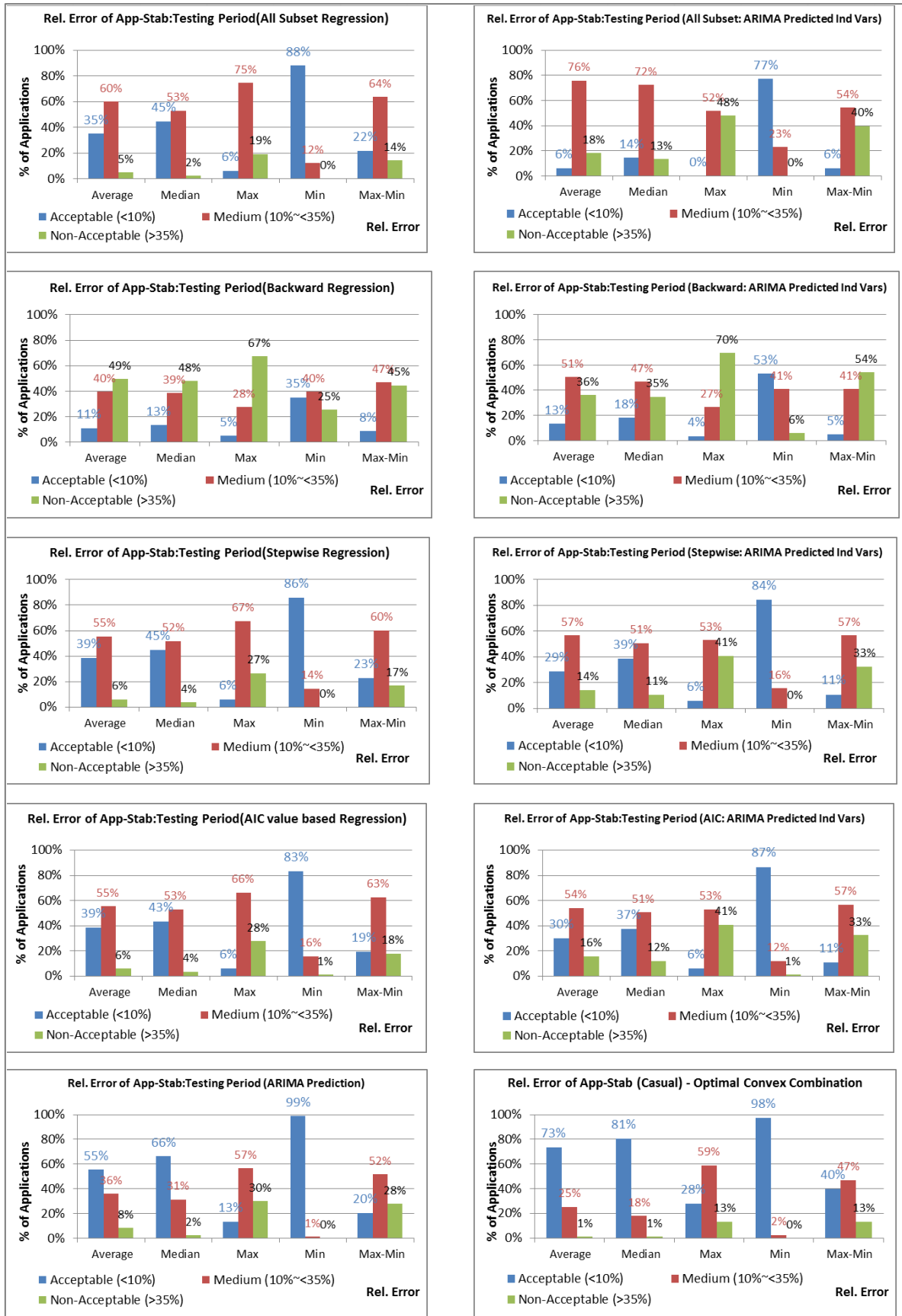
Figure 7. 10 - Estimation Results of App-Stab (Sub-category: Casual)
