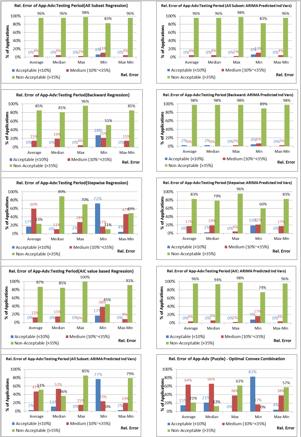
Figure 7. 15 - Estimation Results of App-Adv (Sub-category: Puzzle)
