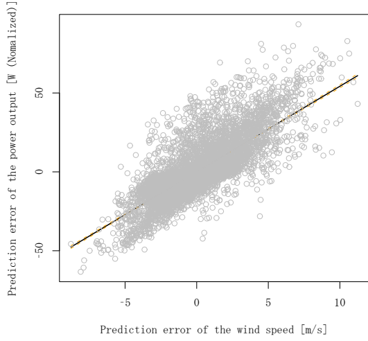
Figure 5.8: Wind speed prediction error ( \epsilon_{w,n} ) vs. Power output prediction error ( \epsilon_{p,n} )
