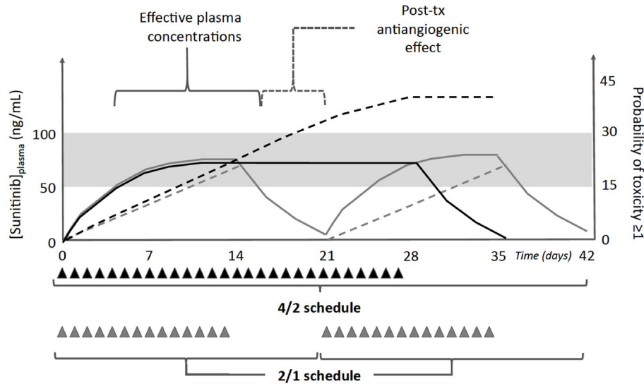
FIGURE 1 | Schematic representation of plasma concentrations (solid lines) and probability of toxicities grade \geq 1 (dashed lines) associated with administration of sunitinib 50 mg/day (triangles) according to the standard 4/2 (black lines/triangles), or the alternative 2/1 schedule (gray lines/triangles). Both regimens have the same dose intensity, but the increased severity of toxicities is associated with the standard schedule. Furthermore, there is the evidence that sunitinib effects may extend up to 1 week after the last daily dose (post-tx antiangiogenic effects), hence the 1 week of rest in the 2/1 schedule could be beneficial for patients while ensuring the recovery from mild toxicities. The gray area represents the therapeutic range of sunitinib plasma concentrations (50–100 ng/mL).
