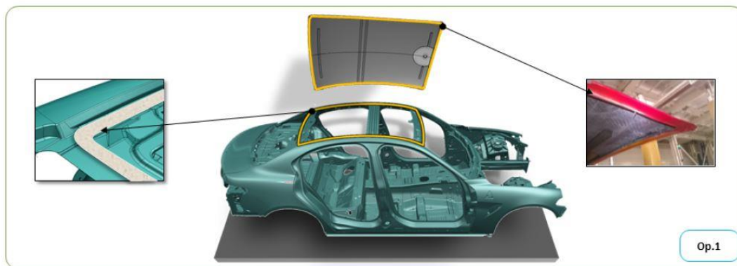
Figure 7.4. First step of pre-assembly of roof panel [1]
