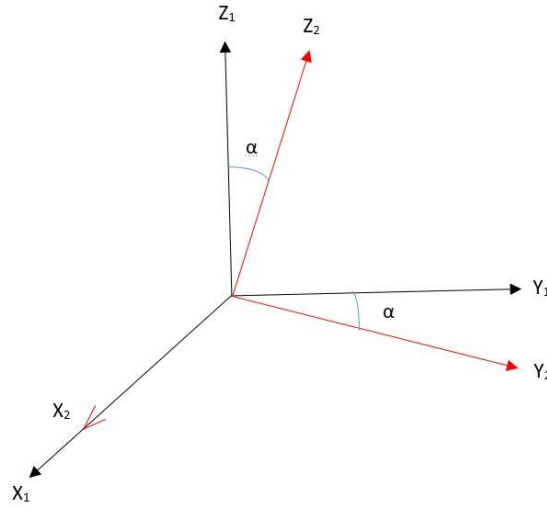
Figure 6.35: Reference coordinate system rotating about the Z-Y plane
