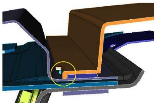
Figure 7.3. Roof feet [1]
