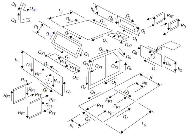
Figure 4.23: Edge forces in the standard sedan in the torsion load case [1]
