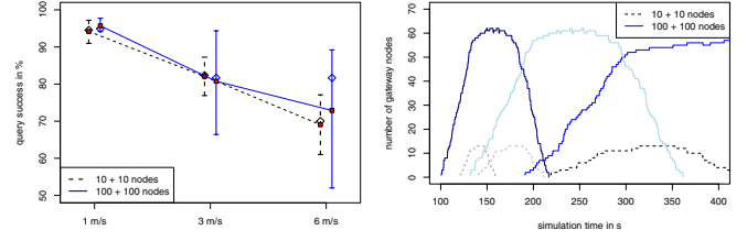
Fig. 7. Success ratio of queries and available gateways over time
