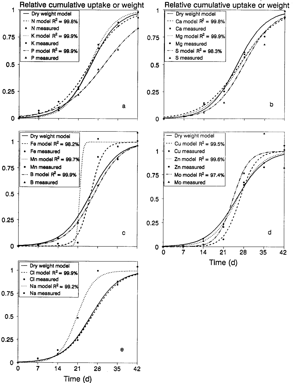
Fig. 2. Relative cumulative uptake of N, P, K, (a), Ca, Mg, S (b), Fe, Mn, B (c), Cu, Zn, Mo (d), and Cl, Na (e) by one lettuce head, and relative dry weight as a function of time. Measured data are described with the logistic model (Eq. 3).
