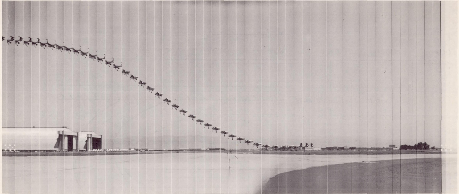
Figure 9.- Typical STOL take-off from a standing start; Ryan VZ-3RY deflected-slipstream test vehicle; wind calm; flap deflection 40^{\circ} .
