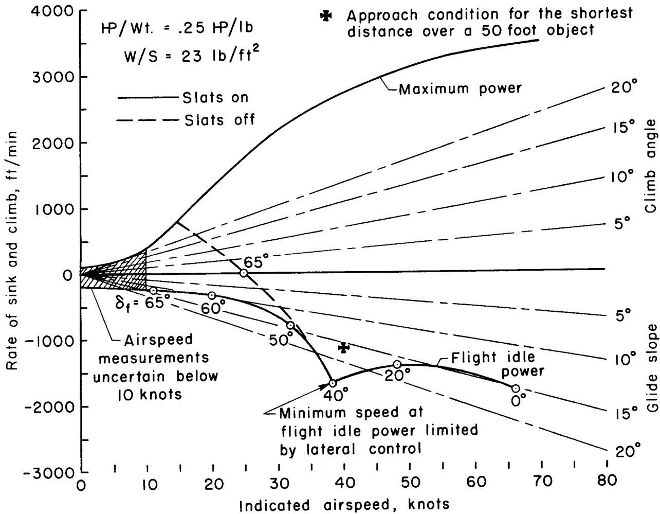
Figure 7.- Flight performance characteristics of deflected-slipstream test vehicle.
