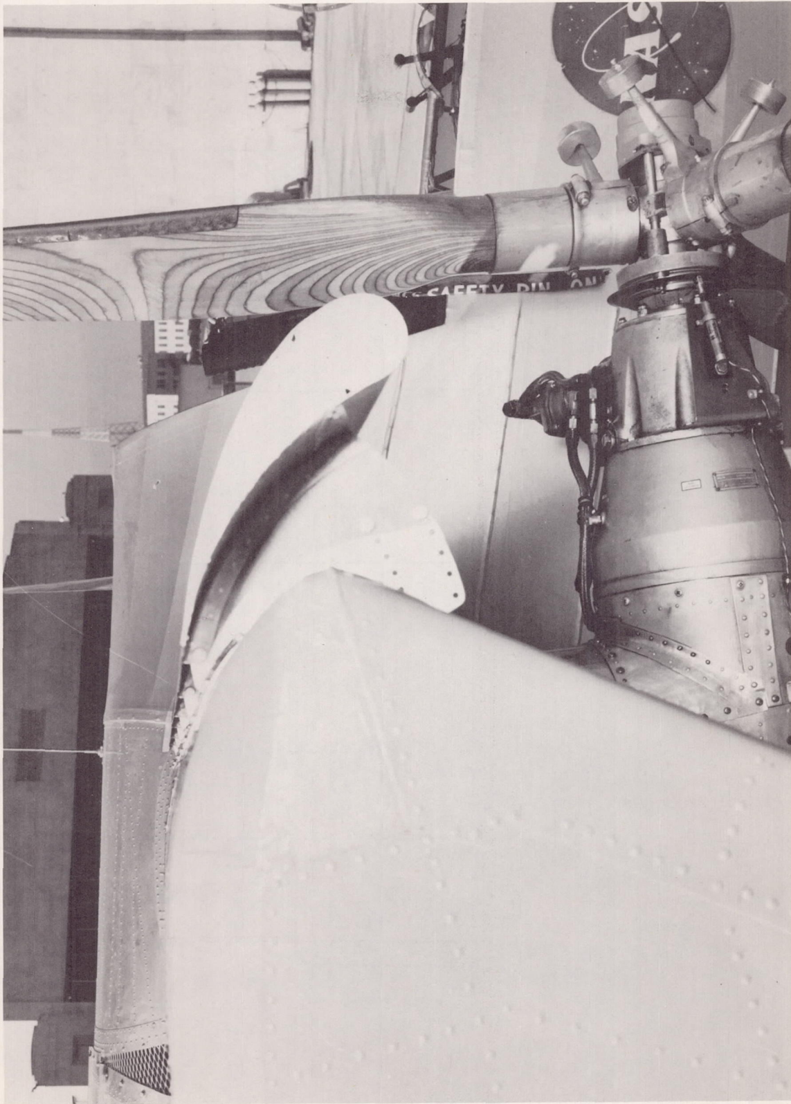
(b) Slat-wing relationship.
