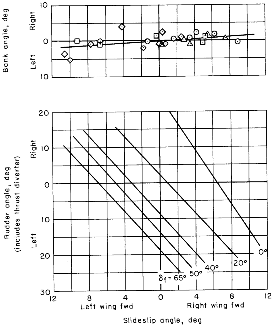
Figure 17.- Directional stability characteristics of Ryan VZ-3RY.
