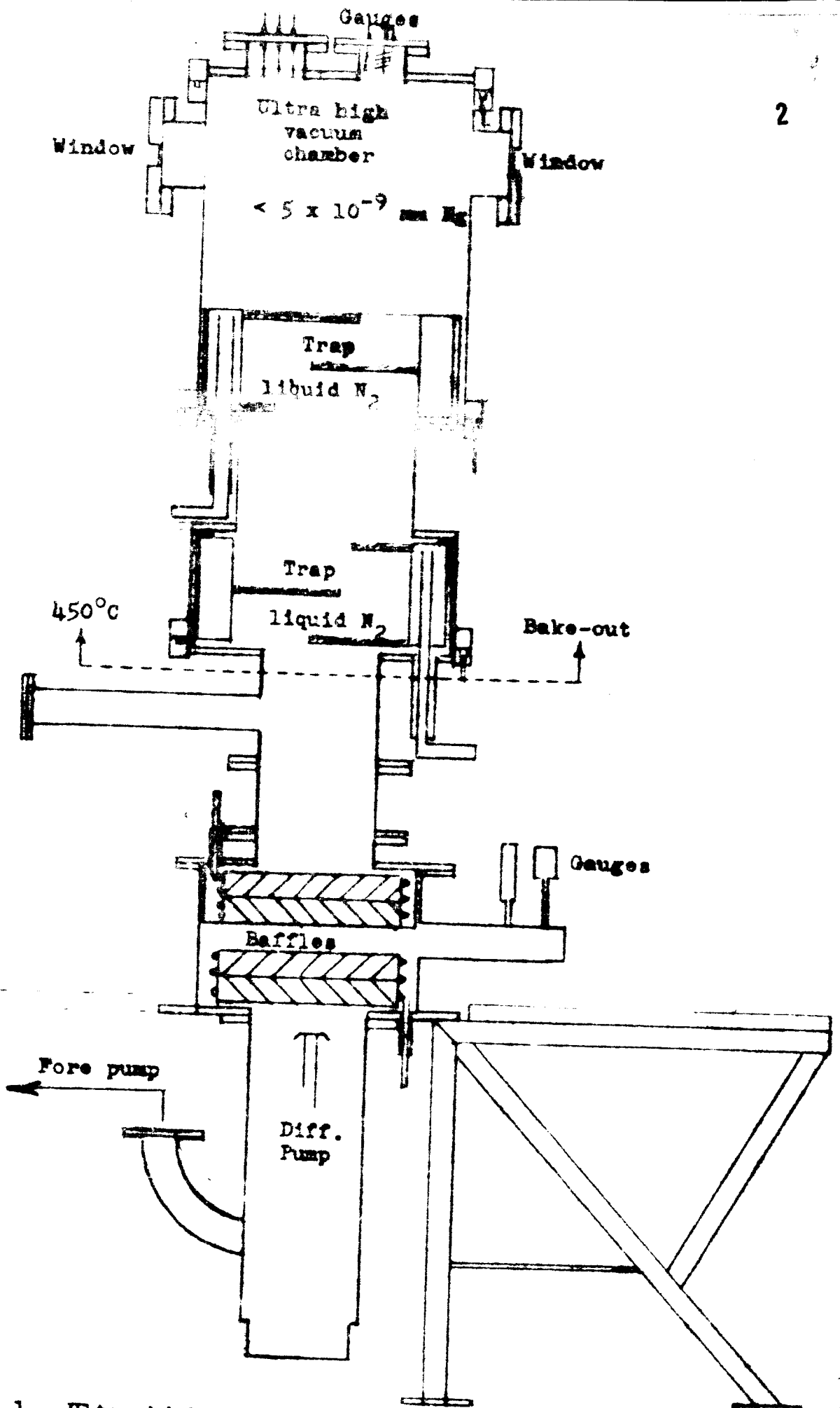
Fig. 1. Ultra high vacuum system for reflectivity measurements on ultra clean evaporated films (side view).
