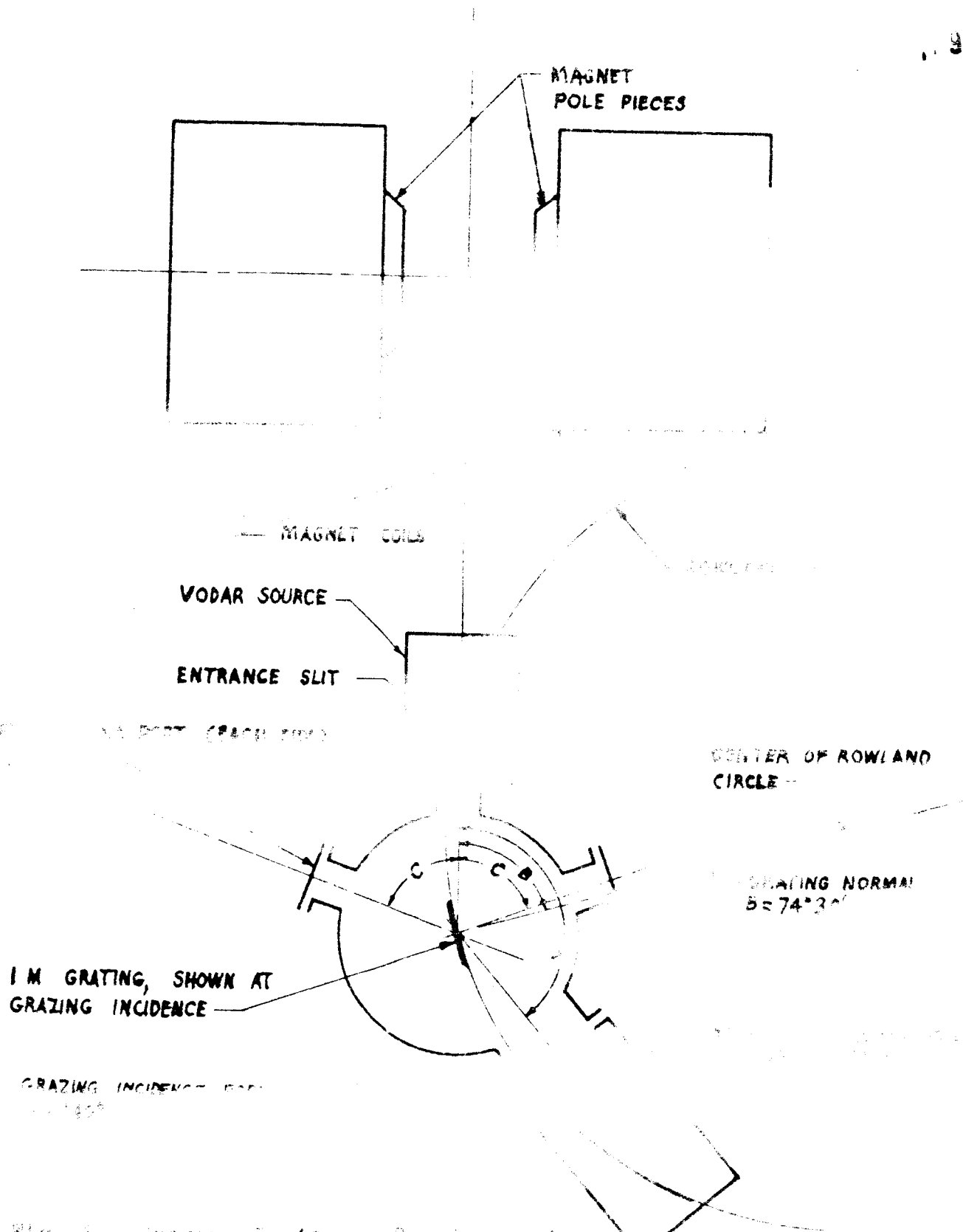
Fig. 3. Grazing Incidence Spectrograph and Monochromator designed for two purposes: light source development at shorter wavelengths (100 to 500Å), and Zeeman effect splitting of spectral lines in the vacuum ultraviolet with subsequent
