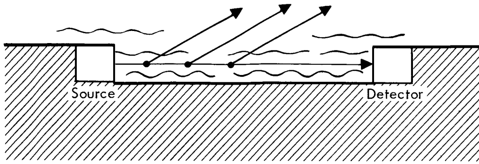
Transmission gauging
