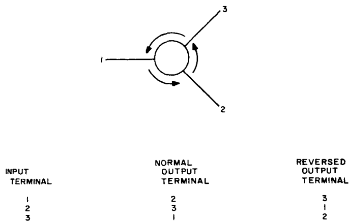
Fig. 3. Circulator switch circuit
