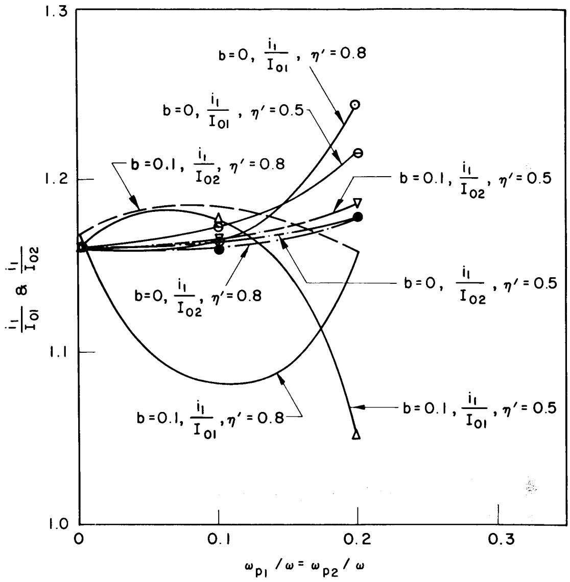
FIG. B.4 BEAM-PLASMA INTERACTION. FUNDAMENTAL CURRENT AMPLITUDE VS. \frac{\omega_p}{\omega} , b AND \eta' . ( \epsilon_1 = -1, \epsilon_2 = +1, \alpha = 0.2, I' = 0 )
