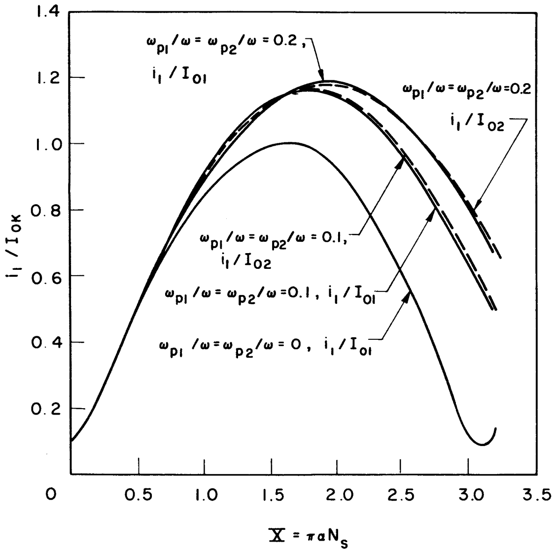
FIG. B.3 DOUBLE-BEAM INTERACTION. EFFECT OF SPACE CHARGE ON FUNDAMENTAL CURRENT AMPLITUDE. ( \epsilon_1 = \epsilon_2 = -1 , \alpha = 0.2 , I' = \eta' = 0 , b = 0 )
