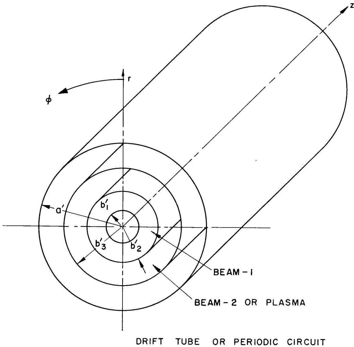
FIG. B.1 BEAM-PLASMA-CIRCUIT INTERACTION CONFIGURATION.
