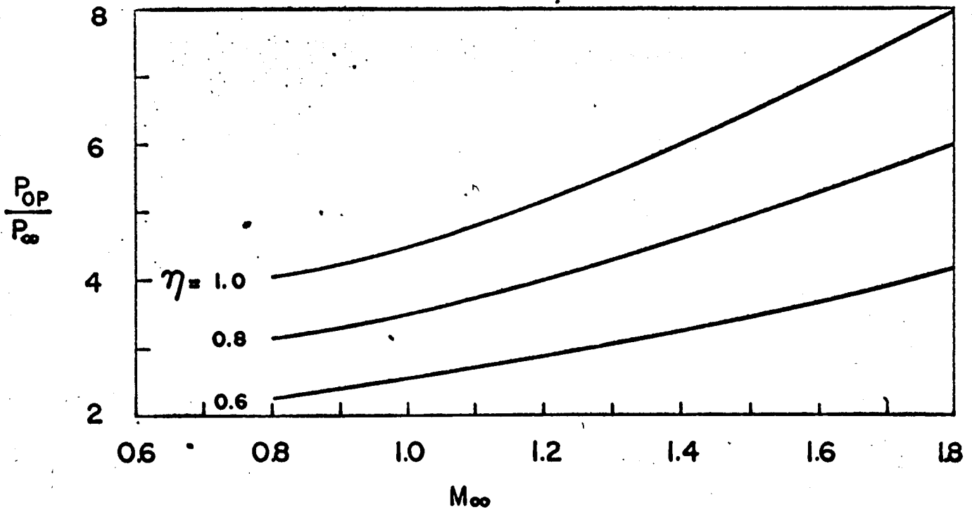
FIG. 10 THEORETICAL IN-FLIGHT P_{0p}/P_{\infty} SCHEDULE BASED ON AN EJECTOR OPERATING POINT AS AFFECTED BY INTAKE EFFICIENCY
