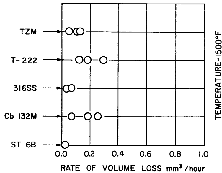
FIGURE 7 - CAVITATION DAMAGE RESISTANCE OF REFRACTORY ALLOYS IN HIGH TEMPERATURE LIQUID SODIUM (1000° AND 1500° F)
