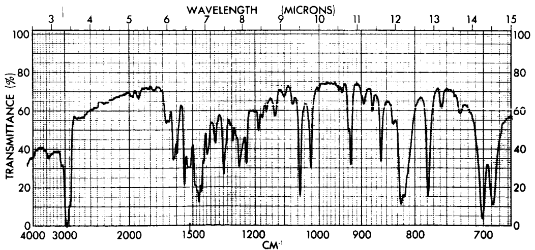
Fig. 18 - Infrared Spectrum of N,N' -Dibenzoyl-3,3'-dihydroxybenzidine Heated 2 Hr. at 300°
