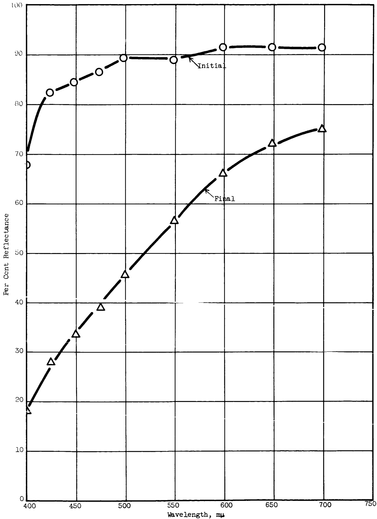
Fig. 46 - Reflectance of Plate 1 (LTV-602)
