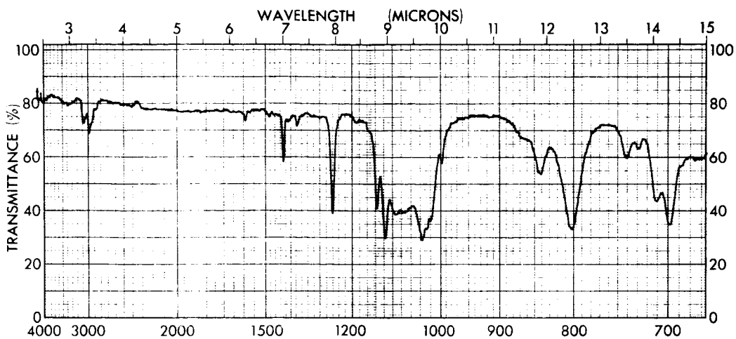
Fig. 10 - Infrared Spectrum of the Polymer from Heptamethyl-1-aza-3,5-dioxa-2,4,6-trisilacyclohexane and p -Phenylene-bis(diphenylsilanol), \eta_{sp} 0.07 (Film)
