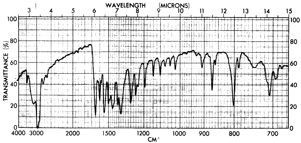
Fig. 16 - Infrared Spectrum of N,N' -Dibenzoyl-2,2'-diamino- p,p' -biphenol (Nujol)
