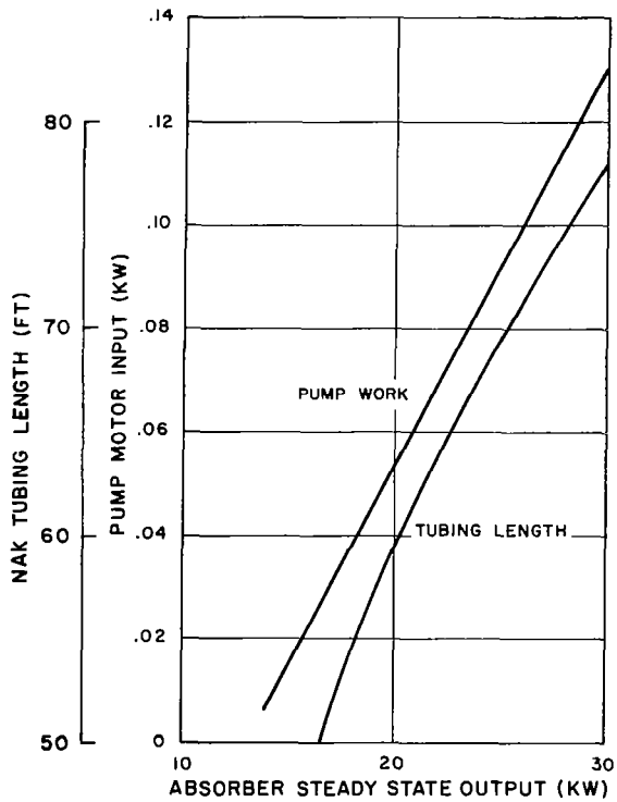
Figure 5-15. Stirling Cycle Absorber Characteristics: NaK Tubing Length Vs. Output Power
