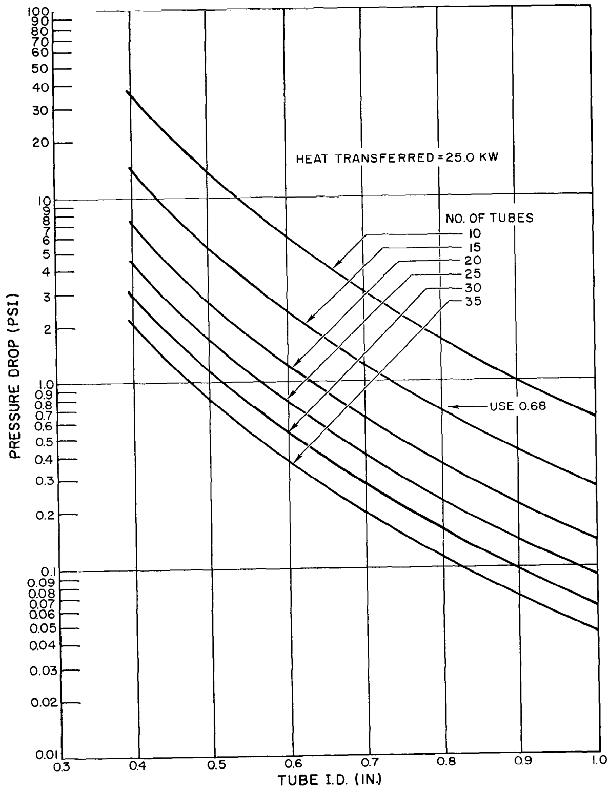
Figure 6-6. Absorber \Delta P Vs. Tube I.D.
