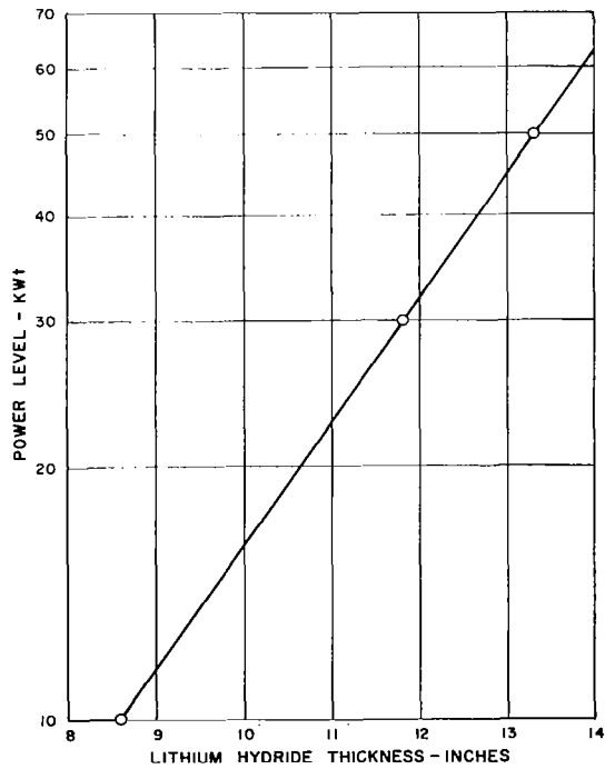
Figure 5-19. Lithium Hydride Shield Thickness
