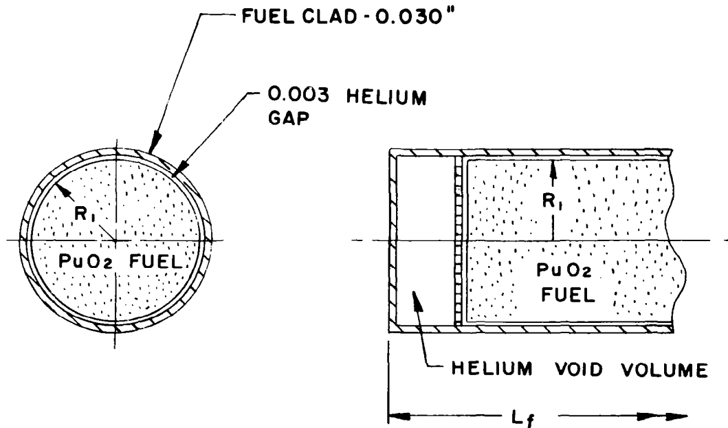
Figure 5-20. Fuel Capsule
