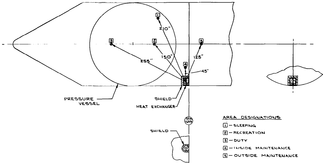
Figure 5-18. Heat Exchanger Location on Vehicle
