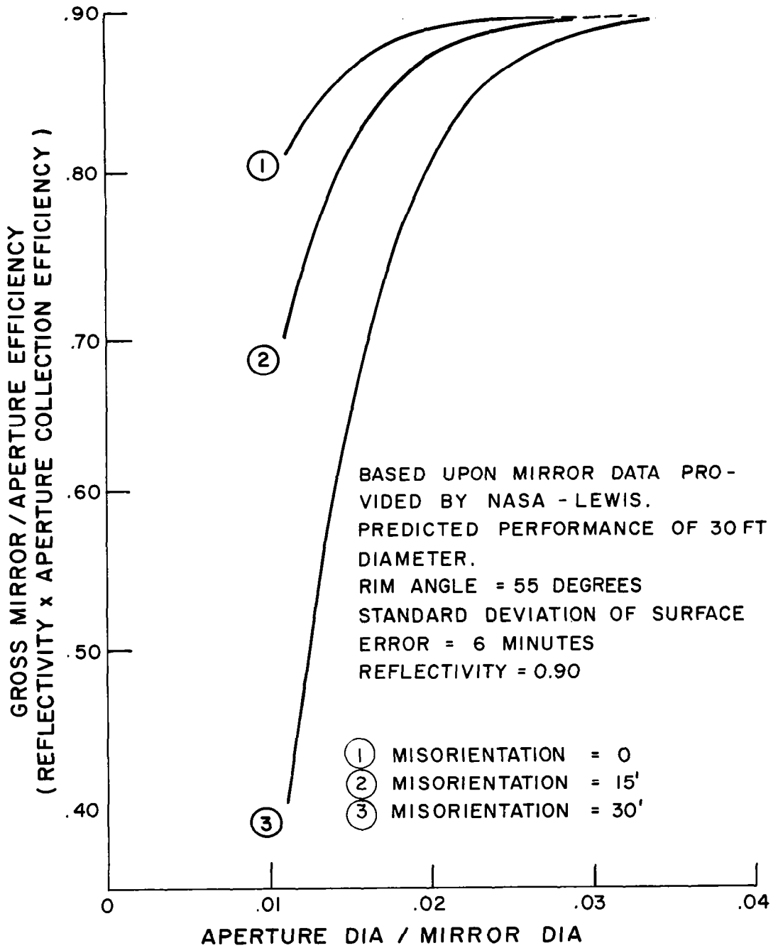
Figure B-2. Performance of Solar Collector and Absorber
