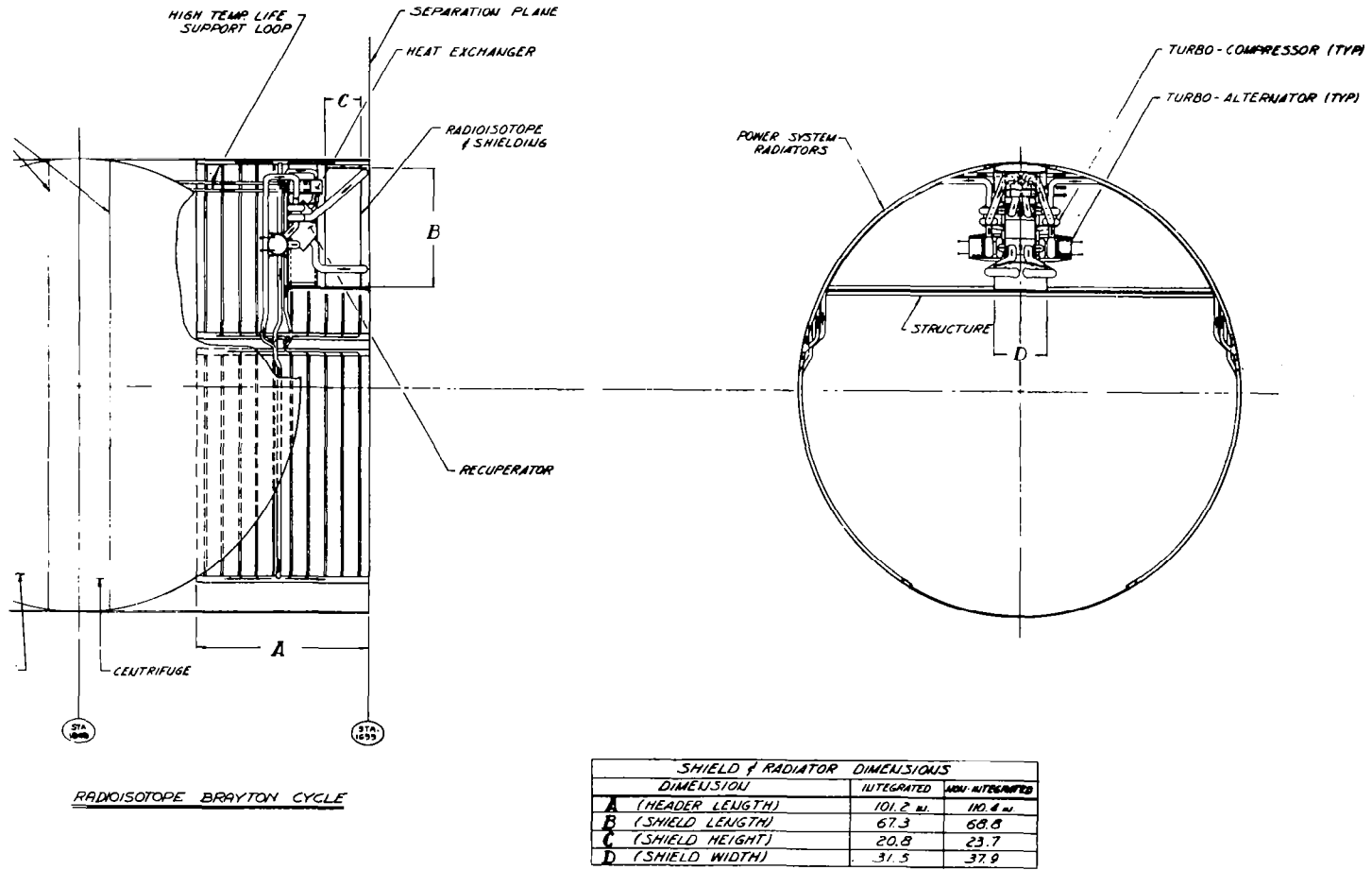
Figure 6-4. Power System Component Layout - Isotope Brayton
