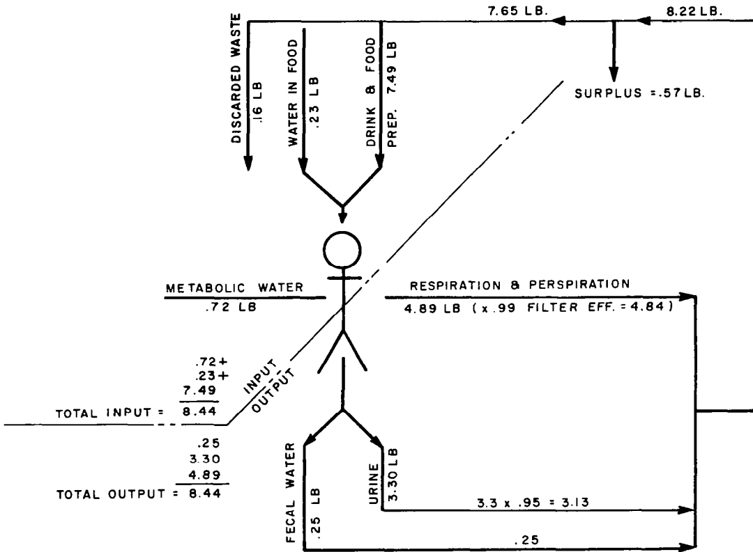
Figure 4-7. Daily Water Balance
