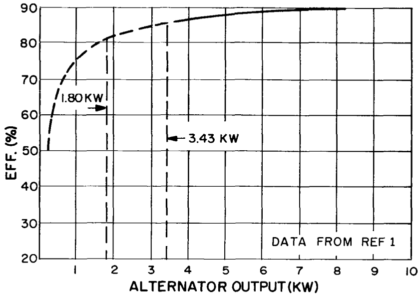
Figure 7-1. Mercury Rankine System PM Alternator Efficiency Vs. Alternator Output
