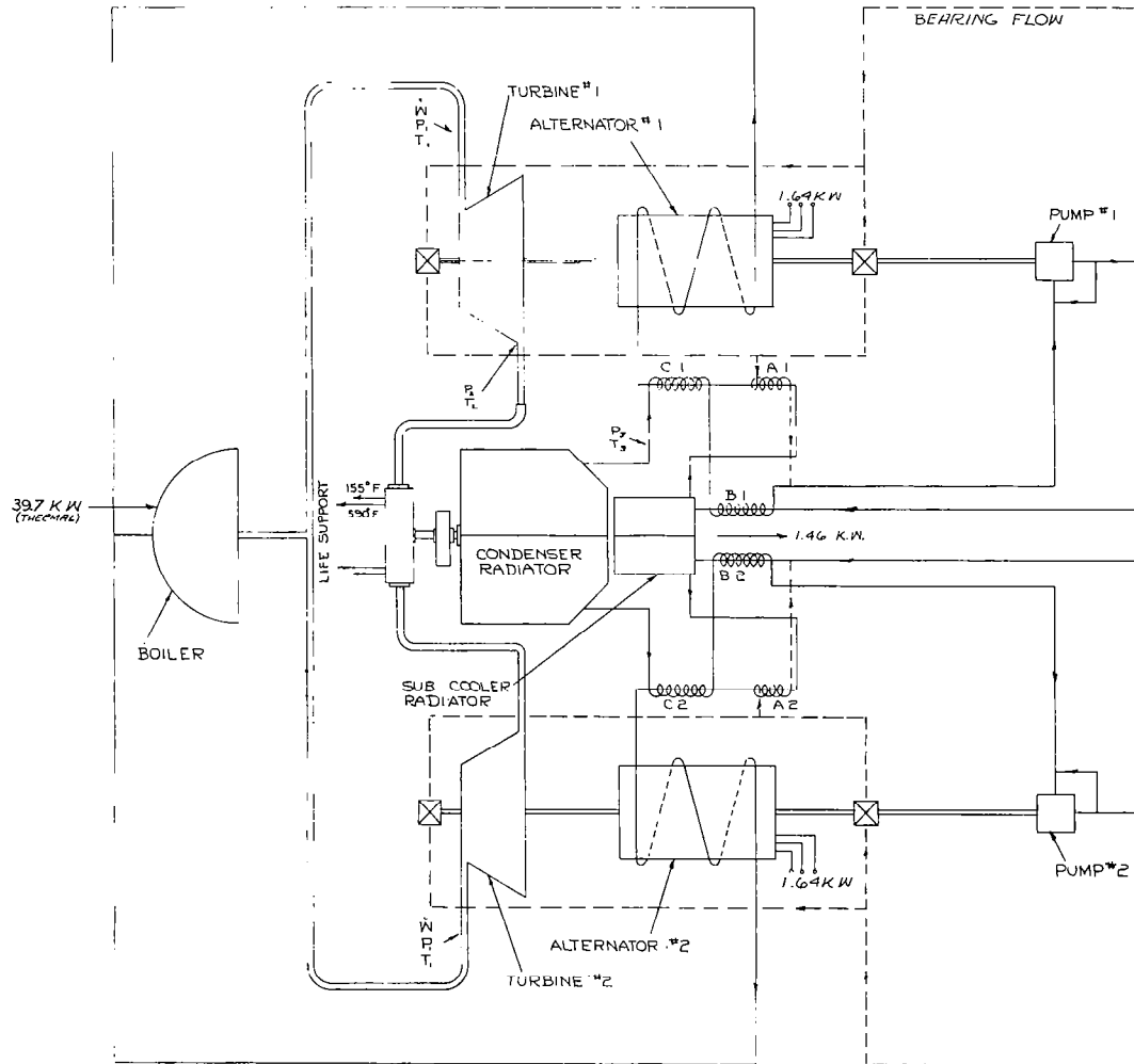
Figure 7-12. Schematic Flow Diagram-Mercury Rankine Cycle Parallel Integrated 1.64 KW Units
