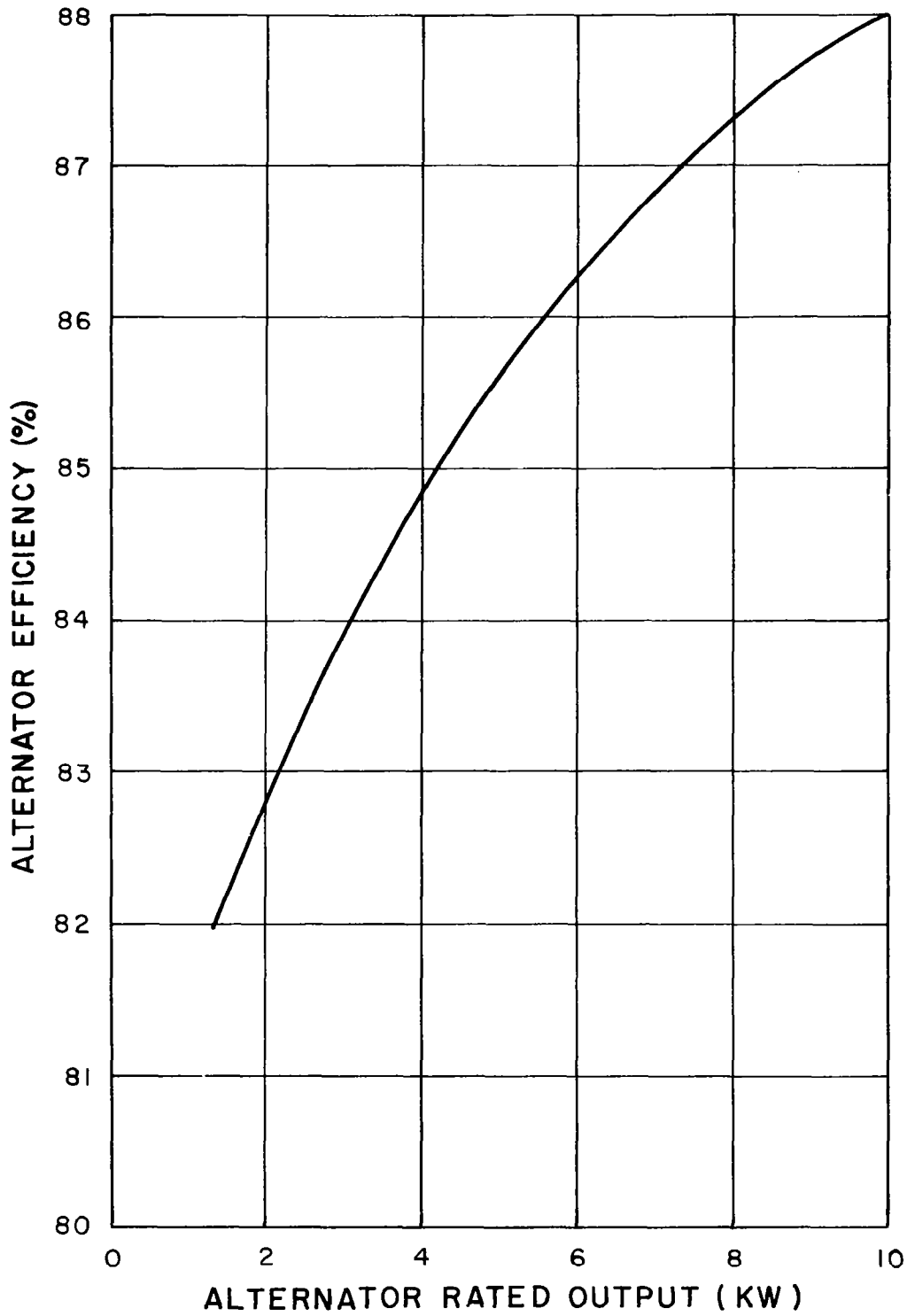
Figure 5-6. Estimated Alternator Performance
