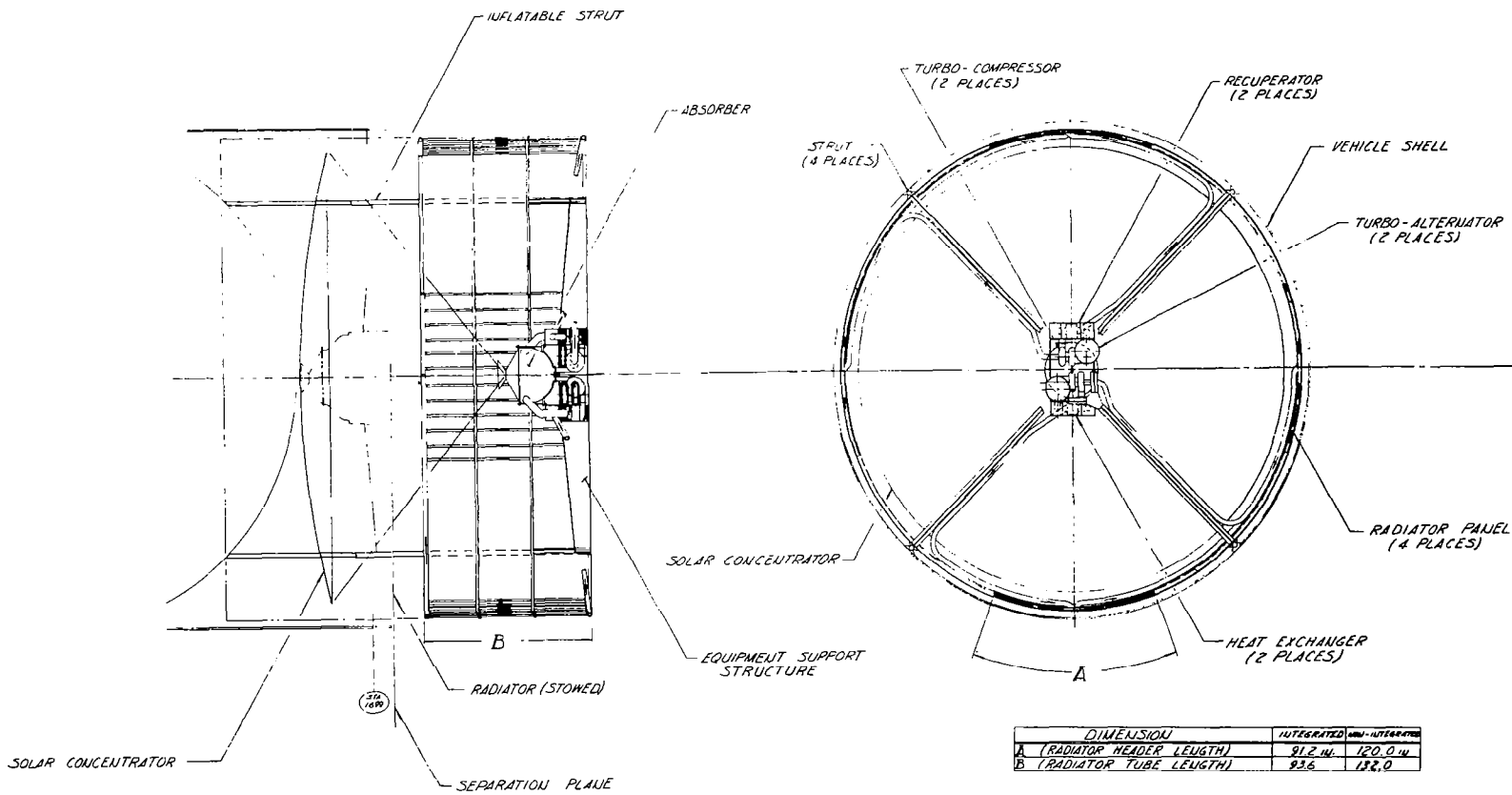
Figure 2-5. System Layout for Solar Brayton Power System
