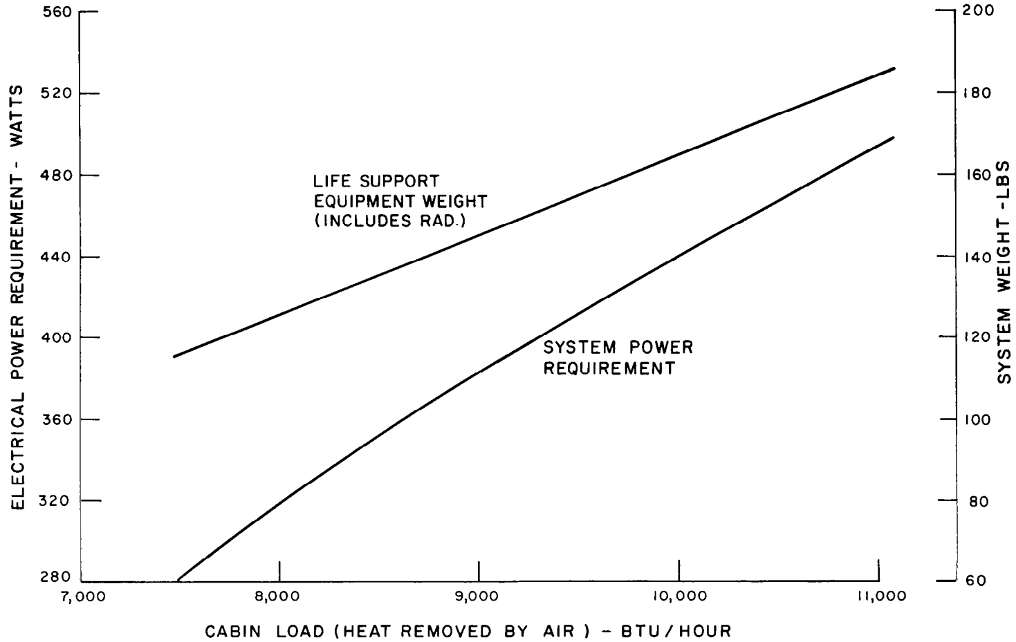
Figure 4-22. Environmental Control System Weight and Power Vs. Cabin Load Heat Requirements
