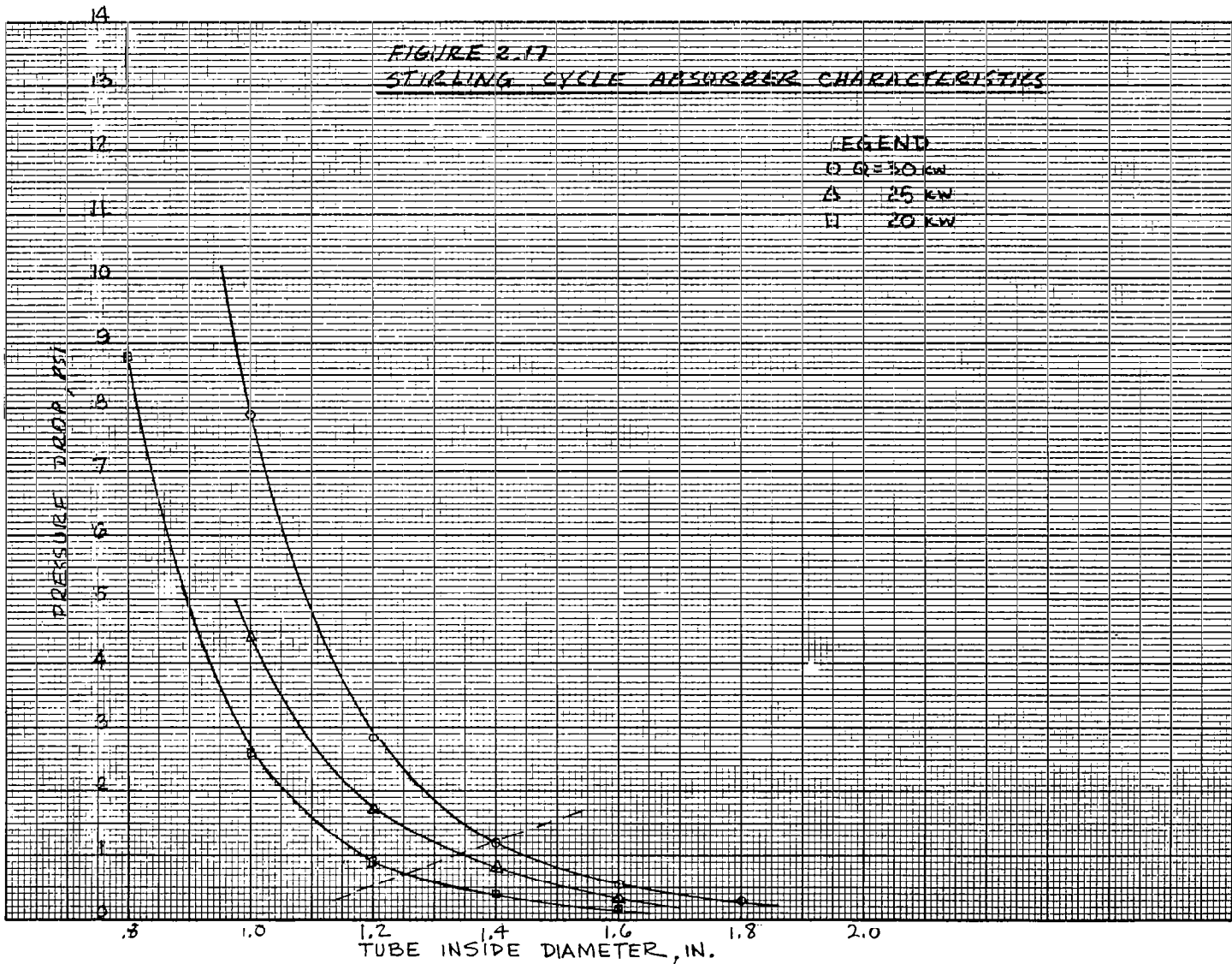
Figure C-17. Pressure Drop Vs. Tube ID
