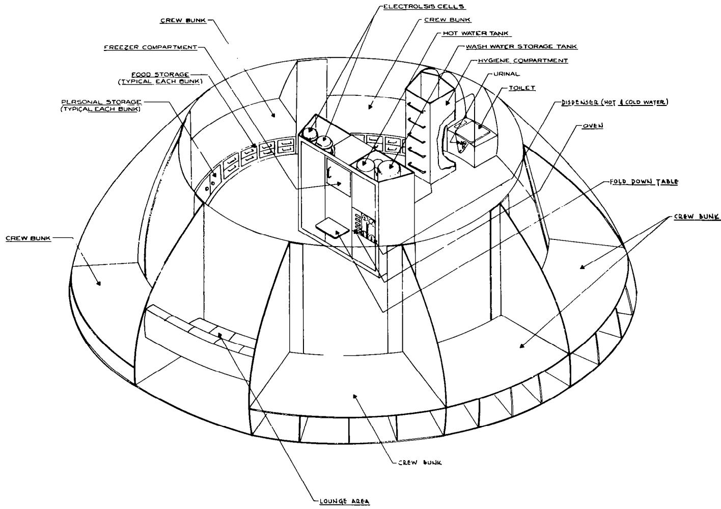
Figure 4-12. Life Support System Equipment Layout
