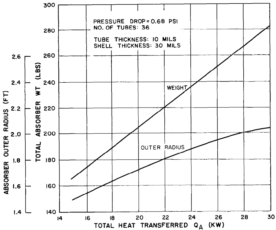
Figure 6-11. Absorber Weight Vs. Heat Transferred ( Q_A )
