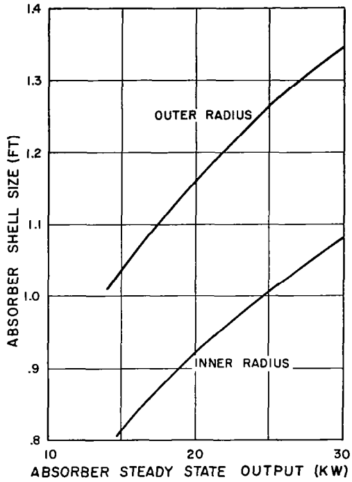
Figure 5-14. Stirling Cycle Absorber Characteristics: Shell Size Vs. Output Power
