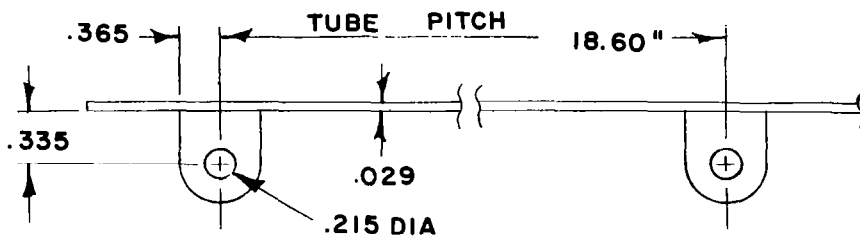
SECTION A - A IDEALIZED INTEGRAL RADIATOR
