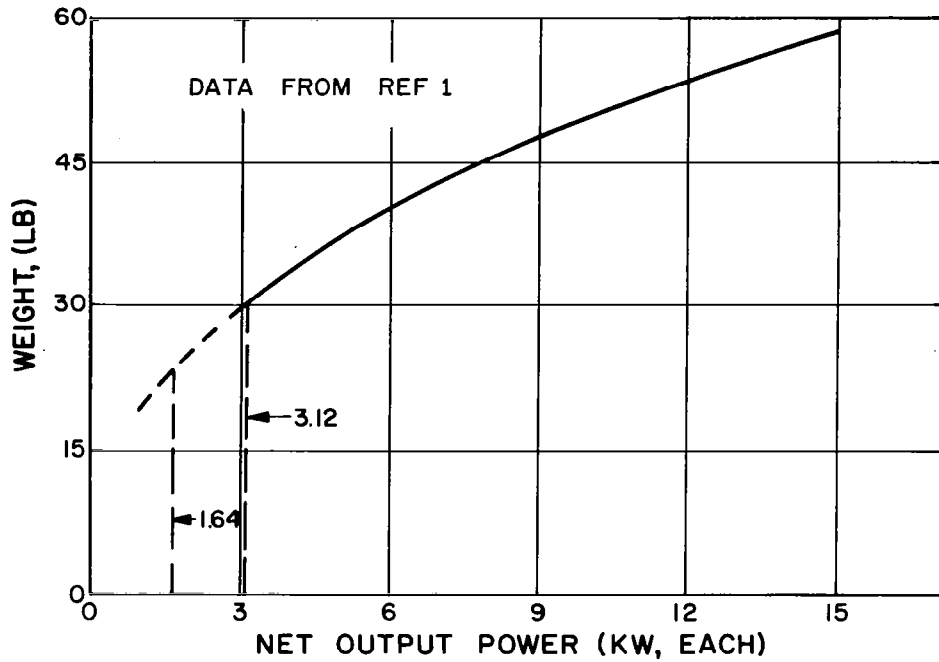
Figure 7-3. Mercury Rankine System Turbo-alternator Weight Vs. Net Output Power (PIC-SOL 209/4, SEC B-1, Fig. 39)
