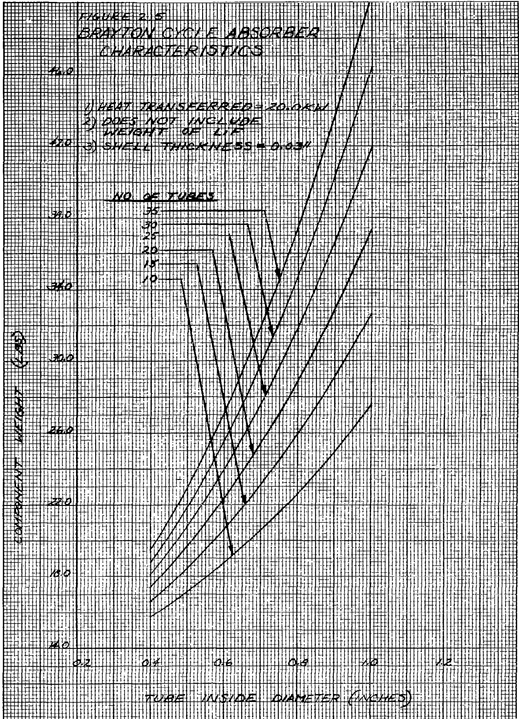
Figure C-5. Component Weight Vs. Tube ID (Heat transferred = 20.0 KW)
