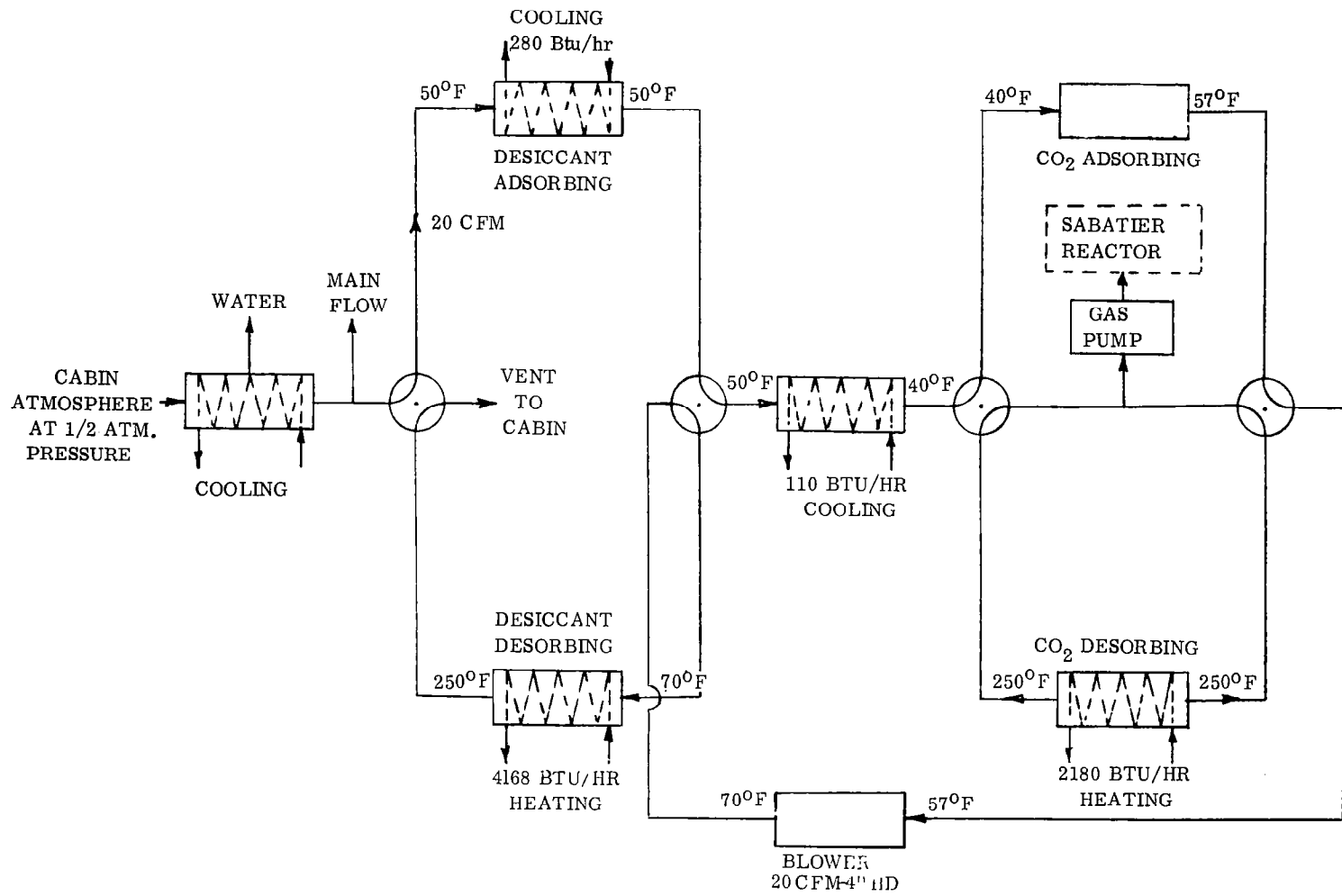
Figure 4-2. Carbon Dioxide Collection
