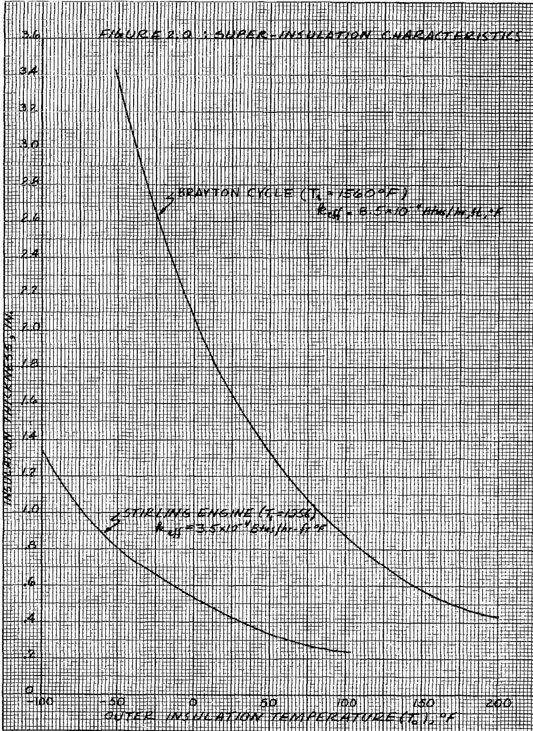
Figure C-19. Super-Insulation Characteristics: Insulation Thickness Vs. Outer Insulation Temperature
