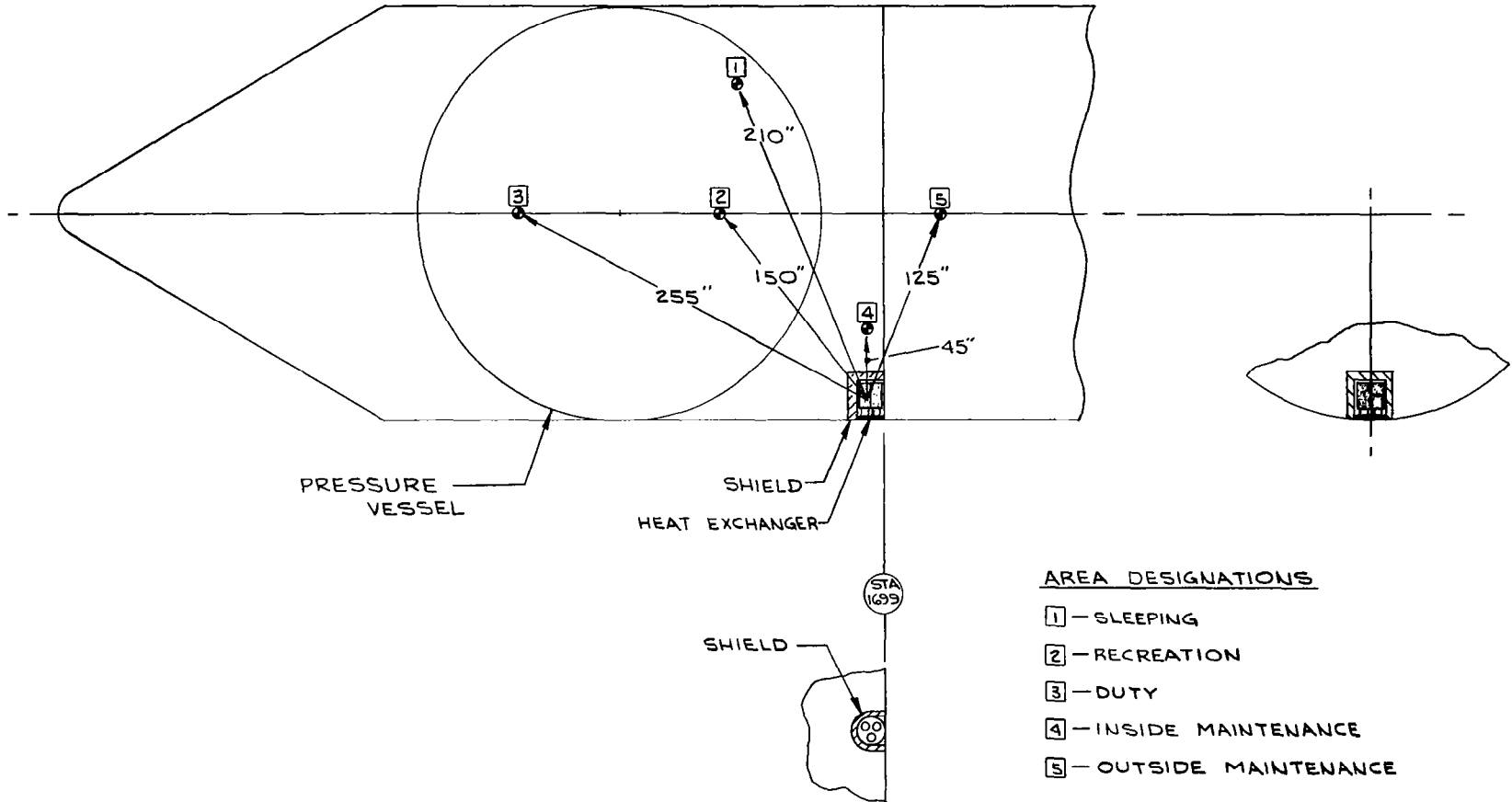
Figure 6-12. Heat Exchanger Location on Vehicle
