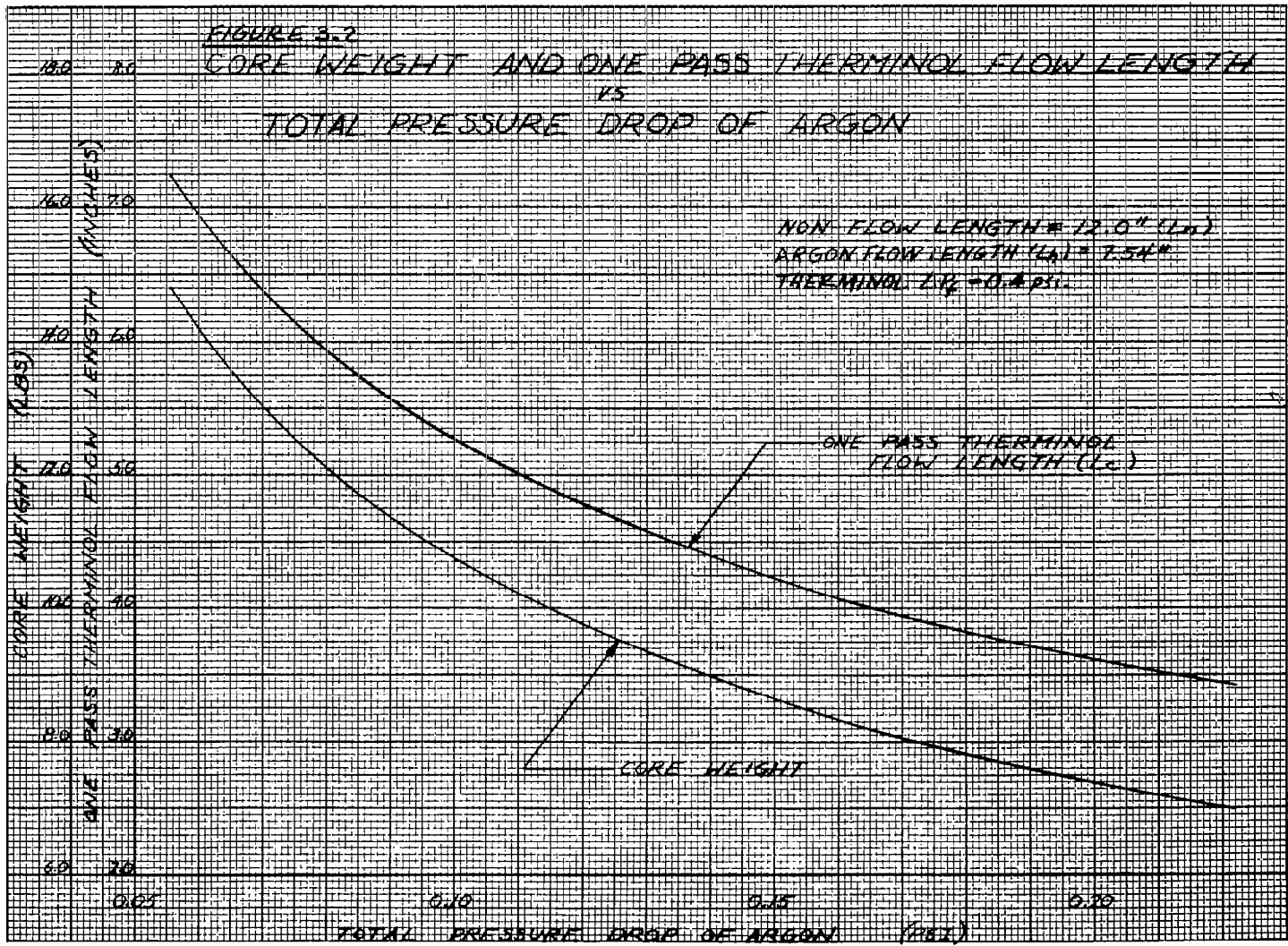
Figure C-21. Core Weight and One-Pass Therminol Flow Length Vs. Total Pressure Drop of Argon
