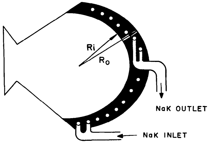
Figure 5-12. Converging-Diverging Conical Shell Aperture
