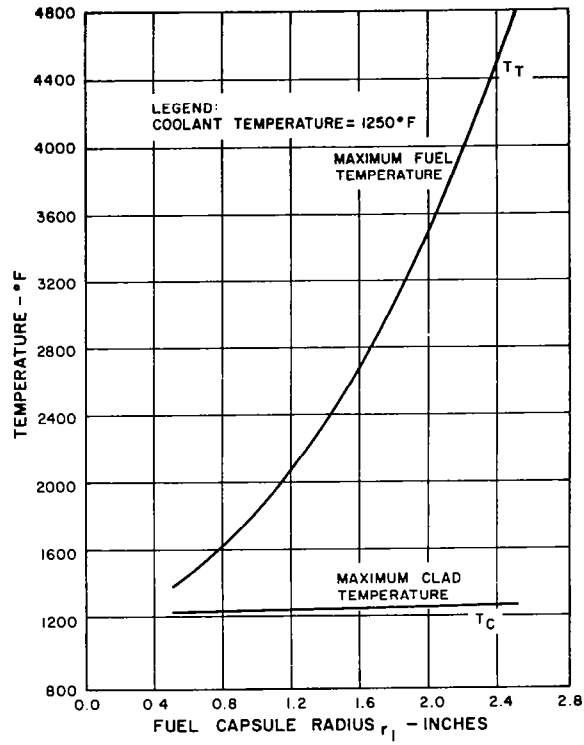
Figure 5-27. Fuel Capsule Temperatures
