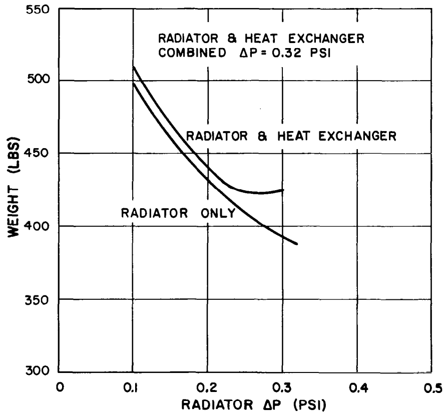
Figure 6-32. Radiator and LSS Heat Exchanger Weight
