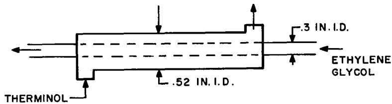
Figure 6-31. Therminol FR-1 to Ethylene Glycol Heat Exchanger
