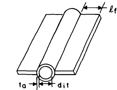
NON-INTEGRAL STRUCTURE
