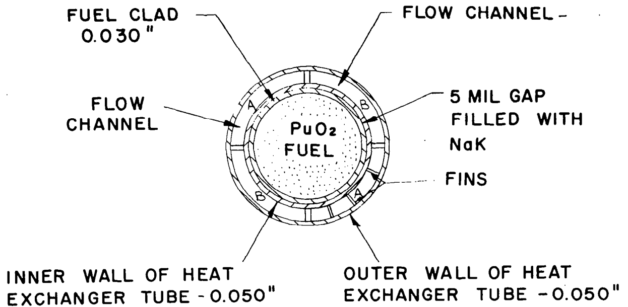
Figure 5-22. Fuel Capsule and Heat Exchanger Tube
