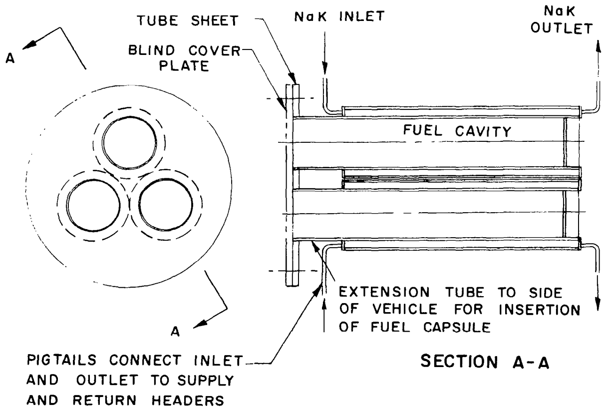
Figure 5-23. Heat Exchanger Assembly
