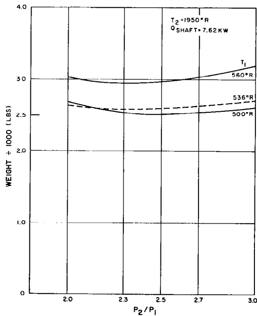
Figure 6-29. Isotope Brayton Cycle Isotope Source/Shield and Radiator Weight
