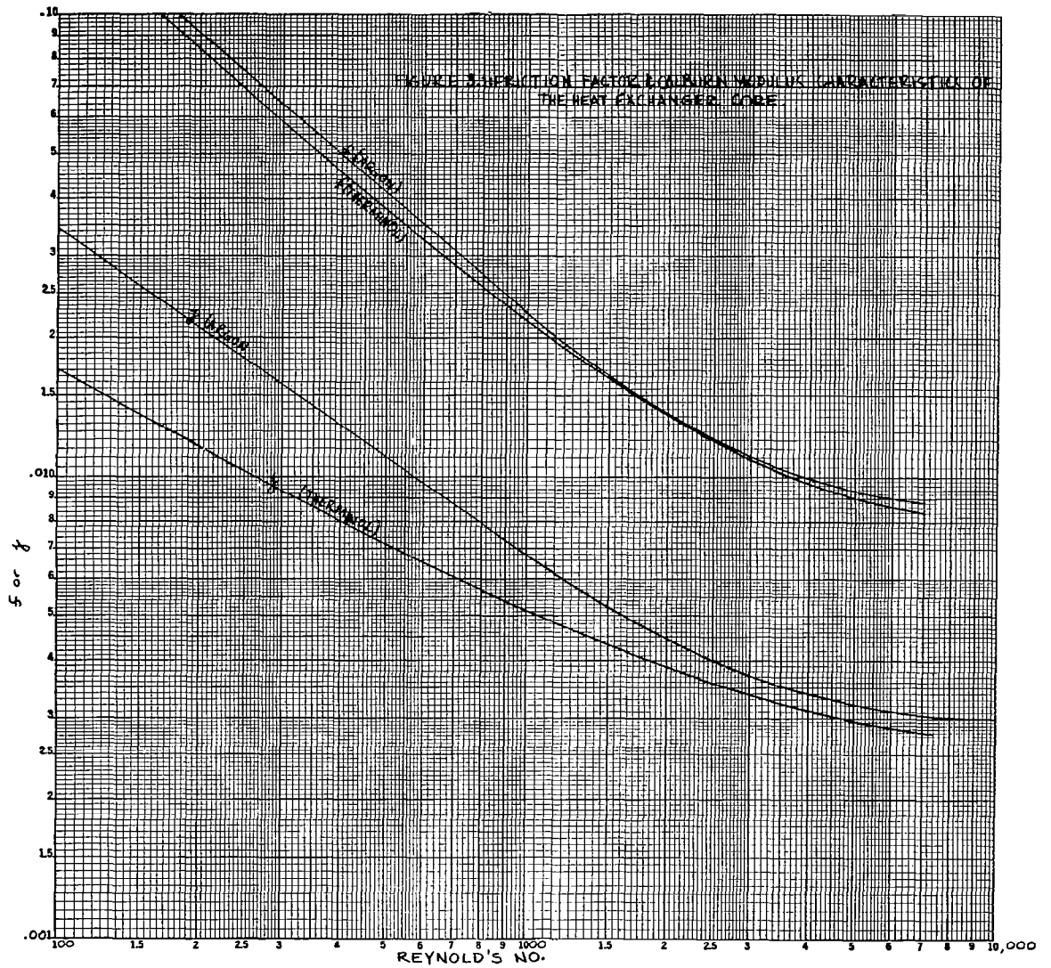
Figure C-20. Friction Factor and Colburn Modulus Characteristics of the Heat Exchanger Core
