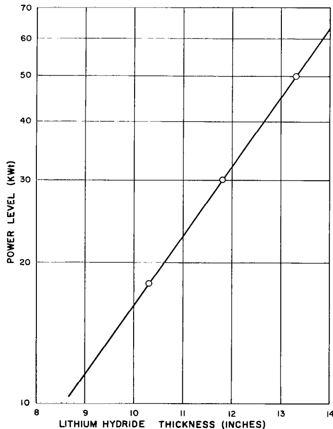
Figure 6-13. Isotope Brayton Lithium Hydride Shield Thickness
