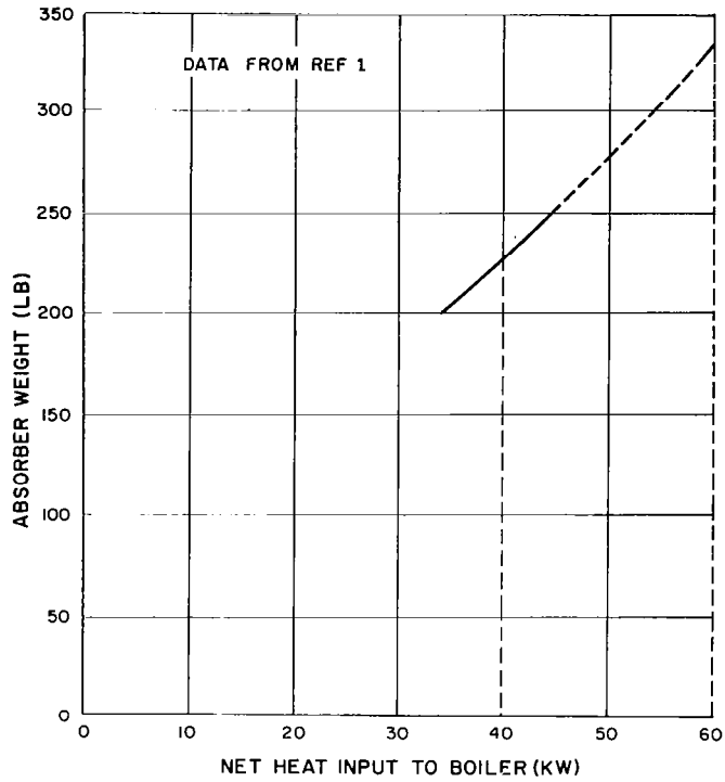
Figure 7-7. Mercury-Rankine System Absorber Weight Vs. Net Heat Input to Boiler (PIC-SOL 209/4, SEC B-1, Fig. 51, 53)
