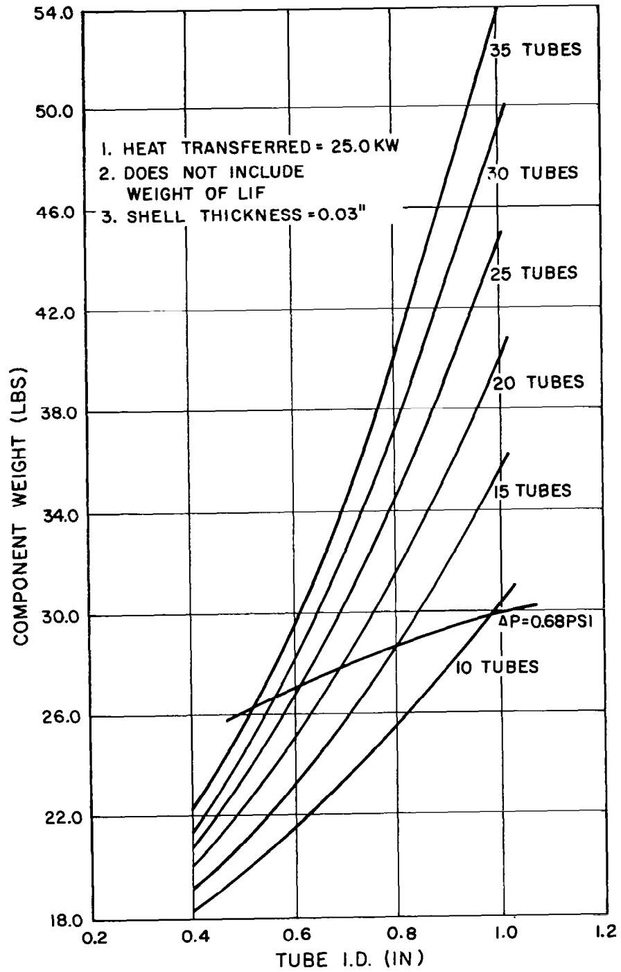
Figure 6-7. Absorber Component Weight Vs. Tube I.D.
