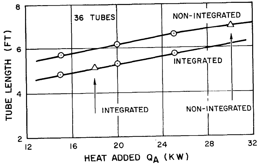
Figure 6-10. Absorber Heat Vs. Tube Length
