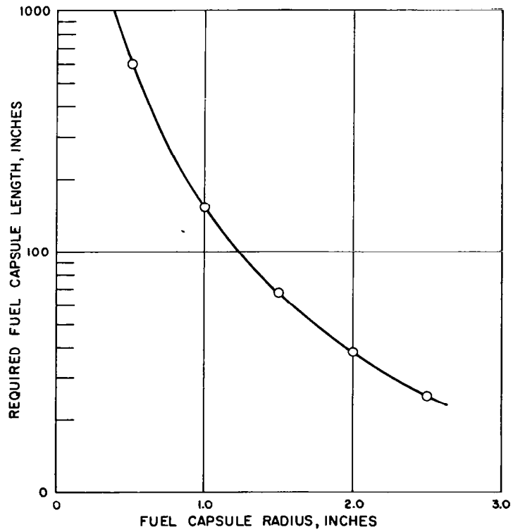
Figure 5-28. Total Fuel Capsule Length Versus Capsule Radius
