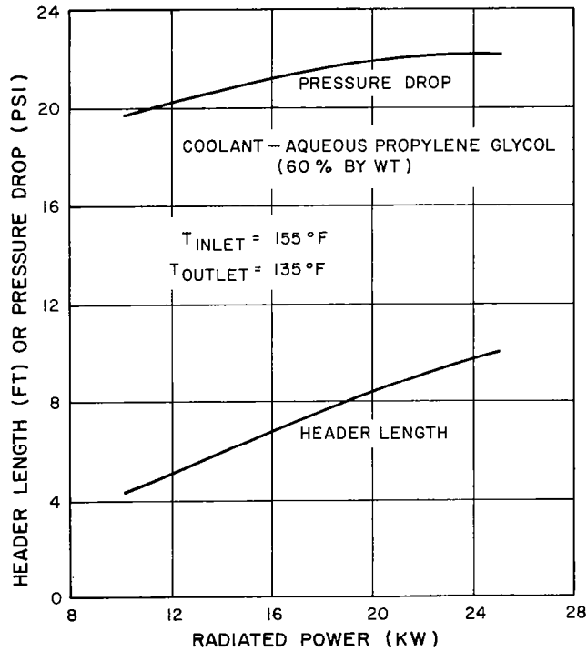
Figure 5-9. Characteristics of Engine Coolant Radiator (Integral with MORL Vehicle)
