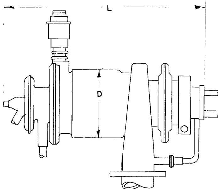
Figure 7-4. Turbo-alternator and Pump
