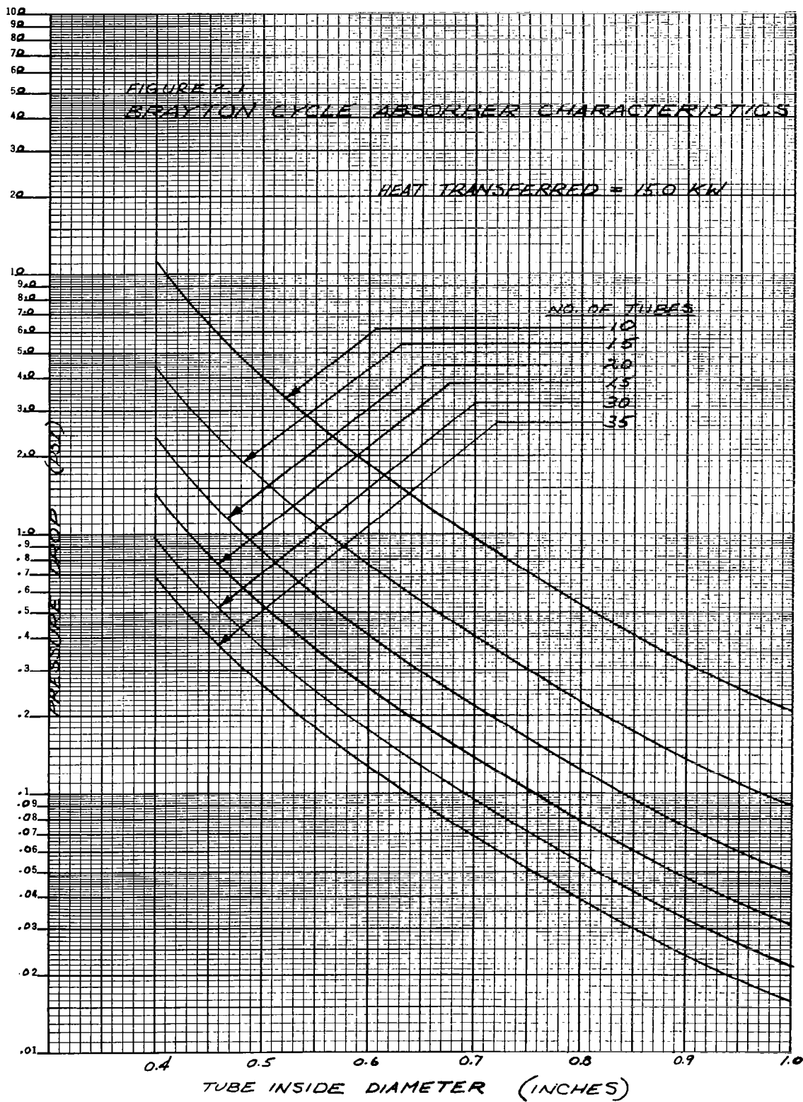
Figure C-1. Pressure Drop Vs. Tube ID (Heat transferred = 15.0 KW)
