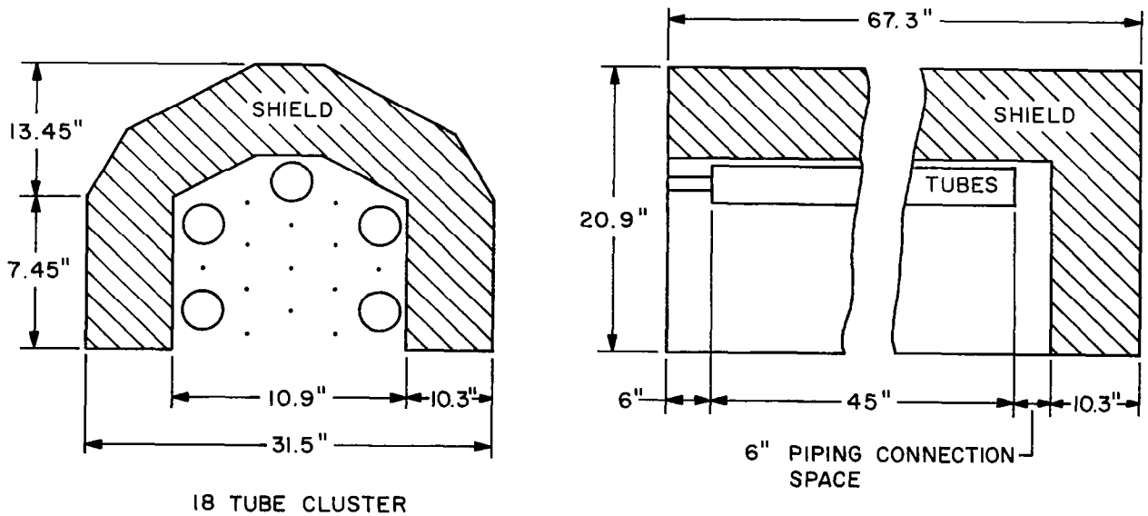
Figure 6-18. Isotope Heat Exchanger and Shield, Integrated System
