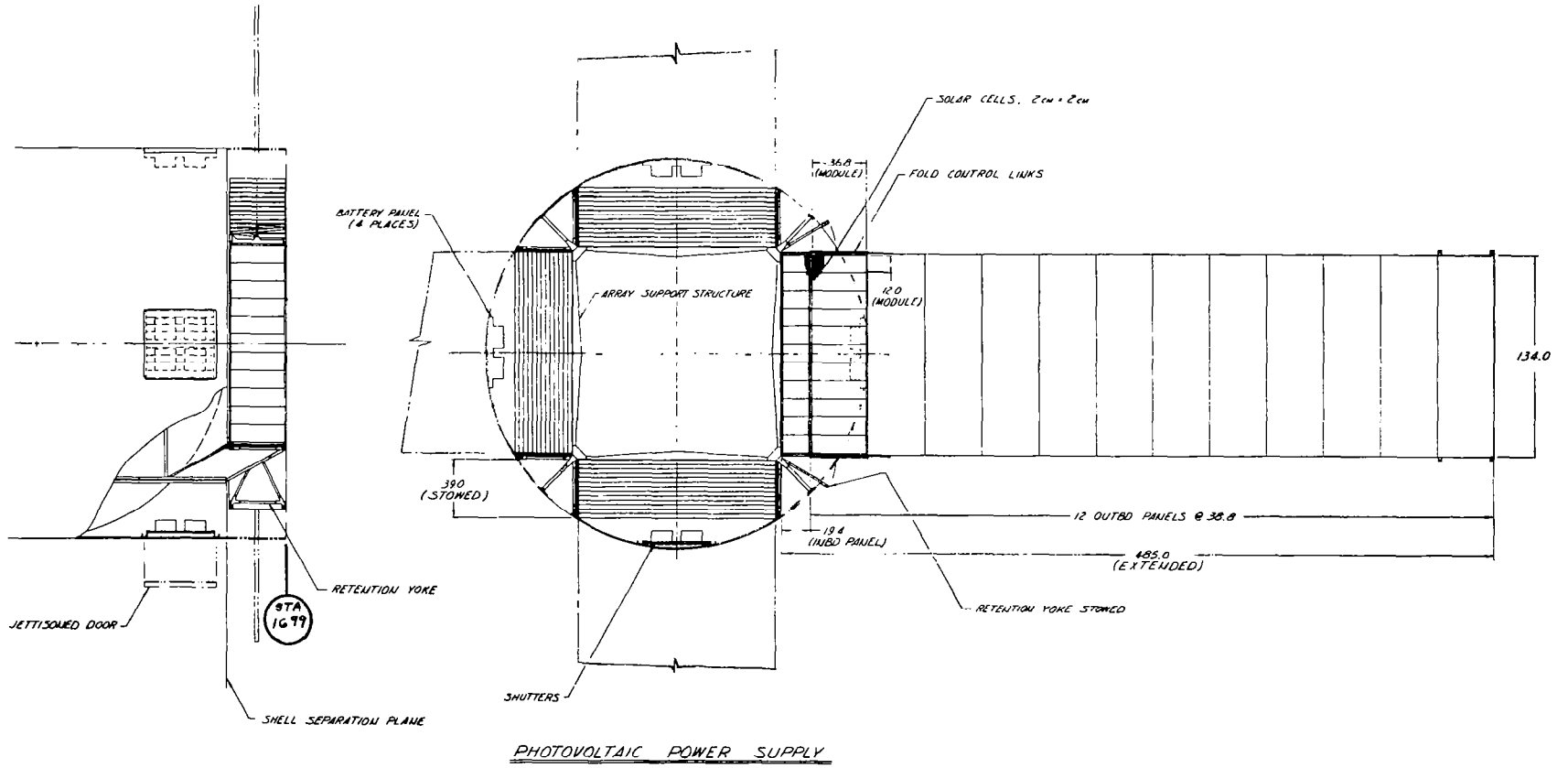
Figure 2-8. System Layout for Photovoltaic Power System
