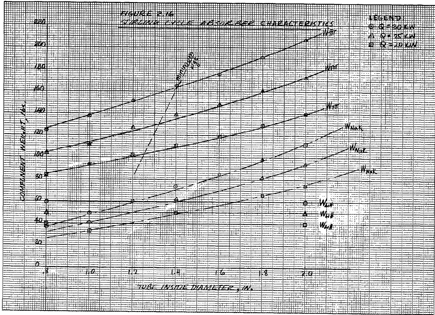
Figure C-16. Component Weight Vs. Tube ID ( W_{NaK} )
