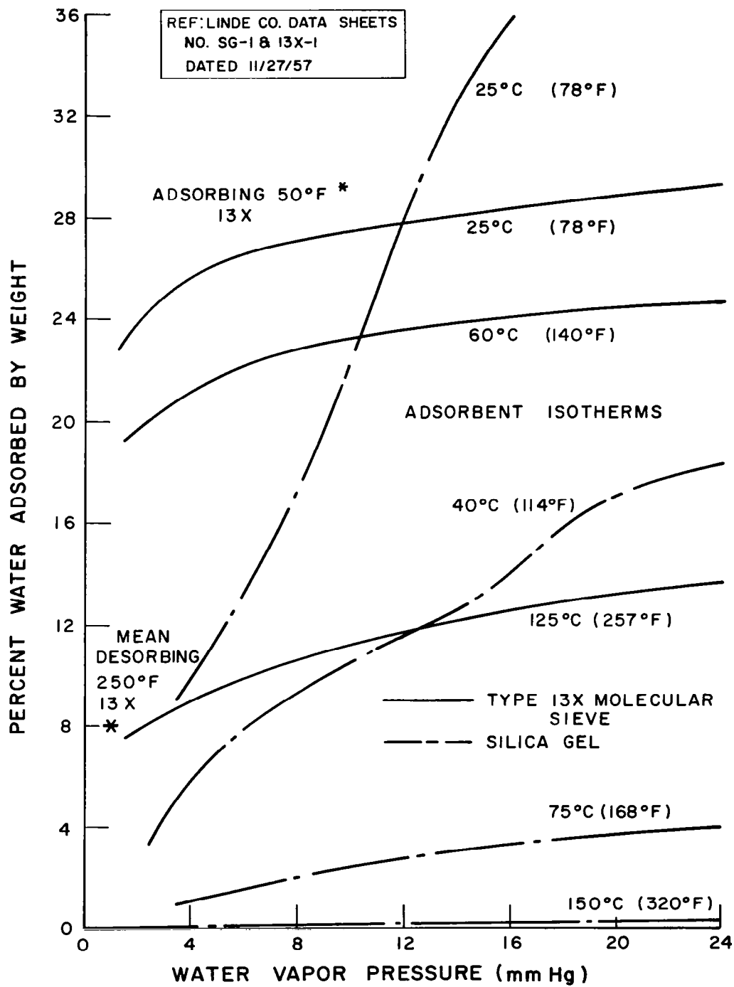
Figure 4-3. Water Vapor Adsorbent Characteristics
