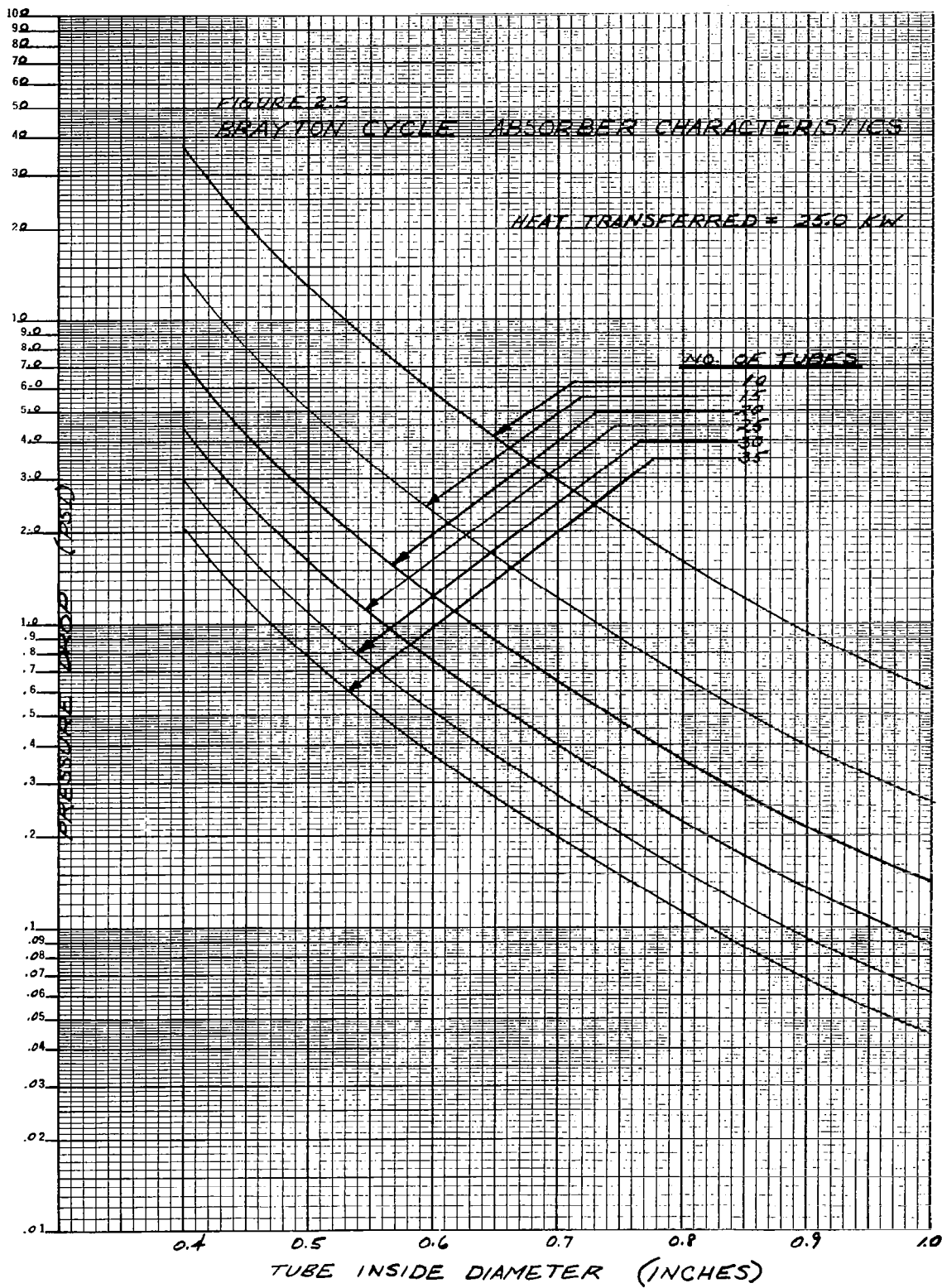
Figure C-3. Pressure Drop Vs. Tube ID (Heat transferred = 25.0 KW)
