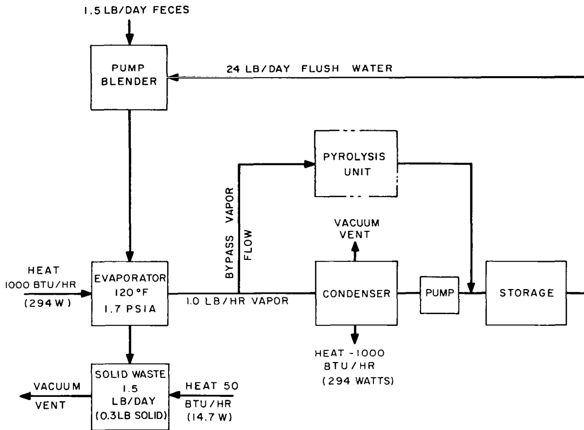
Figure 4-10. Fecal Solid Waste Management System
