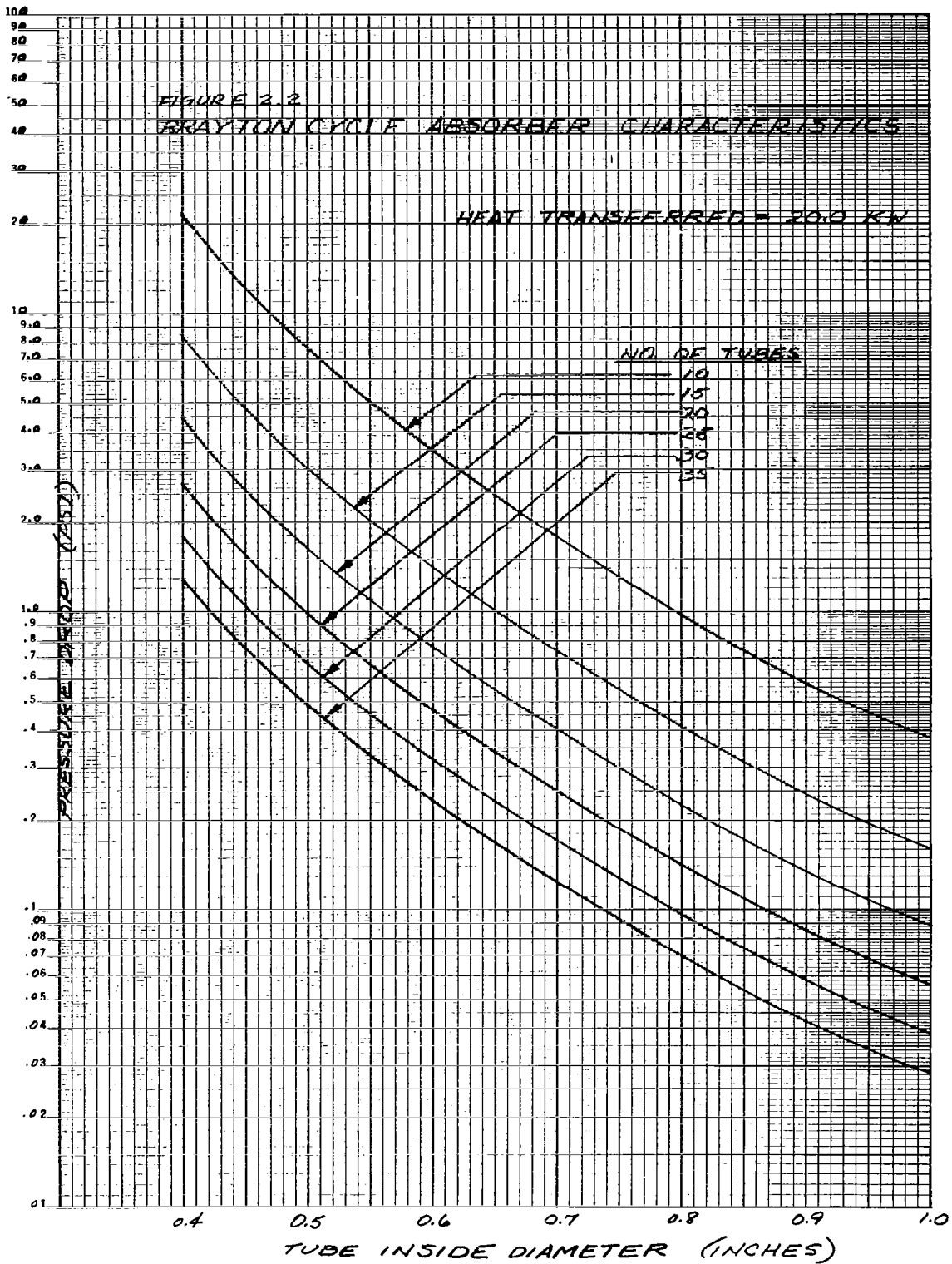
Figure C-2. Pressure Drop Vs. Tube ID (Heat transferred = 20.0 KW)
