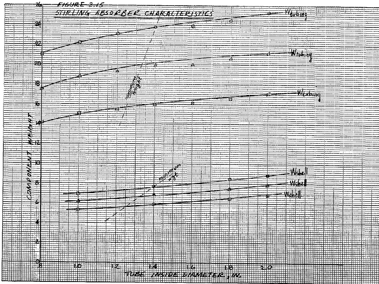
Figure C-15. Component Weight Vs. Tube ID ( W_{tubing} )
