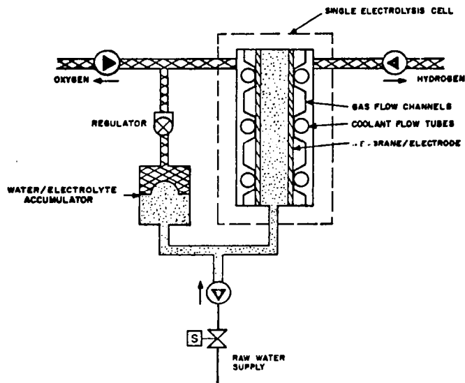
Figure 4-5. Functional Schematic of a Single Electrolysis Cell
