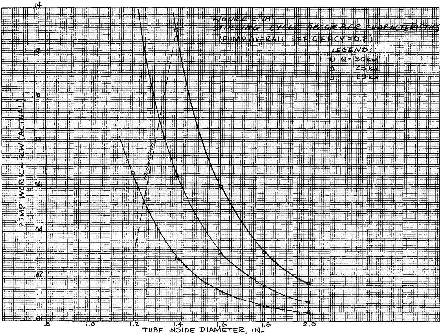
Figure C-18. Pump Work Vs. Tube ID
