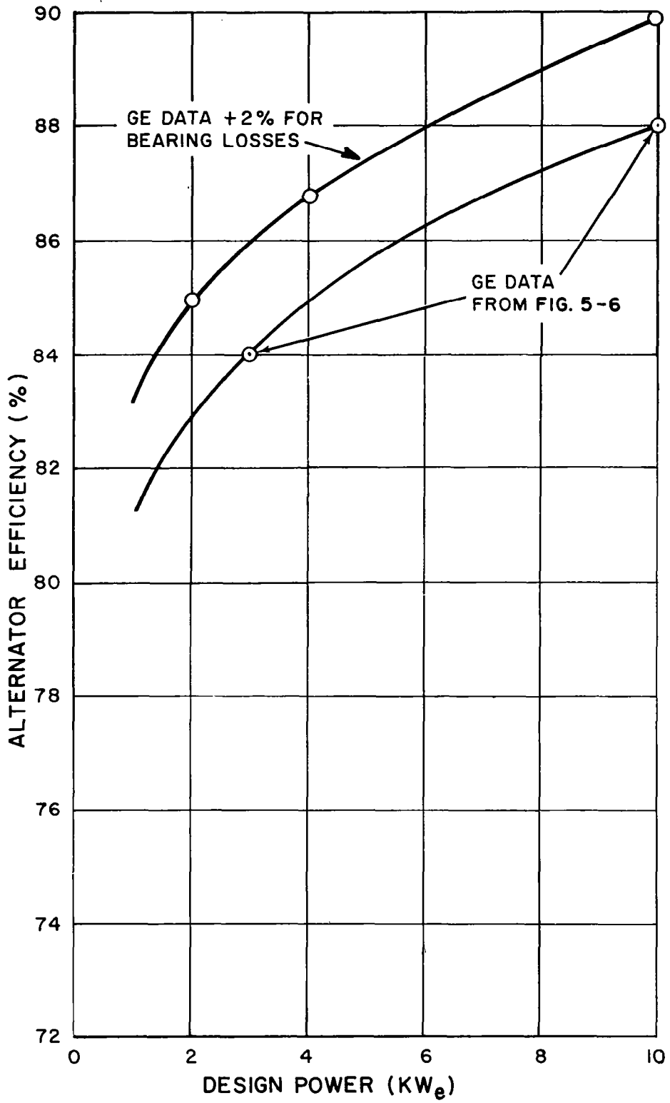
Figure 6-23. Brayton Cycle Alternator Performance
