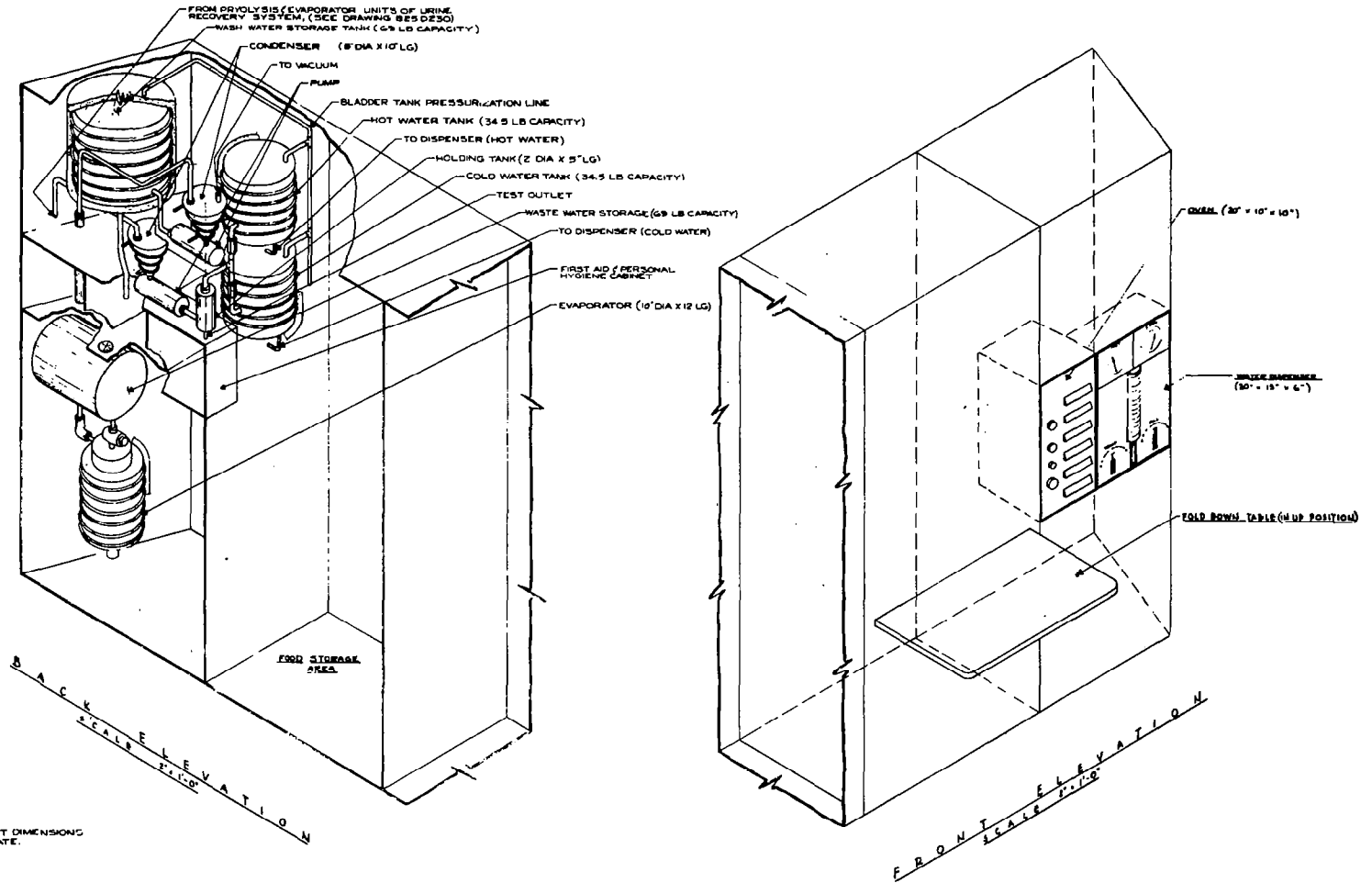
Figure 4-16. Water Recovery and Dispensing Equipment Layout
