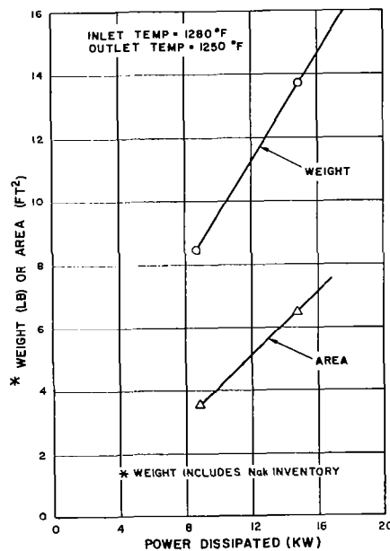
Figure 5-30. Isotope Temperature Control Radiator
