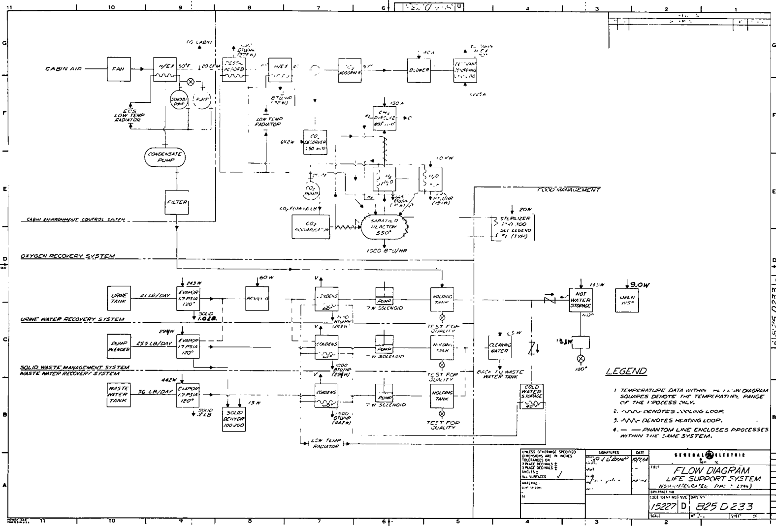
Figure 2-1. System Layout for Non-Integrated Life Support System
