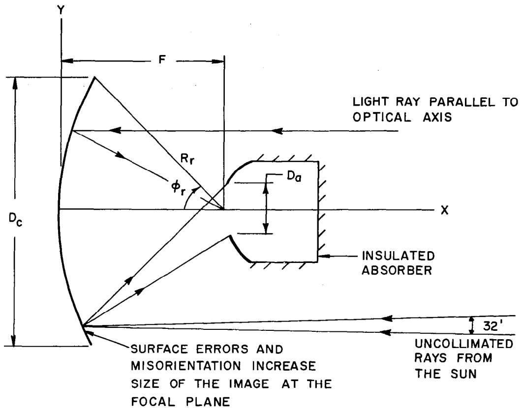
Figure B-1. Mirror/Aperture Nomenclature
