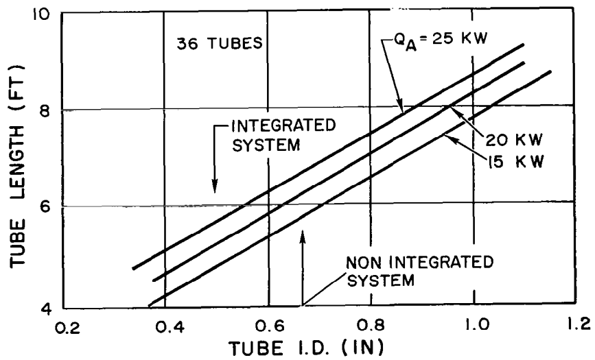
Figure 6-9. Absorber Tube Length Vs. Tube I. D.
