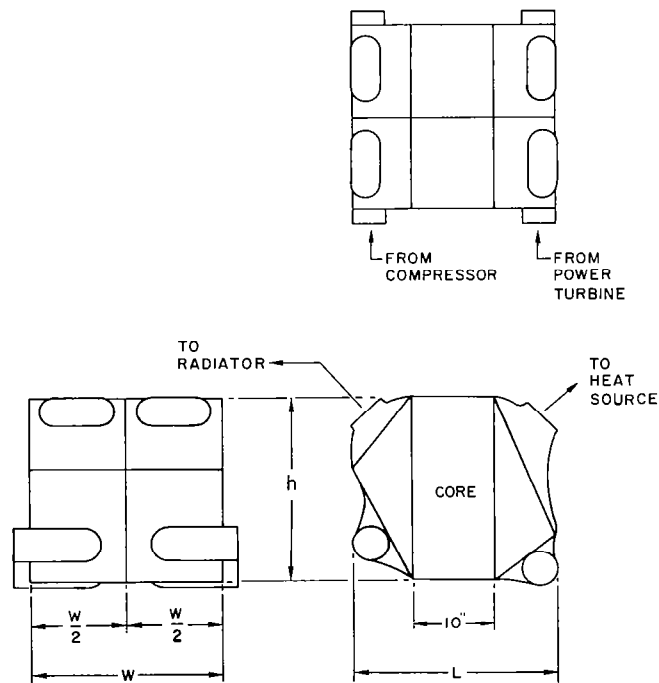
Figure 6-28. Recuperator
