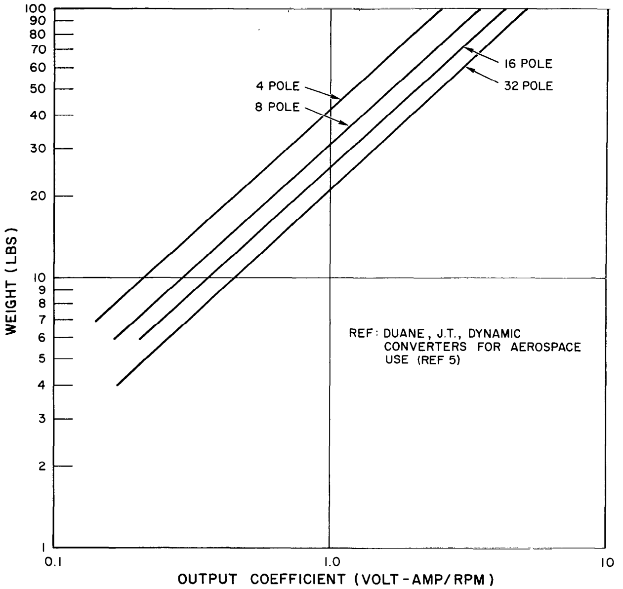
Figure 5-5. Weight Variation with Output for Space Application Type Solid Rotor AC Generator
