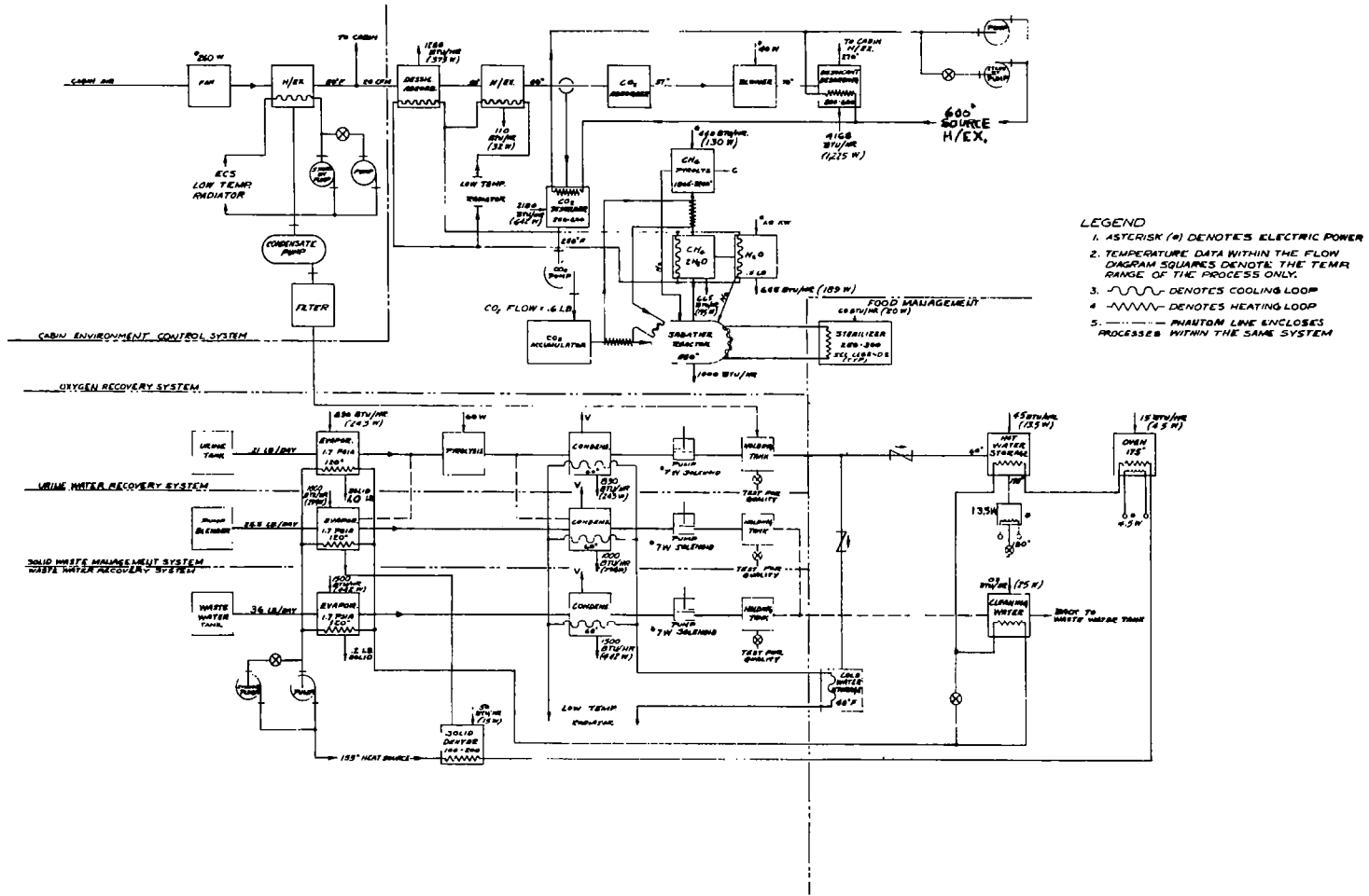
Figure 4-18. Flow Diagram - Life Support System - Integrated
