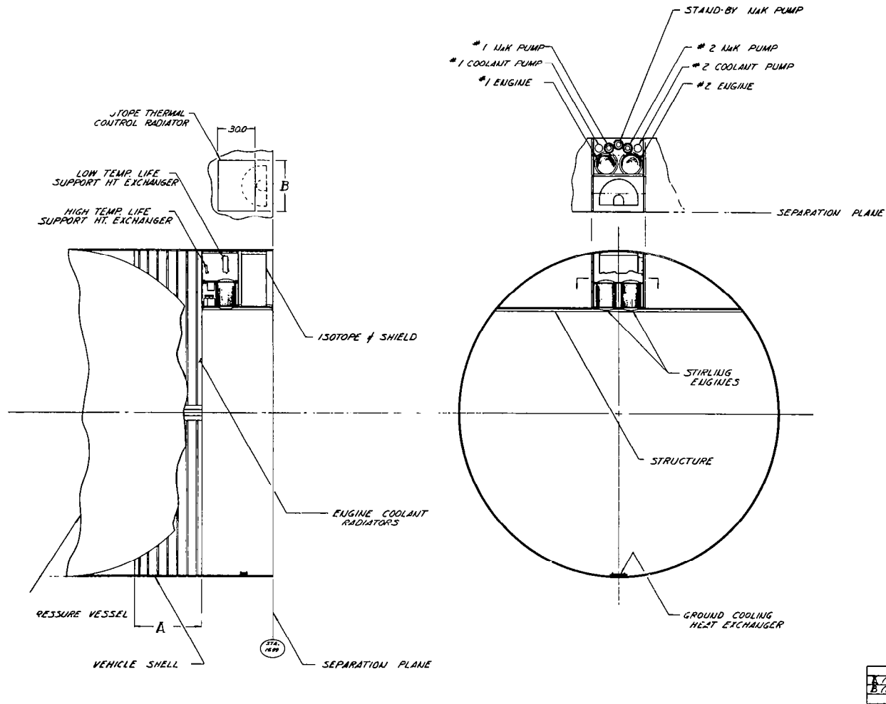
Figure 5-31. Power System Component Layout - Isotope Stirling
