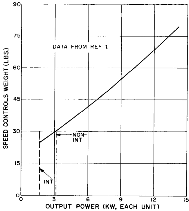
Figure 7-8. Mercury-Rankine System Speed Control Weight Vs. Power (PIC-SOL 209/4, SEC B-1, Fig. 39)
