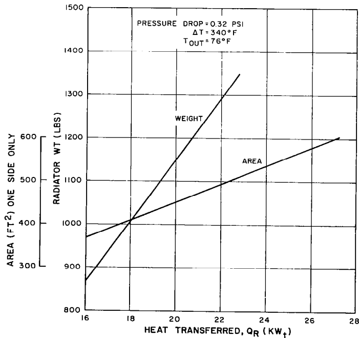
Figure 6-33. Solar Brayton Cycle Radiator Characteristics
