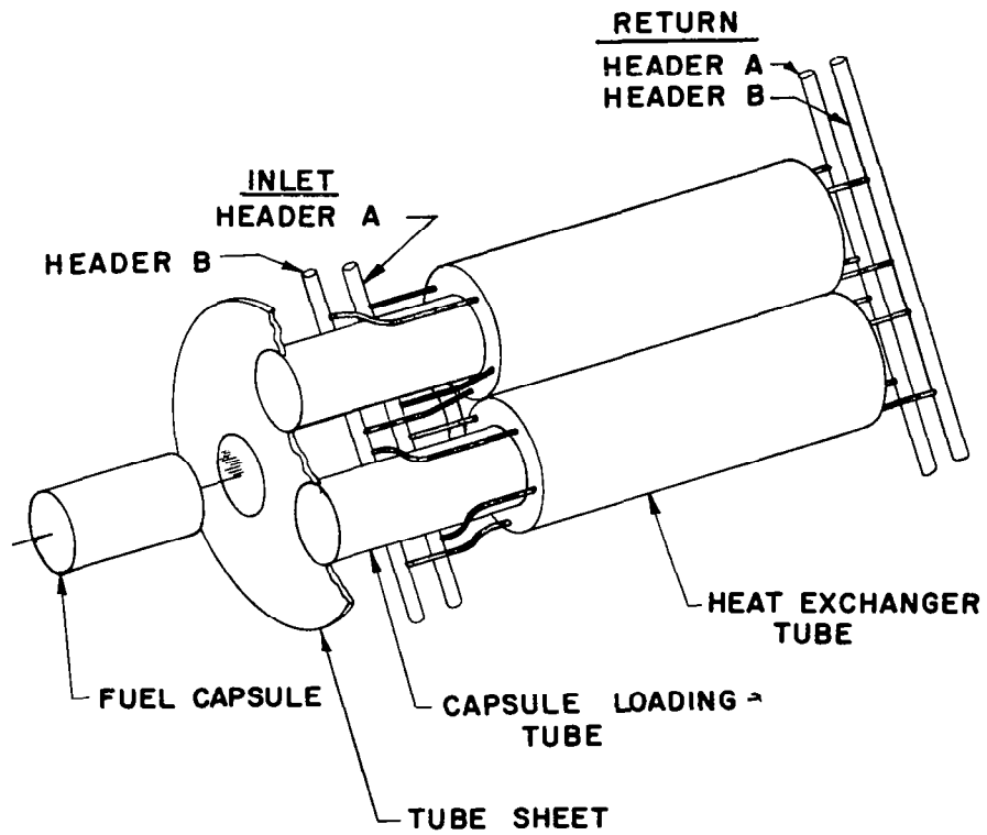
Figure 5-24. Heat Exchanger Header Arrangement
