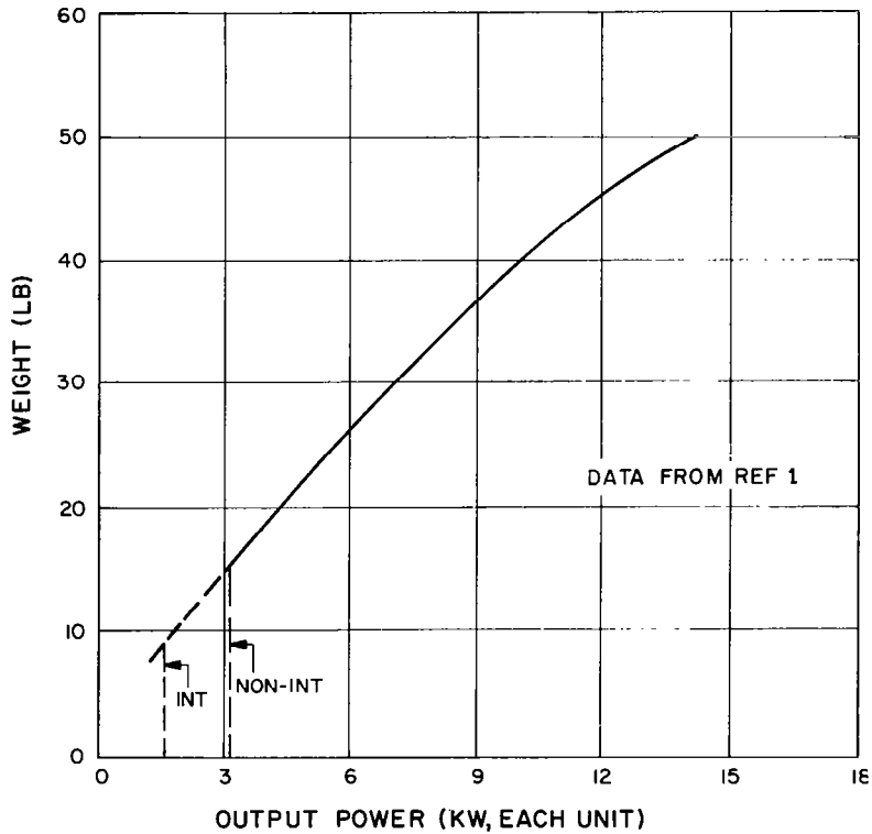
Figure 7-10. Mercury-Rankine System Mercury Inventory Weight Vs. Output Power (PIC-SOL 209/4, SEC B-1, Fig. 39)
