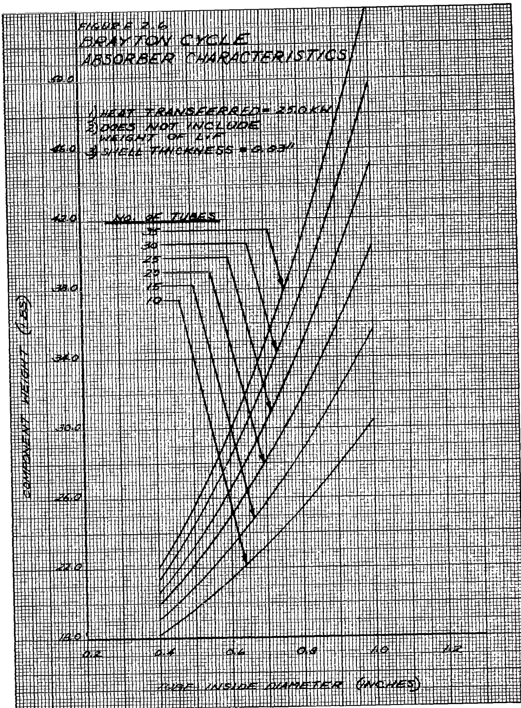
Figure C-6. Component Weight Vs. Tube ID (Heat transferred = 25.0 KW)
