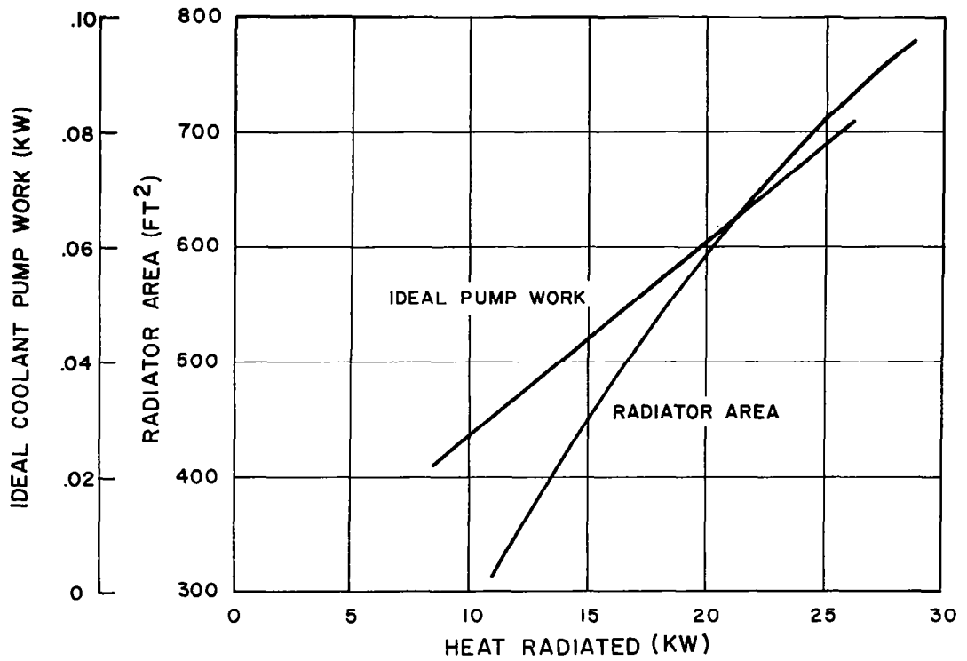
Figure 5-10. Solar Stirling Cycle Radiator Characteristics
