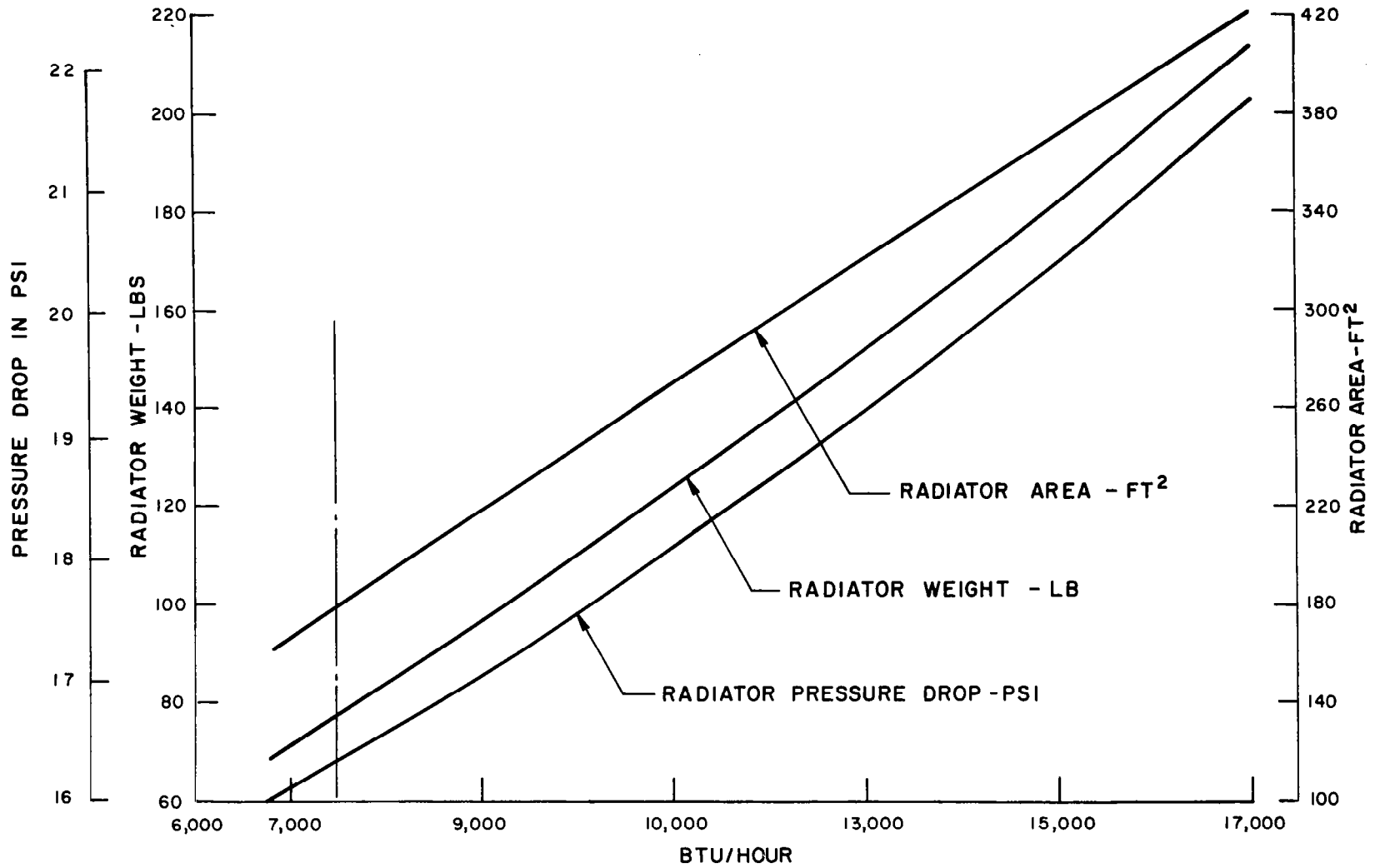
Figure 4-20. Environmental Control System Radiator Size
