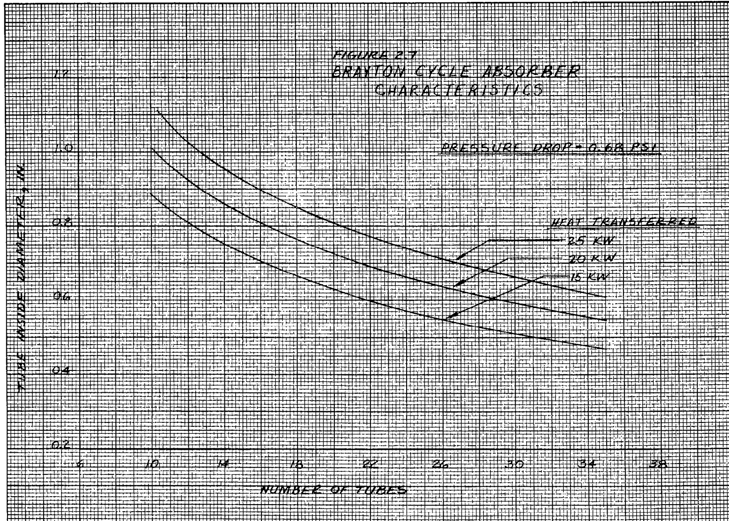
Figure C-7. Tube ID Vs. Number of Tubes
