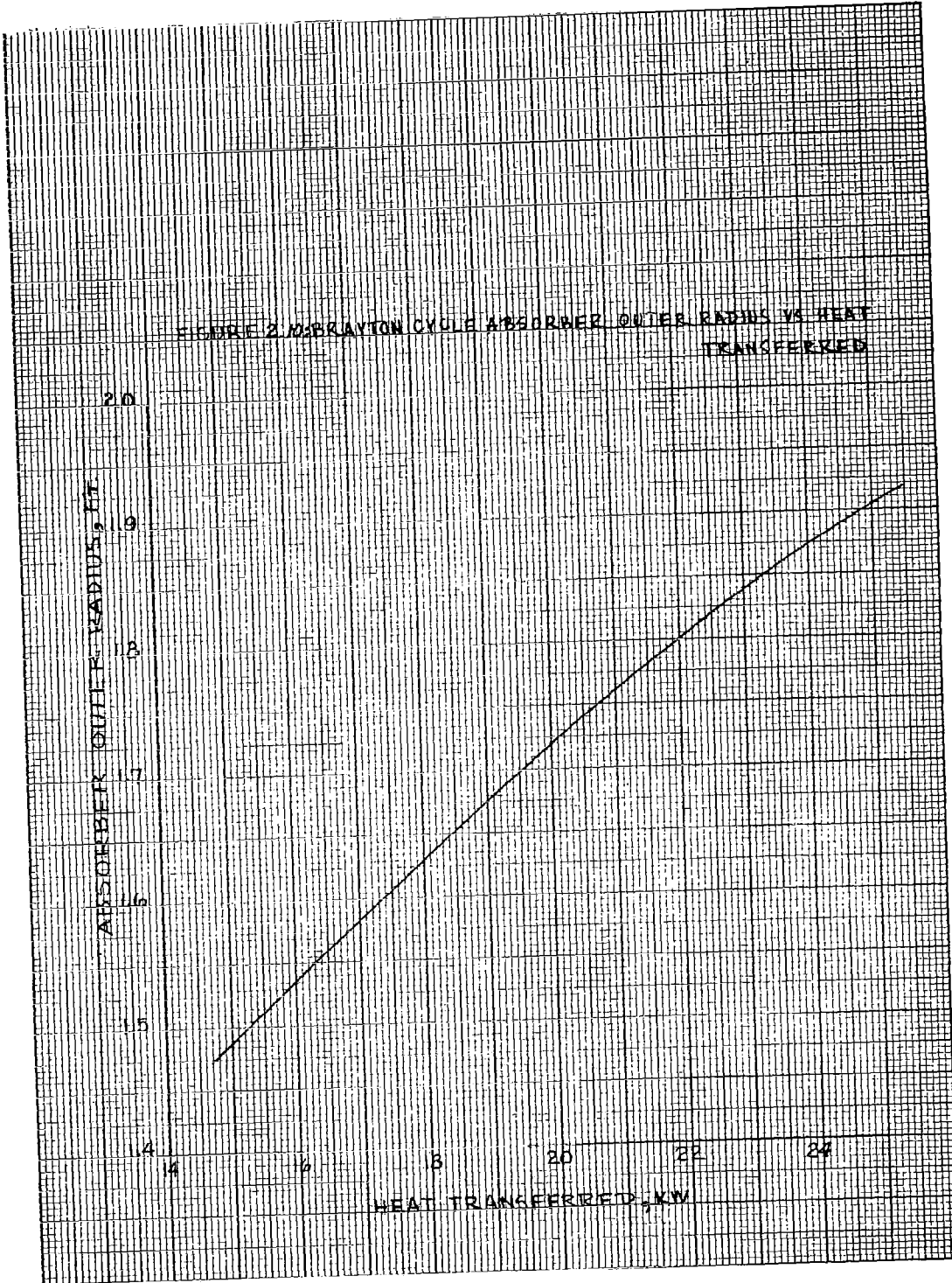
Figure C-10. Absorber Outer Radius Vs. Heat Transferred
