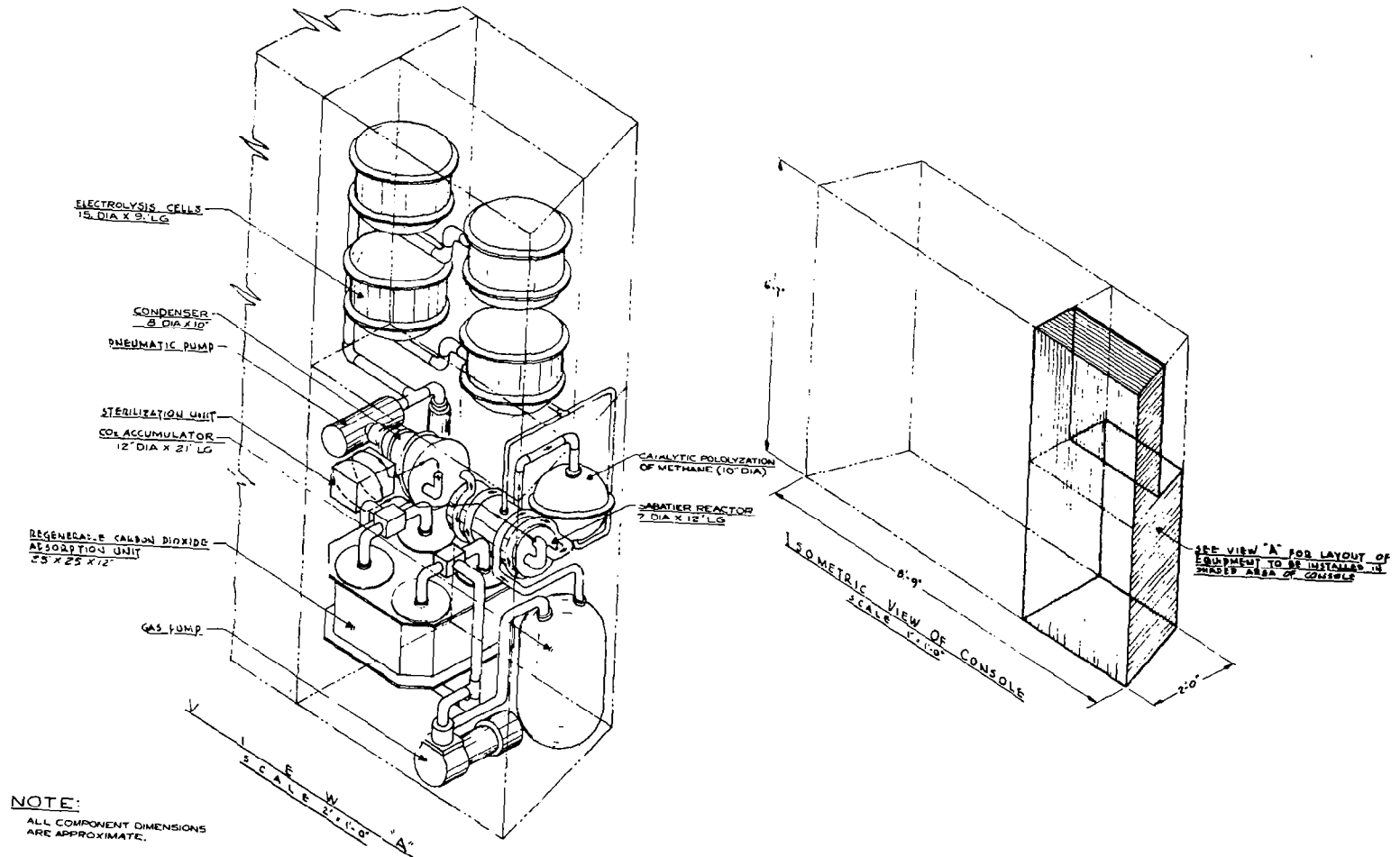
Figure 4-14. Oxygen Recovery from Carbon Dioxide - Equipment Layout
