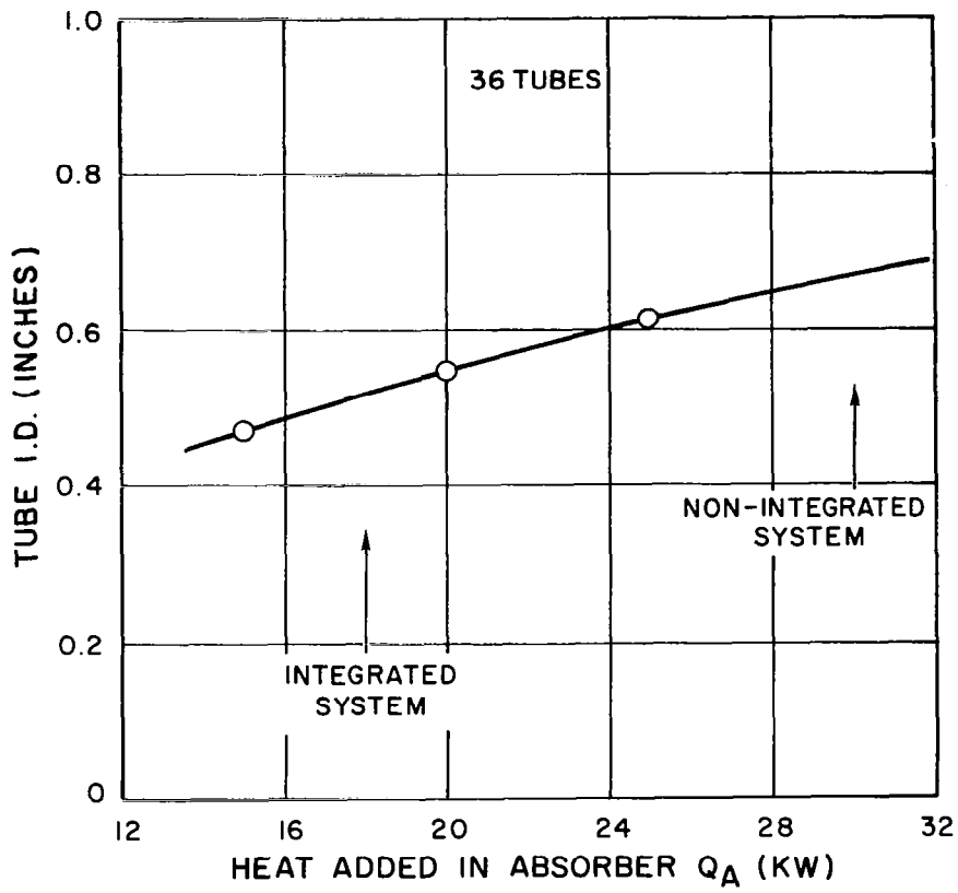
Figure 6-8. Absorber Heat Vs. Tube I. D.
