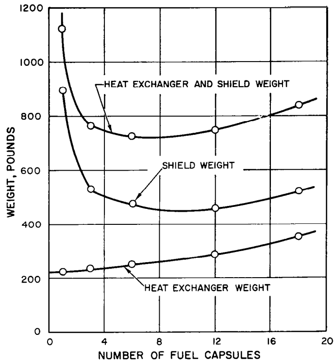
Figure 5-29. Heat Exchanger and Shield Weight
