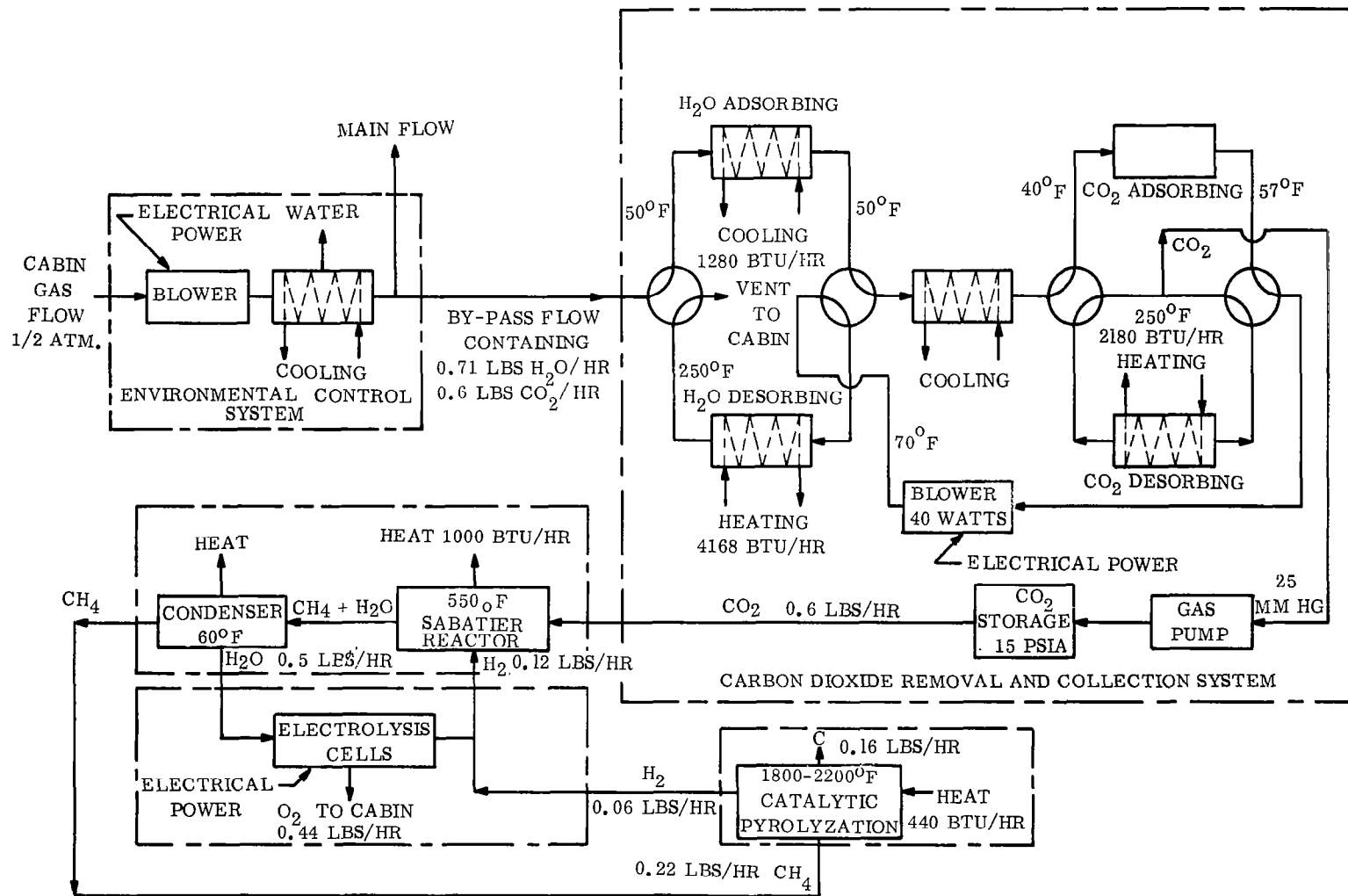
Figure 4-6. Total System for Oxygen Recovery from Carbon Dioxide (six-man system)
