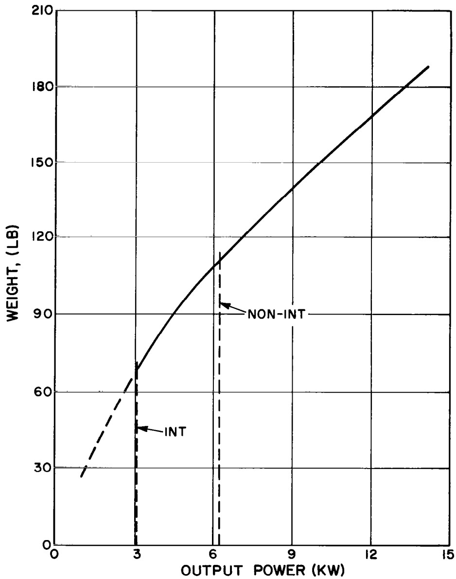
Figure 7-11. Mercury-Rankine System Structure Weight Vs. Output Power (From PIC-SOL 209/4, Figure 39)
