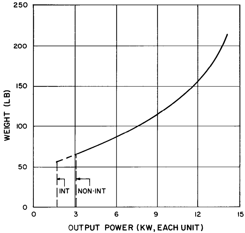
Figure 7-9. Mercury-Rankine System Start Auxiliaries Weight Vs. Output Power (PIC-SOL 209/4, SEC B-1, Fig. 39)
