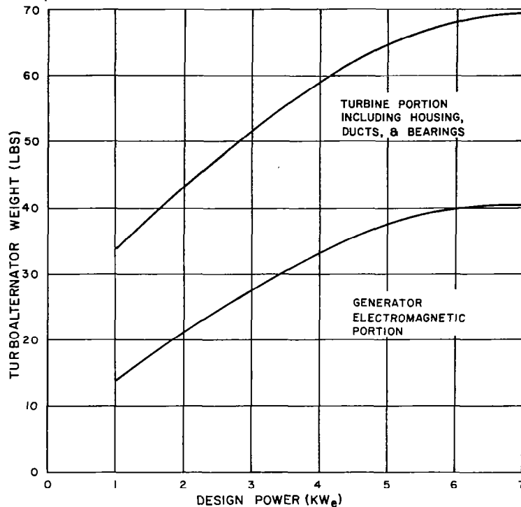
Figure 6-24. Brayton Turboalternator Weight
