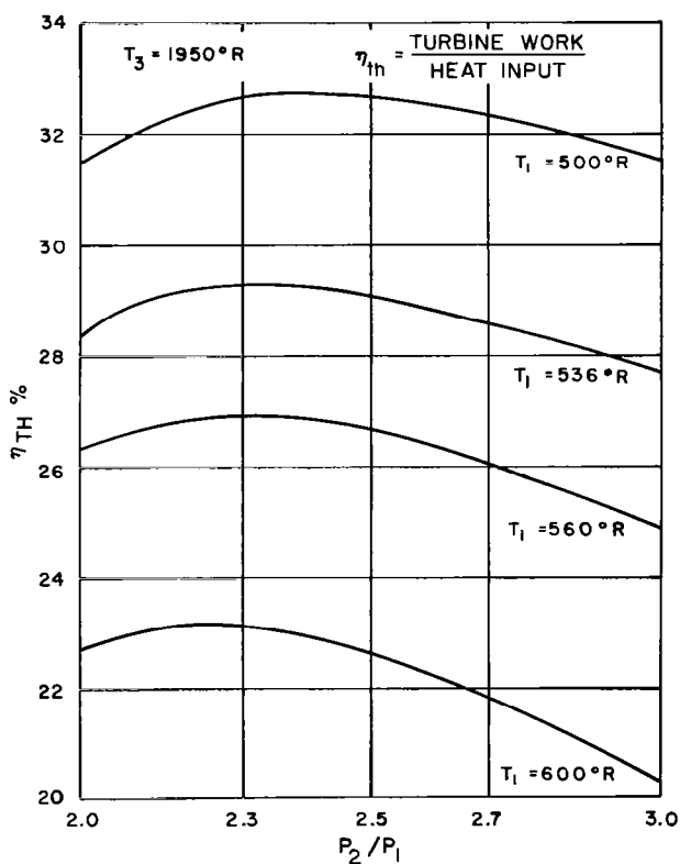
Figure 6-21. Brayton Cycle Thermodynamic Efficiency
