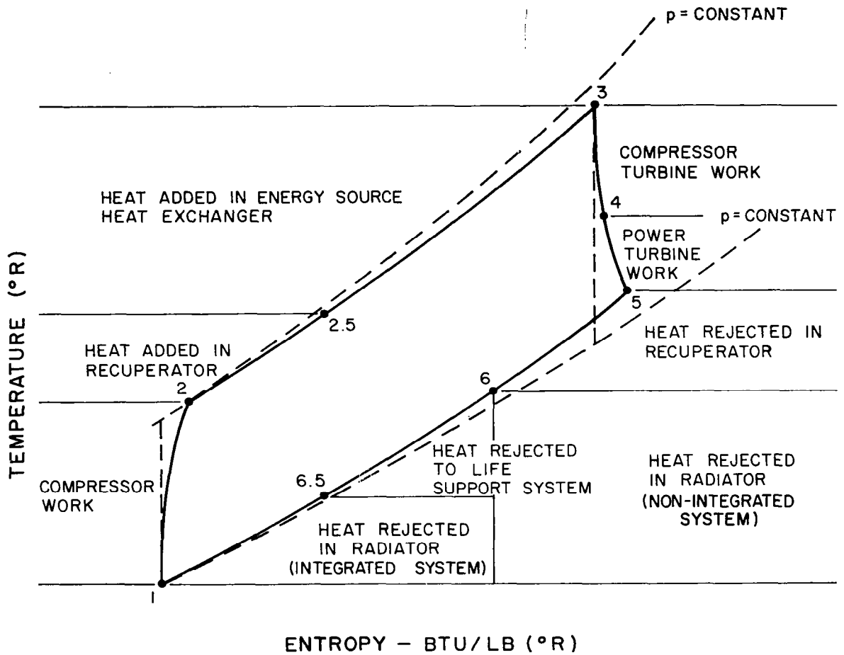
Figure 6-1. Recuperated Brayton Cycle
