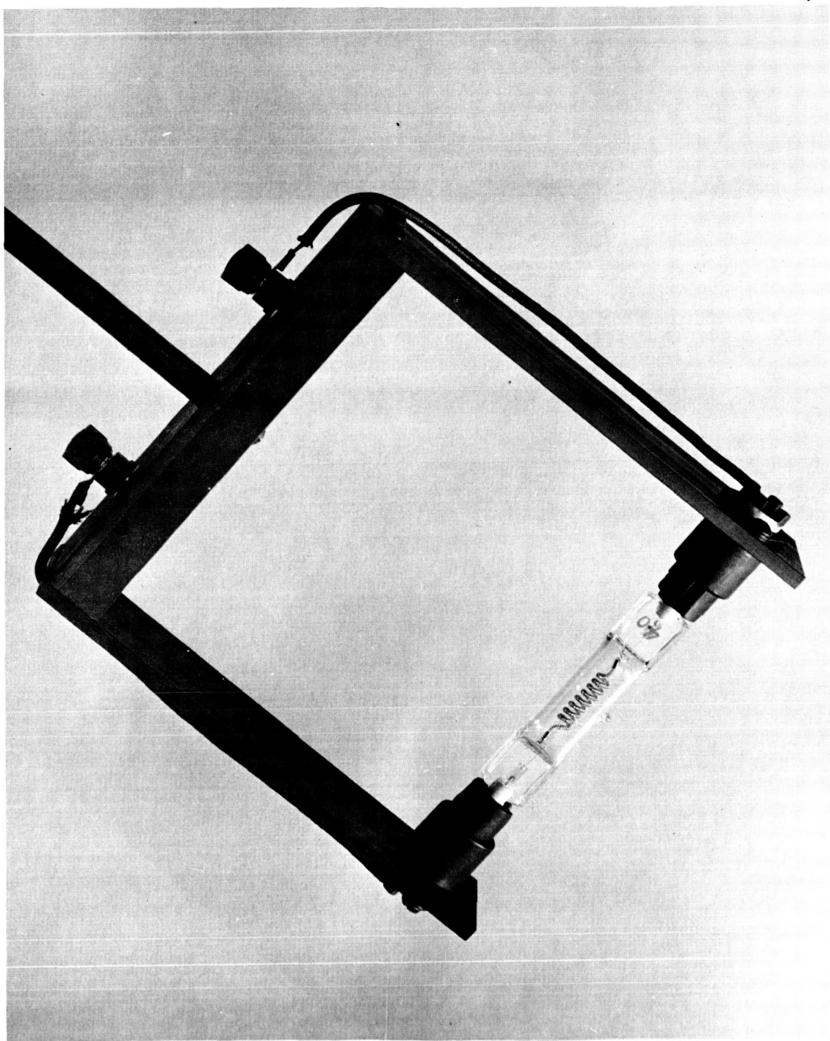
Fig. 5. The 1000-watt quartz-iodine lamp standard of spectral irradiance mounted in special holder ready for use.
