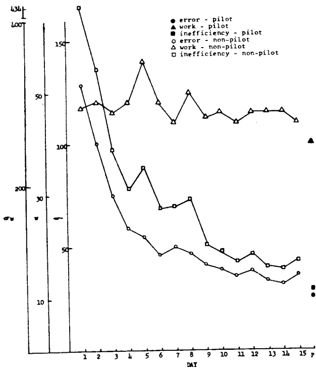
Figure 52 Error ( \sigma ) inefficiency ( \kappa w ) and work ( w ) for pitch in the presence of roll and yaw.
