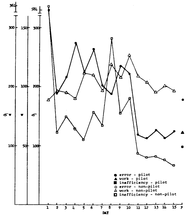
Figure 127 Error ( \sigma ) inefficiency ( \sigma_w ) and work ( w ) for altitude in the presence of pitch, roll and yaw.
