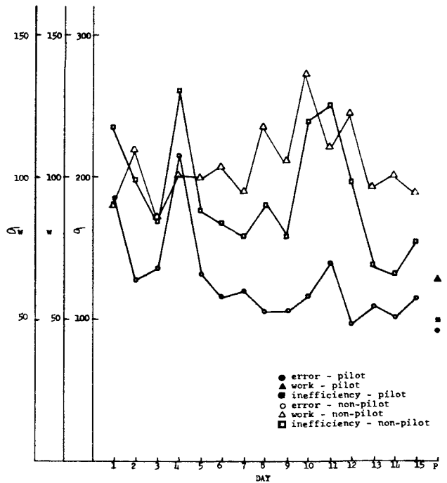
Figure 123 Error (%) inefficiency (%w) and work (w) for altitude in the presence of yaw.
