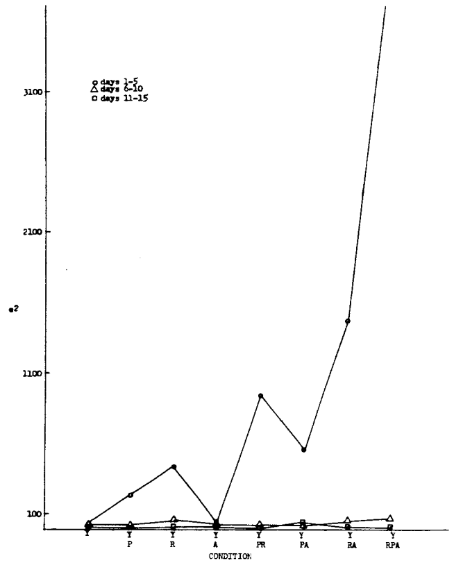
Figure 21 Squared error e^2 for the eight conditions of yaw.
