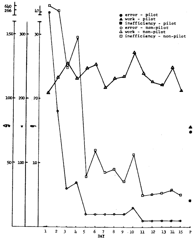
Figure 103 Error (e) and inefficiency (iw) and work (w) for yaw in the presence of pitch, roll, and altitude.
