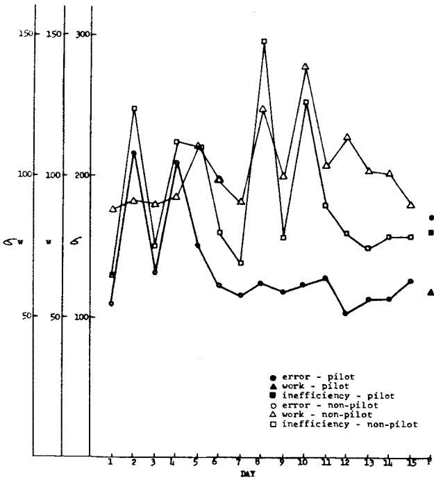
Figure 126 Error ( \sigma ) inefficiency ( \sigma_w ) and work ( w ) for altitude in the presence of roll and yaw.
