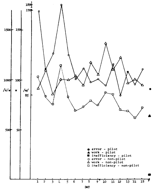
Figure 107 Error (e) and inefficiency (e/w) and work (w) for altitude in the presence of yaw.
