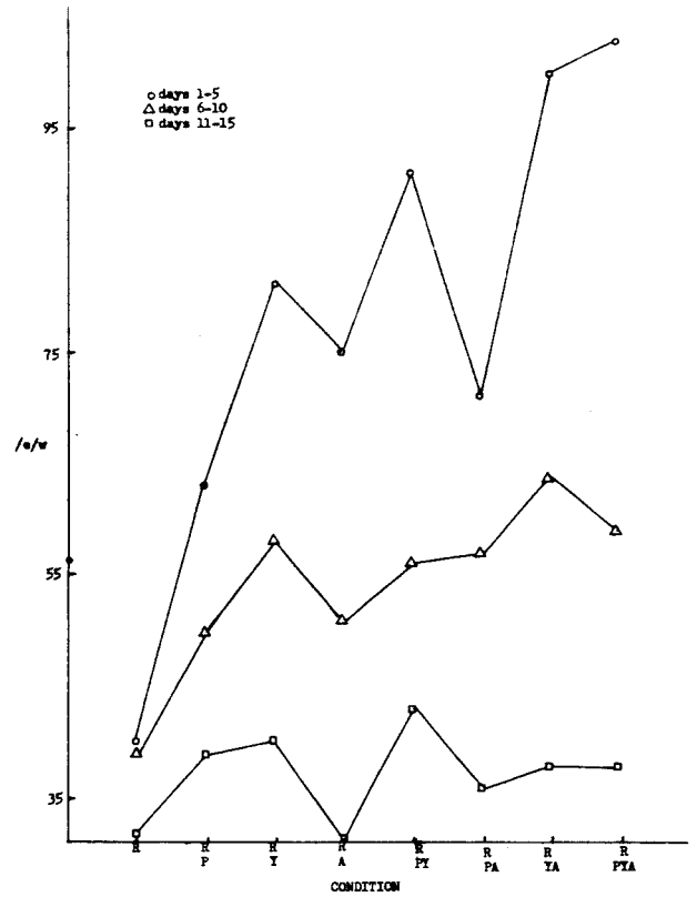
Figure 17 Inefficiency /\sigma w for the eight conditions of roll.
