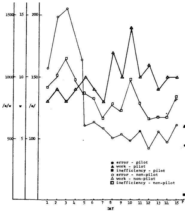
Figure 106 Error (e) and inefficiency (e/w) and work (w) for altitude in the presence of roll.
