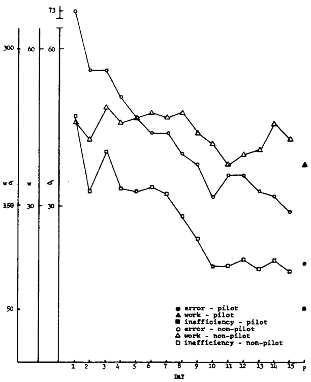
Figure 74 Error (e) inefficiency (iw) and work (w) for roll in the presence of yaw.
