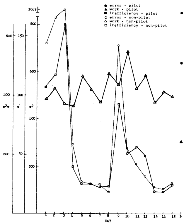
Figure 113 Error (e2) inefficiency (e2w) and work (w) for altitude in the presence of pitch.
