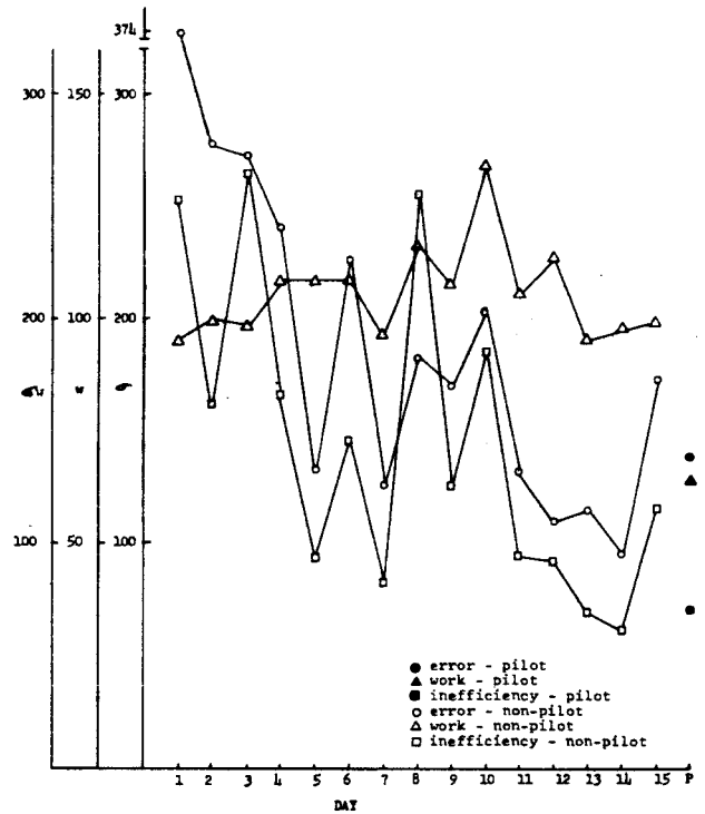
Figure 125 Error ( \sigma ) and inefficiency ( \sigma_w ) and work ( w ) for altitude in the presence of pitch and yaw.
