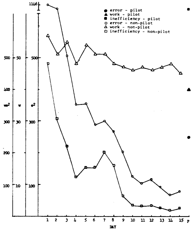
Figure 15 Error (e2) inefficiency (we2) and work (w) for pitch in the presence of roll and altitude.
