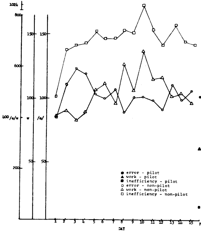
Figure 10 Error (e) and inefficiency (e/w) and work (w) for altitude alone.
