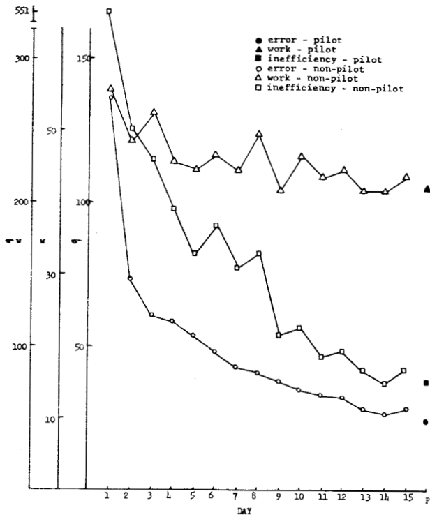
Figure 50 Error ( \epsilon ) inefficiency ( \epsilon w ) and work ( w ) for pitch in the presence of yaw.
