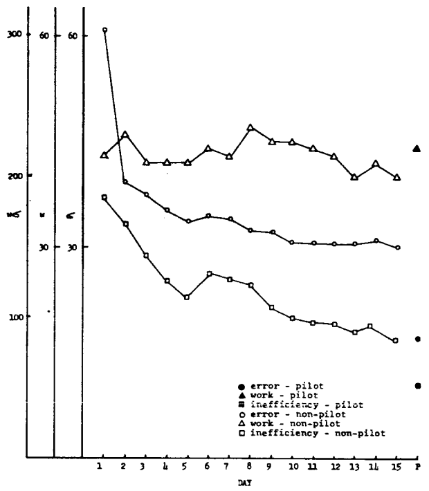
Figure 73 Error (e) inefficiency (iw) and work (w) for roll in the presence of pitch.
