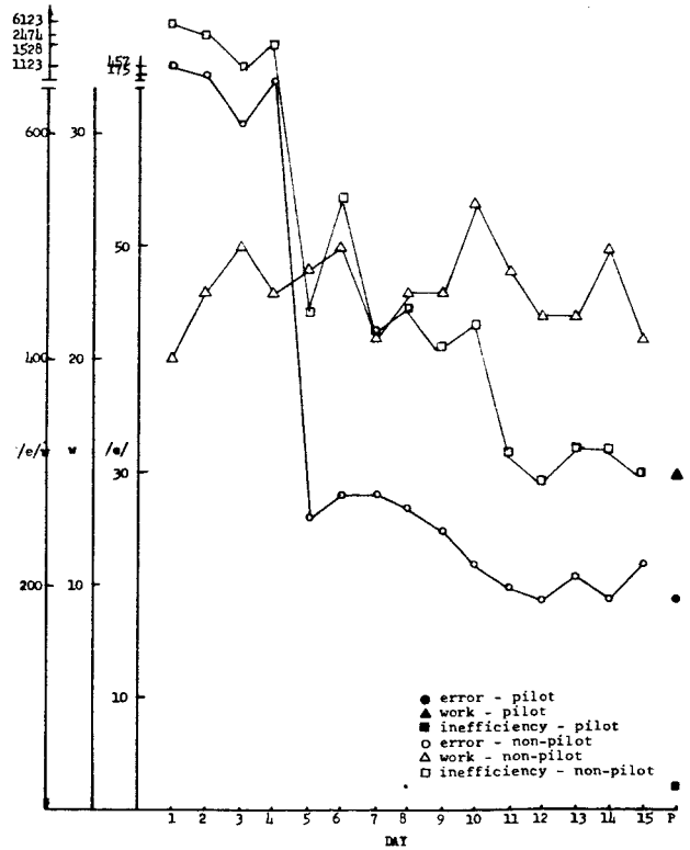
Figure 87 Error (/e/) and inefficiency (/e/w) and work (w) for yaw in the presence of pitch, roll, and altitude.
