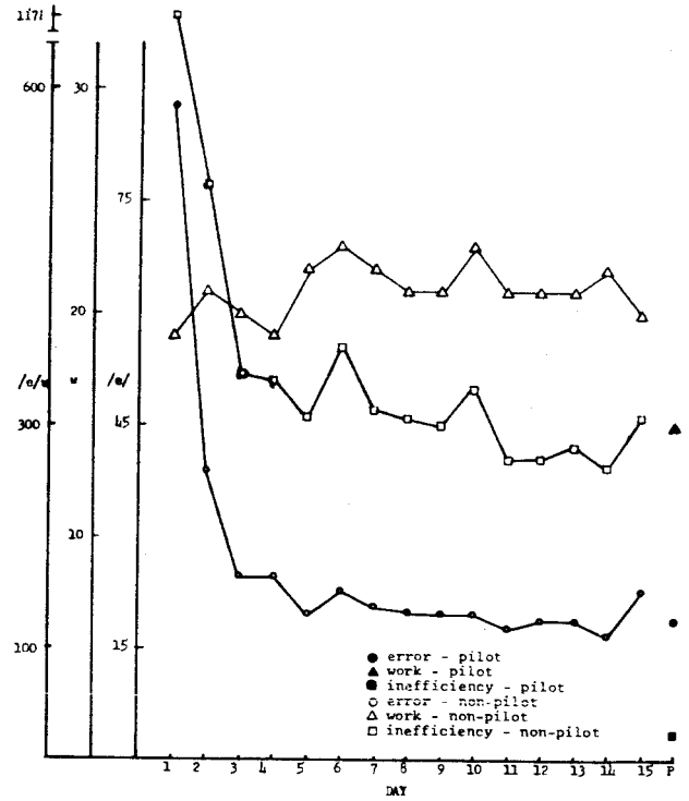
Figure 51 Error (/e/) and inefficiency (/e/w) and work (w) for yaw in the presence of pitch.
