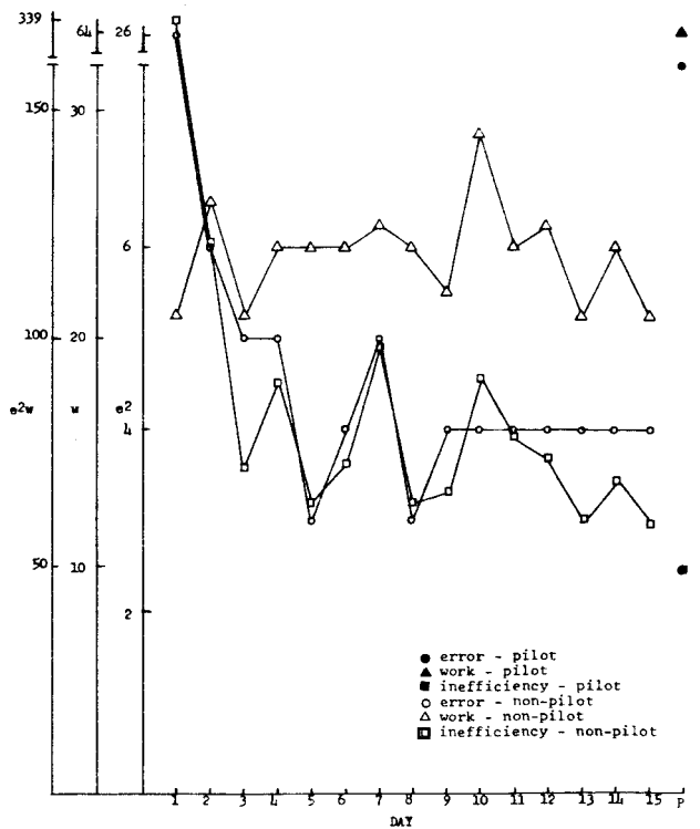
Figure 91 Error (e2) inefficiency (e2w) and work (w) for yaw in the presence of altitude.
