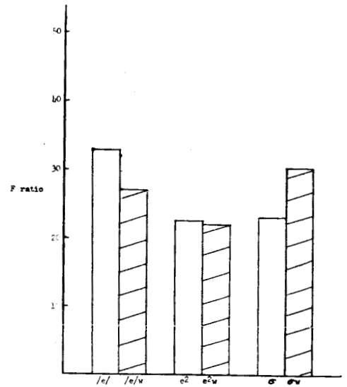
Figure 149 F ratios obtained between days for yaw (non-pilot data).
