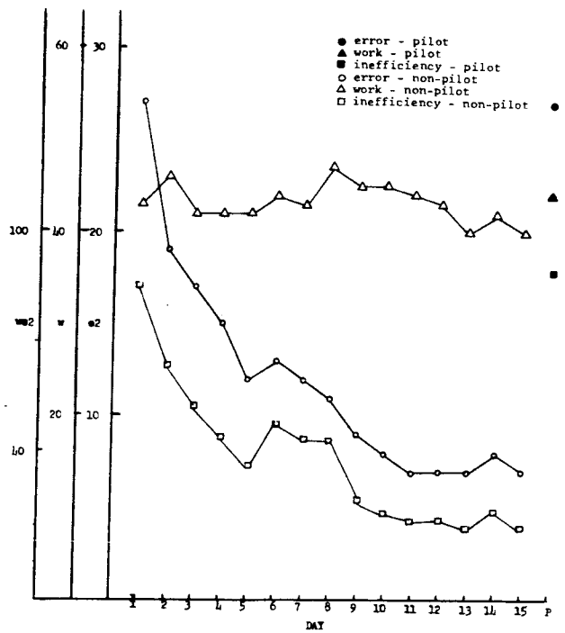
Figure 65. Error (e2) inefficiency (we2) and work (w) for roll in the presence of pitch.
