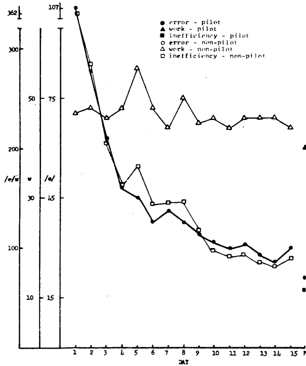
Figure 36 Error (/e/) and inefficiency (/e/w) and work (w) for pitch in the presence of yaw and roll.
