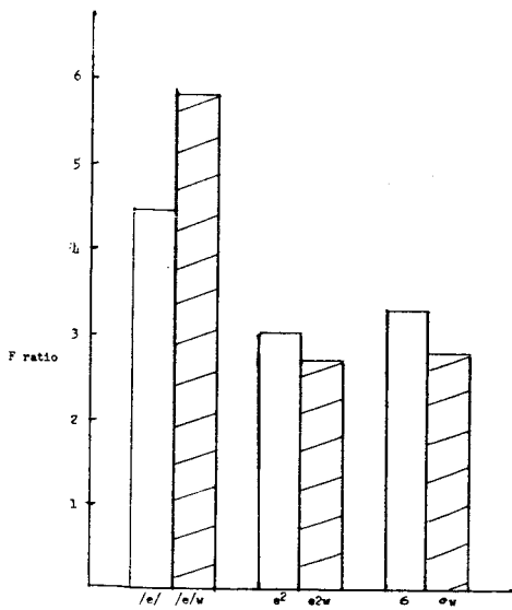
Figure 158 F ratios obtained for conditions x subjects interaction for altitude (non-pilot data)
