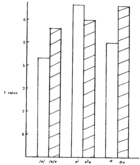
Figure 157 F ratios obtained for conditions x days interaction for altitude (non-pilot) data.
