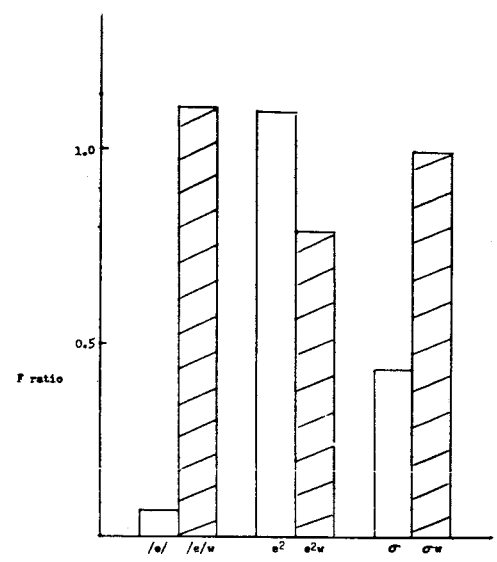
Figure 115 F ratios obtained for conditions x days interaction for roll (non-pilot data).
