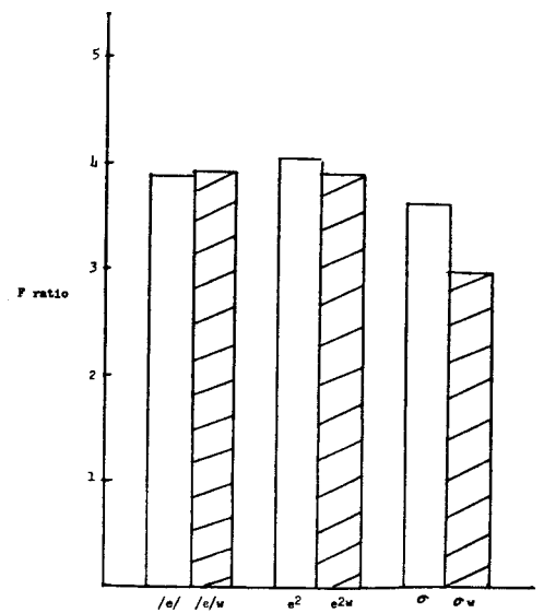
Figure 135 F ratios obtained between subjects for altitude (pilot data).
