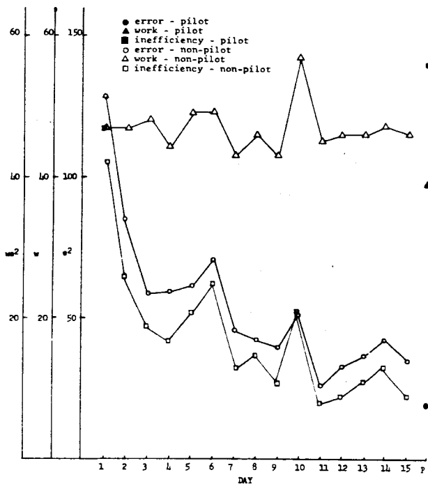
Figure 40 Error (e2) inefficiency (e2w) and work (w) for pitch alone.
