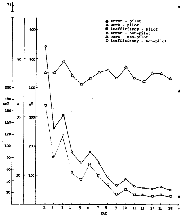
Figure 41 Error (e2) inefficiency (e2w) and work (w) for pitch in the presence of roll.
