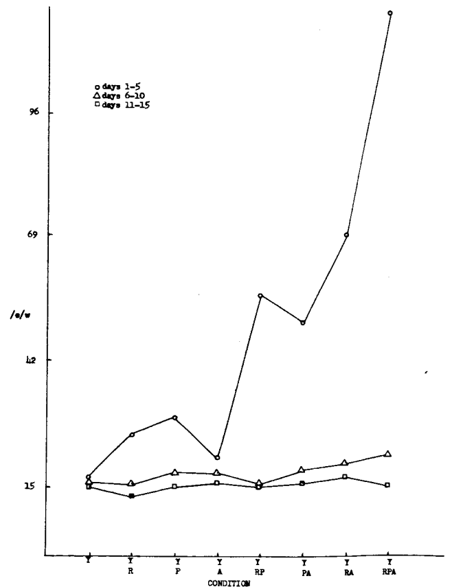
Figure 23 Inefficiency /e/w for the eight conditions of yaw.
