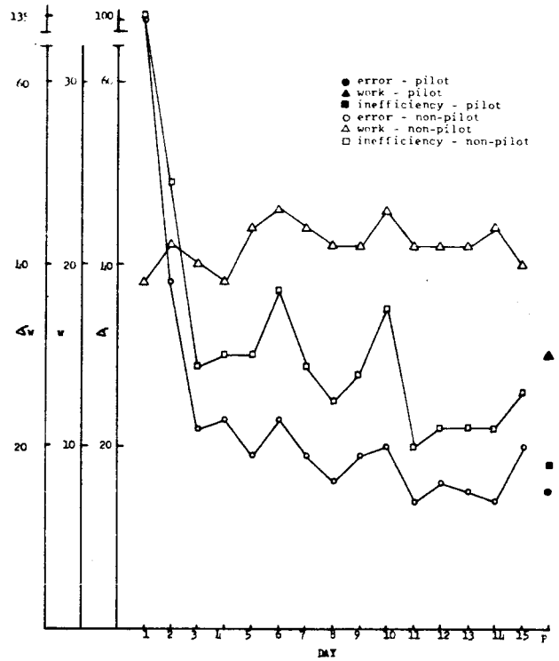
Figure 97 Error ( \sigma ) inefficiency ( \sigma_w ) and work ( w ) for yaw in the presence of pitch.
