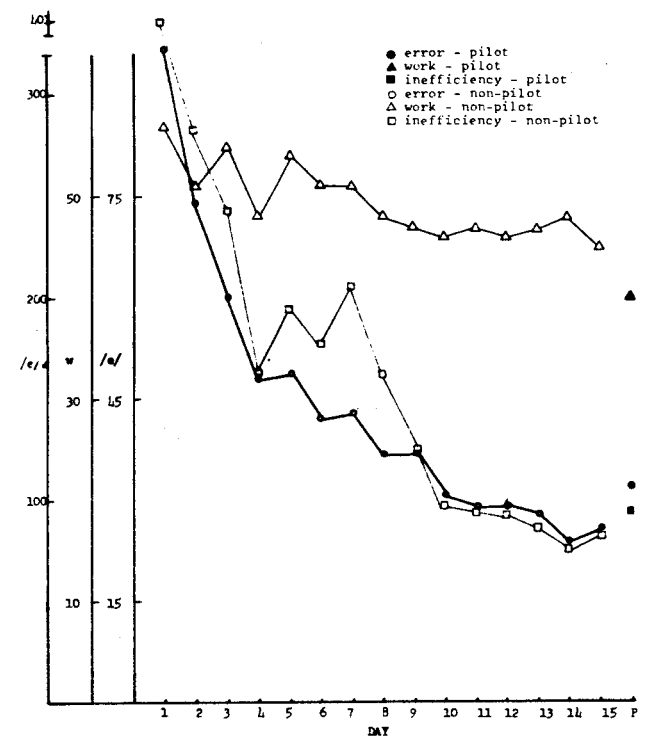
Figure 37 Error (/e/) and inefficiency (/e/w) and work (w) for pitch in the presence of roll and altitude.
