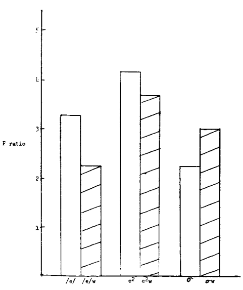
Figure 116 F ratios obtained for conditions x subjects interaction for roll (non-pilot data).
