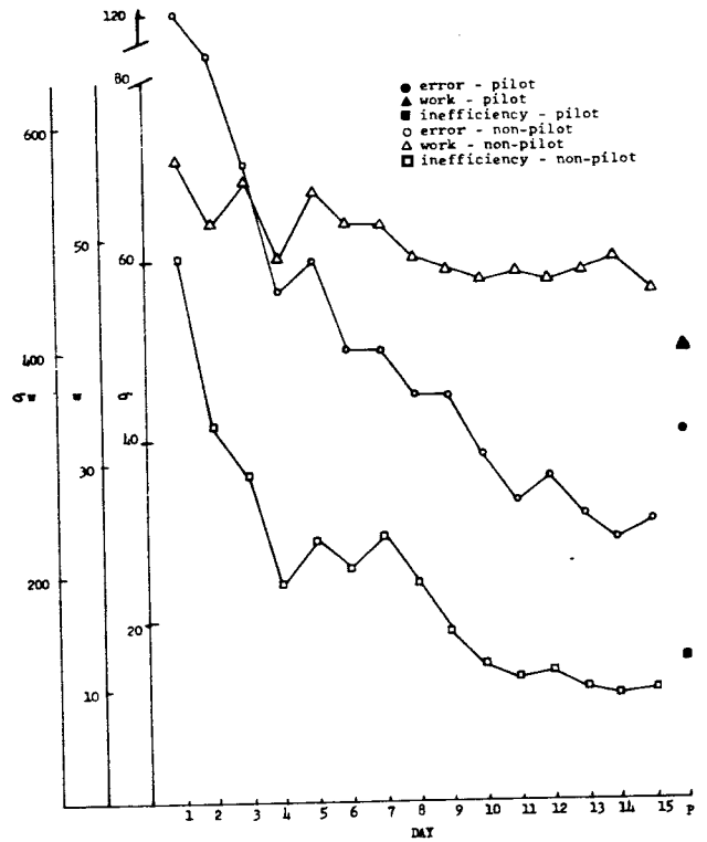
Figure 53 Error ( \sigma ) inefficiency ( \kappa w ) and work ( w ) for pitch in the presence of roll and altitude.
