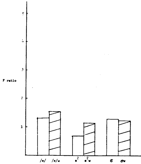
Figure 132 F ratios obtained between conditions for law (pilot data).
