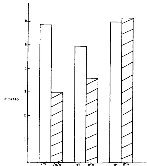
Figure 139 F ratios obtained for conditions x days interaction for pitch (non-pilot data).
