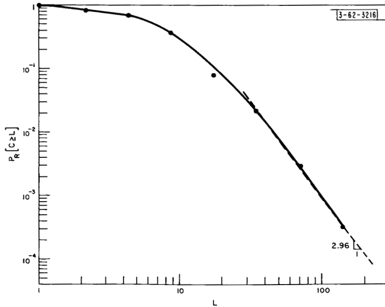
Fig. 21. Empirical distribution of computation.
