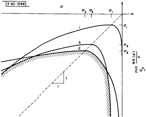
Fig. 13. Minimization of N\epsilon(\sigma)/(F) over \underline{Q}_0 .
